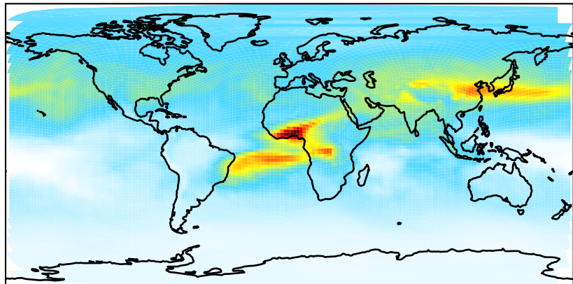
GCHP_13.0.0-beta.1 (Ref) c48
