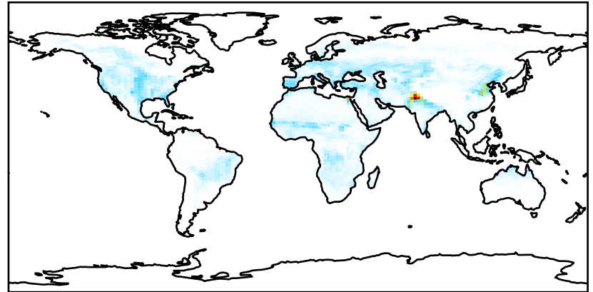
GCHP_12.4.0 (Dev) c48
