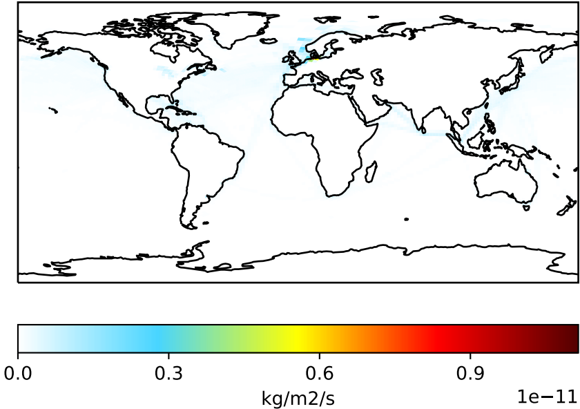
GCHP_12.5.0 (Dev) c48
