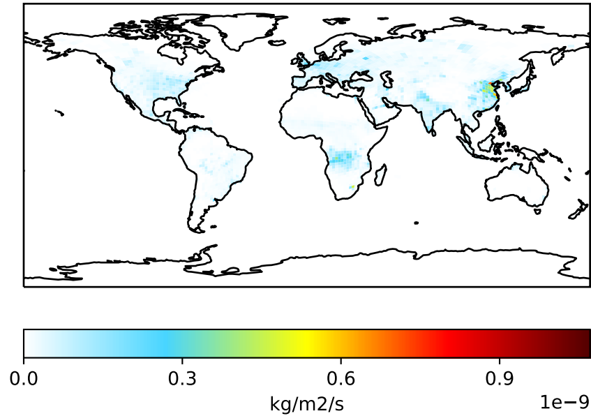
GCHP_12.4.0 (Ref) c48
