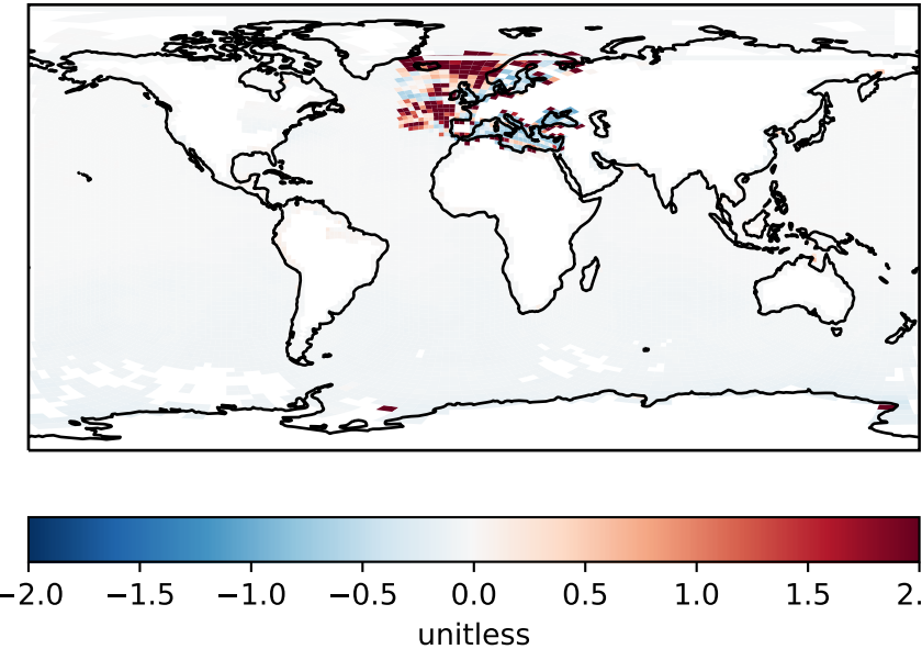
Fractional Difference (Dev-Ref)/Ref, Fixed Range
