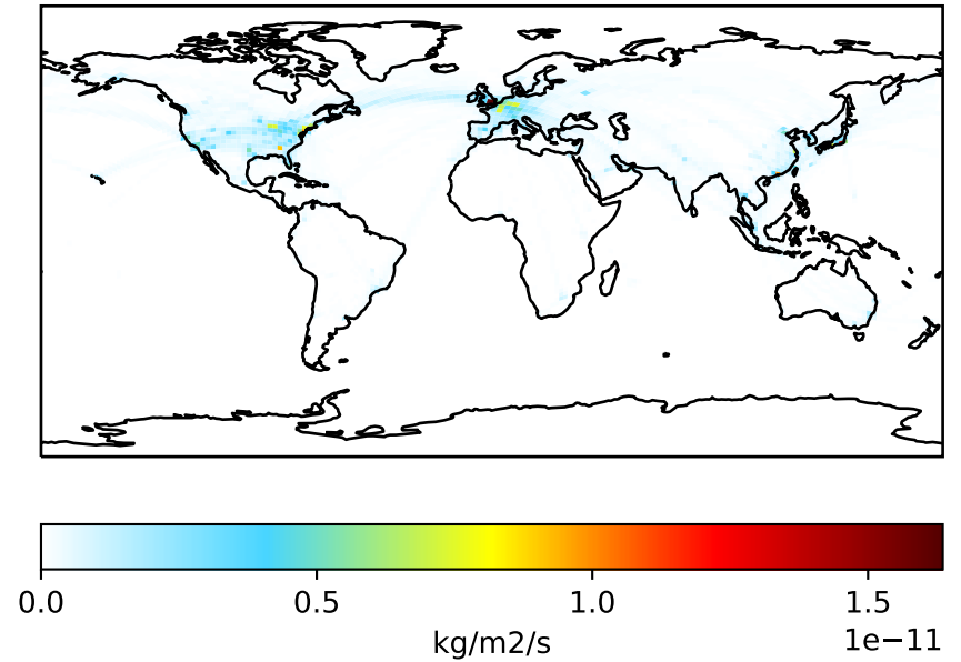
GCHP_12.5.0 (Dev) c48
