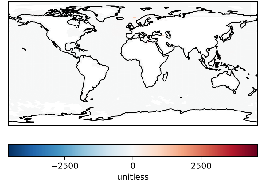
Fractional Difference (Dev-Ref)/Ref, Dynamic Range
