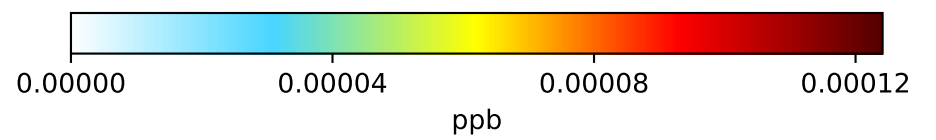
Difference (1x1.25) Dev - Ref, Restricted Range [5%,95%]
