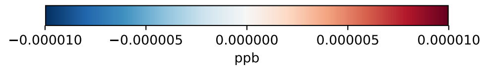
Fractional Difference (1x1.25) (Dev-Ref)/Ref, Fixed Range
