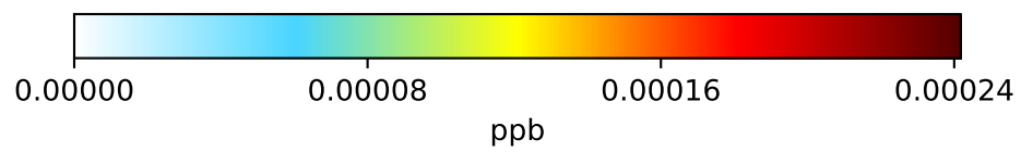
Difference (1x1.25) Dev - Ref, Dynamic Range
