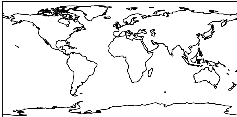
GCHP_12.4.0 (Ref) c48
