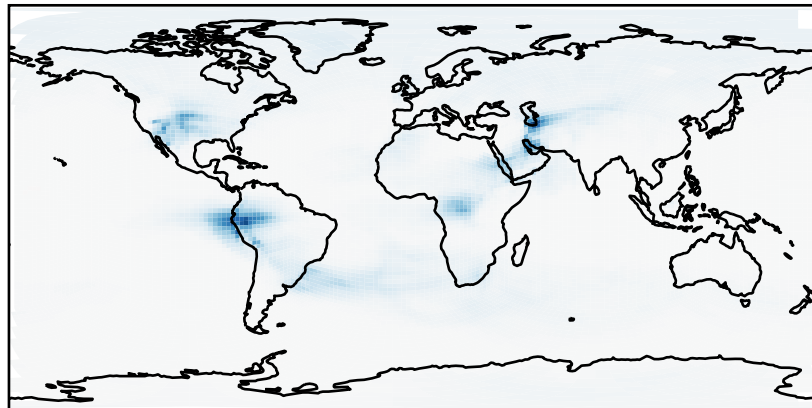
GCHP_12.6.0 - GCHP_12.5.0 (Dev) c48
