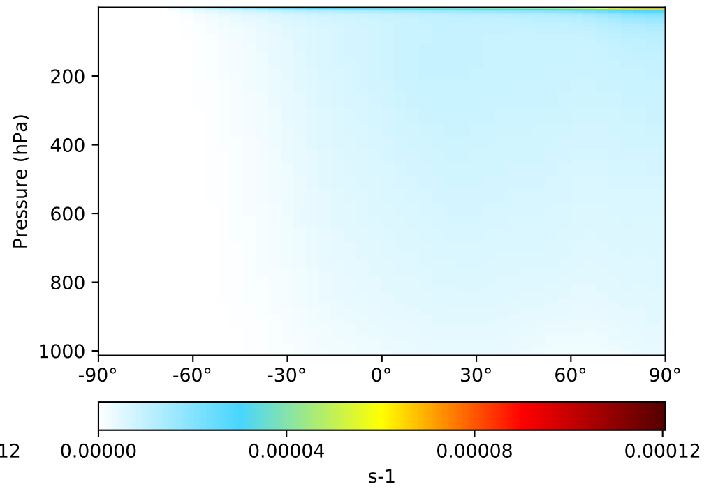
Difference Dev - Ref, Restrictd Range [5%,95%]
