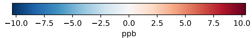
Difference (1x1.25), Dynamic Range \text{GCHP\_dev} / \text{GCHP\_ref} - \text{GCC\_dev} / \text{GCC\_ref}
