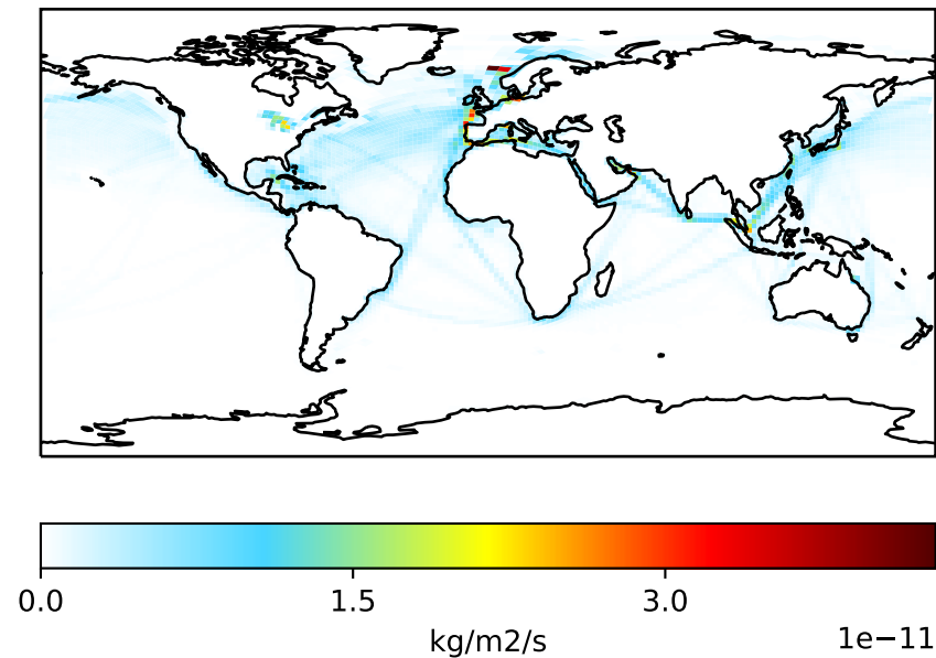
GCHP_13.3.0-rc.1 (Dev) c48
