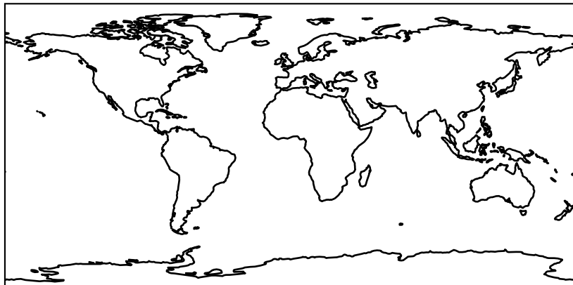
GCHP_13.4.0-rc.1 (Dev) c48
