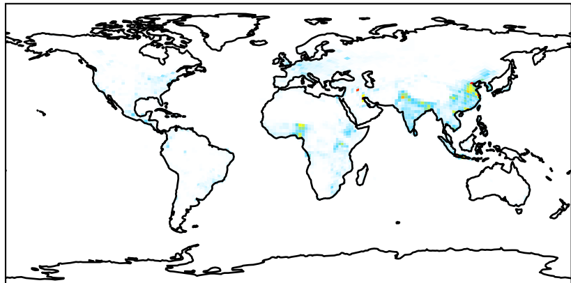
GCHP_13.3.0-rc.1 (Ref) c48
