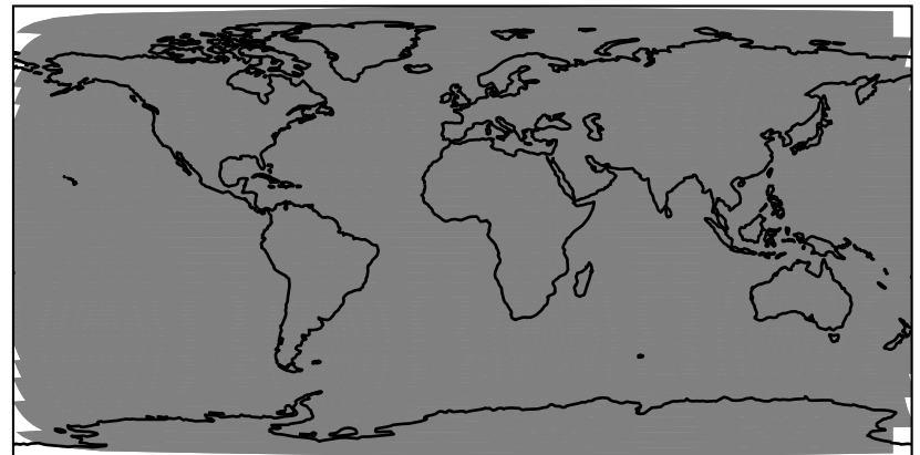
GCHP_13.4.0-rc.2 - GCHP_13.3.0-rc.1 (Dev) c48
