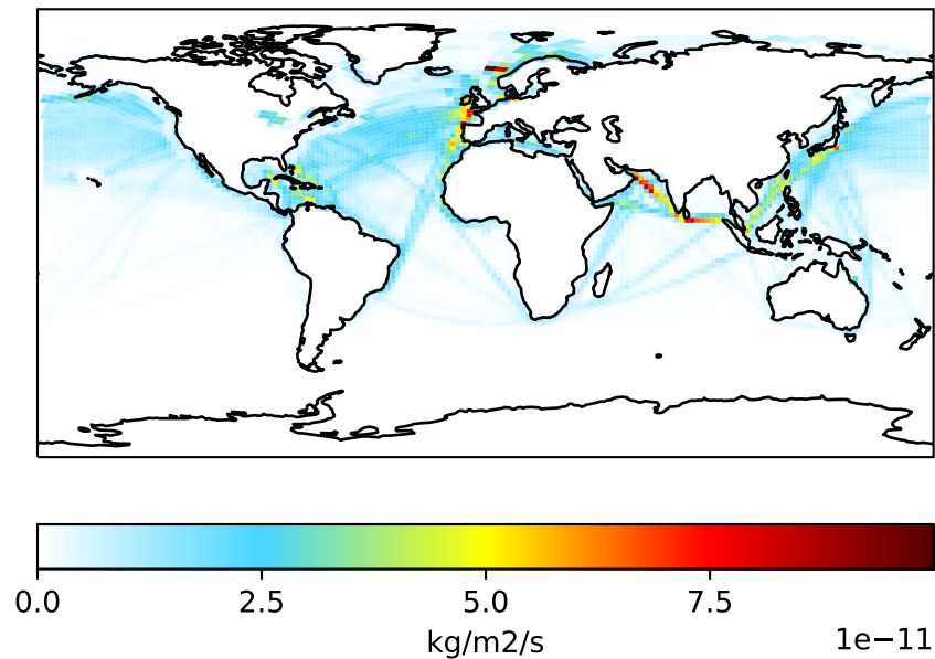
GCHP_13.3.0-rc.1 (Ref) c48
