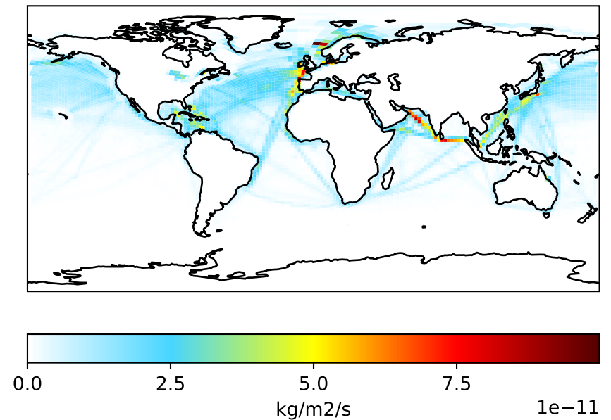
GCHP_13.4.0-rc.2 (Dev) c48
