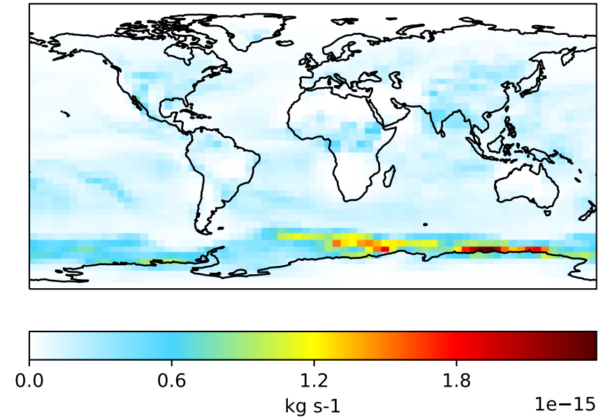
GCC_13.2.0-TransportTracers (Dev) 4.0x5.0
