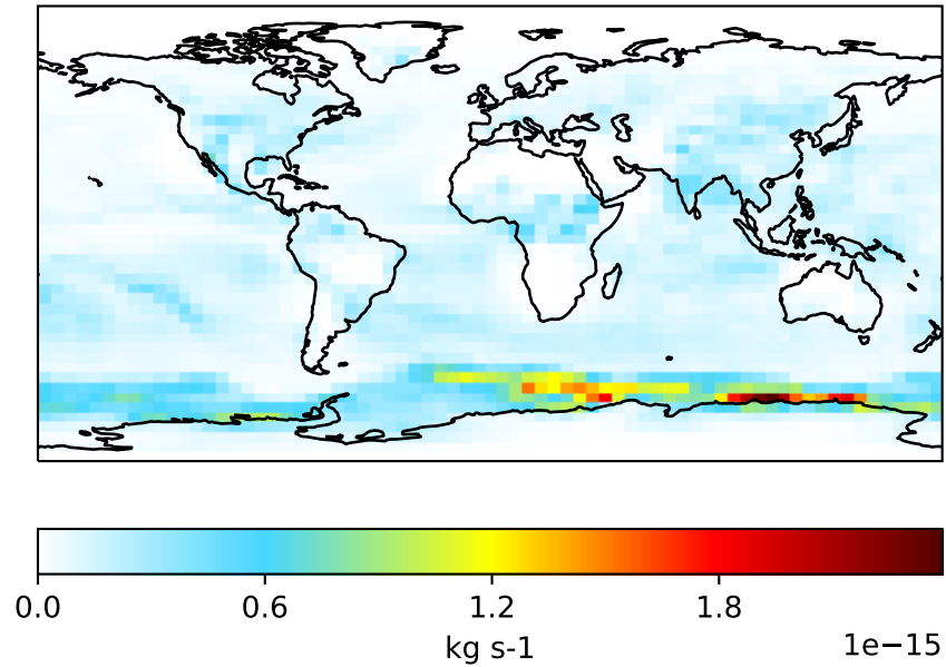
GCC_13.0.0-TransportTracers (Ref) 4.0x5.0
