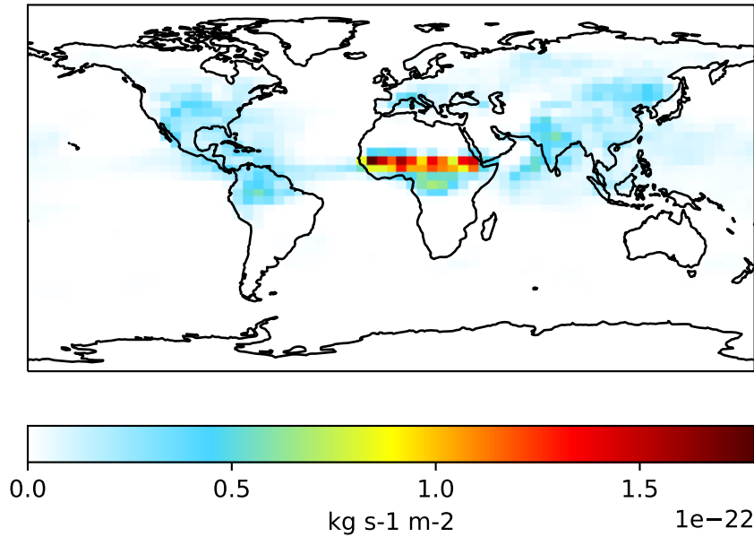
GCC_13.2.0-TransportTracers (Ref), Normalized by Area 4.0x5.0
