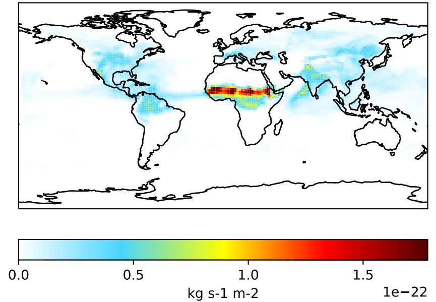
GCHP_13.2.0-TransportTracers (Dev), Normalized by Area c48
