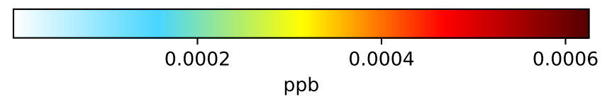
Difference (1x1.25) Dev - Ref, Restricted Range [5%,95%]
