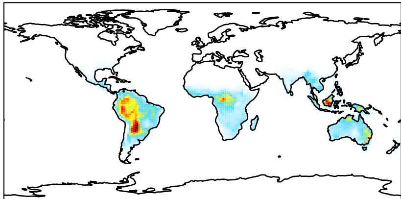
GCHP_13.2.0 (Ref) c48
