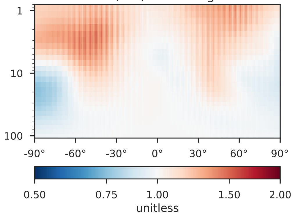
Ratio (1x1.25) Dev/Ref, Fixed Range
