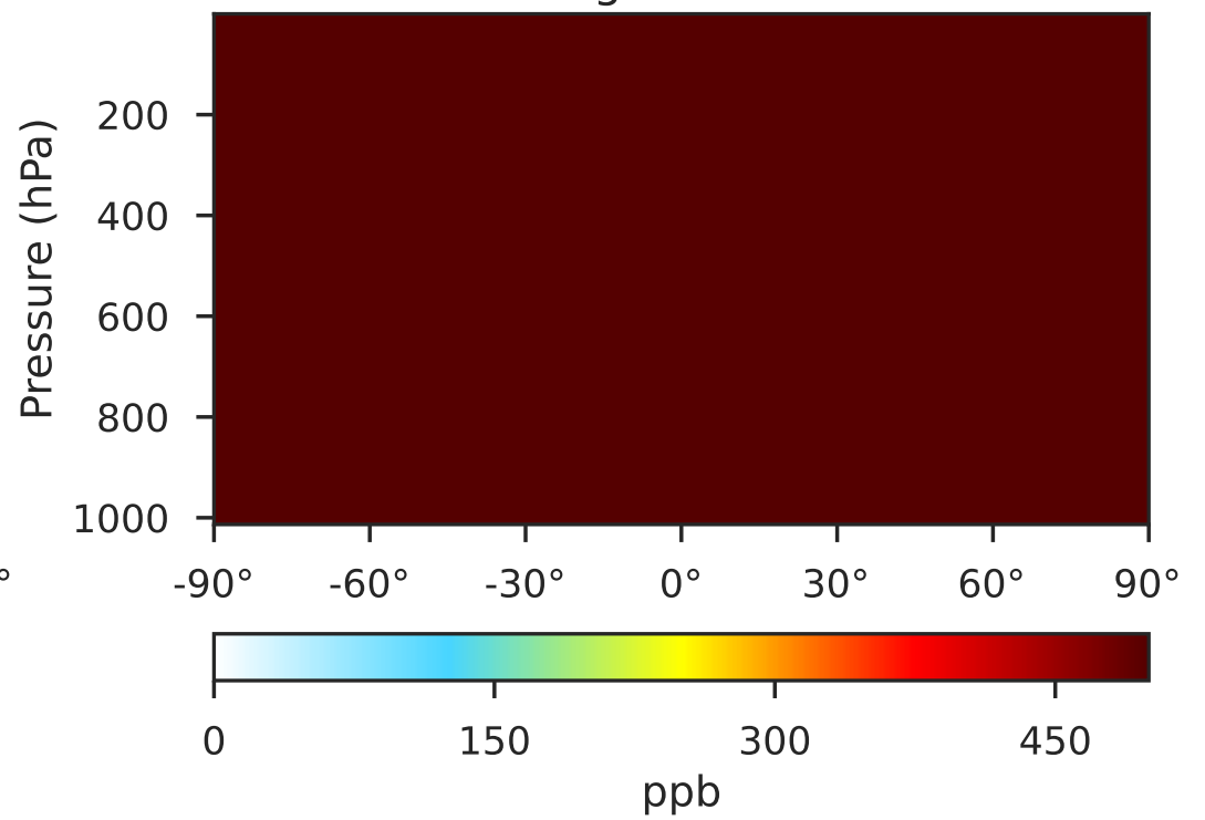
GCHP_14.2.0 (Dev) 1x1.25 regridged from c24
