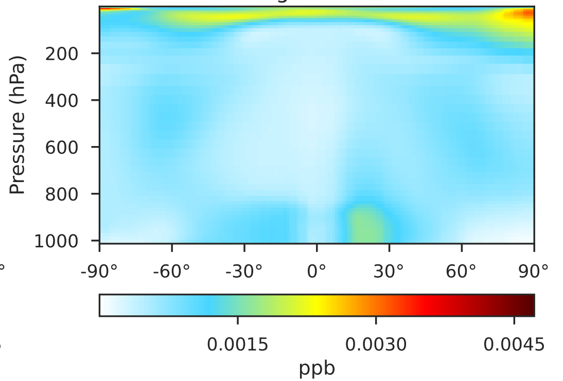
GCHP_14.2.0 (Dev) 1x1.25 regridded from c24
