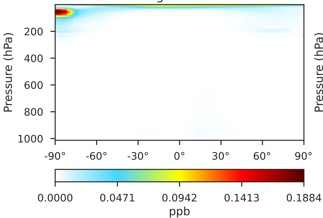
GCHP_14.0.0 (Ref) 1x1.25 regridded from c24
