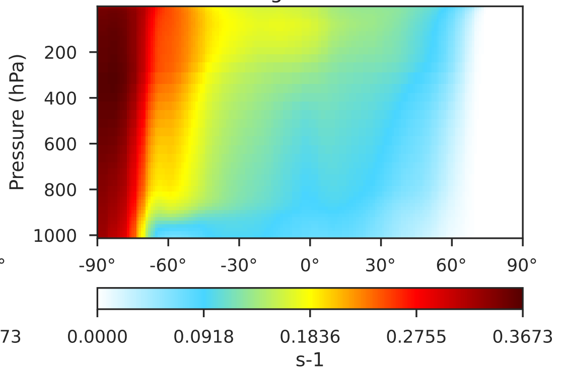
GCHP_14.2.0 (Dev) 1x1.25 regridded from c24
