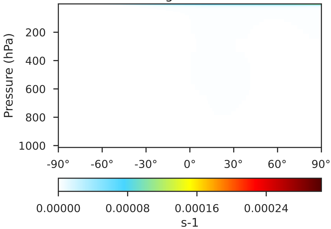
GCHP_14.0.0 (Ref) 1x1.25 regridted from c24
