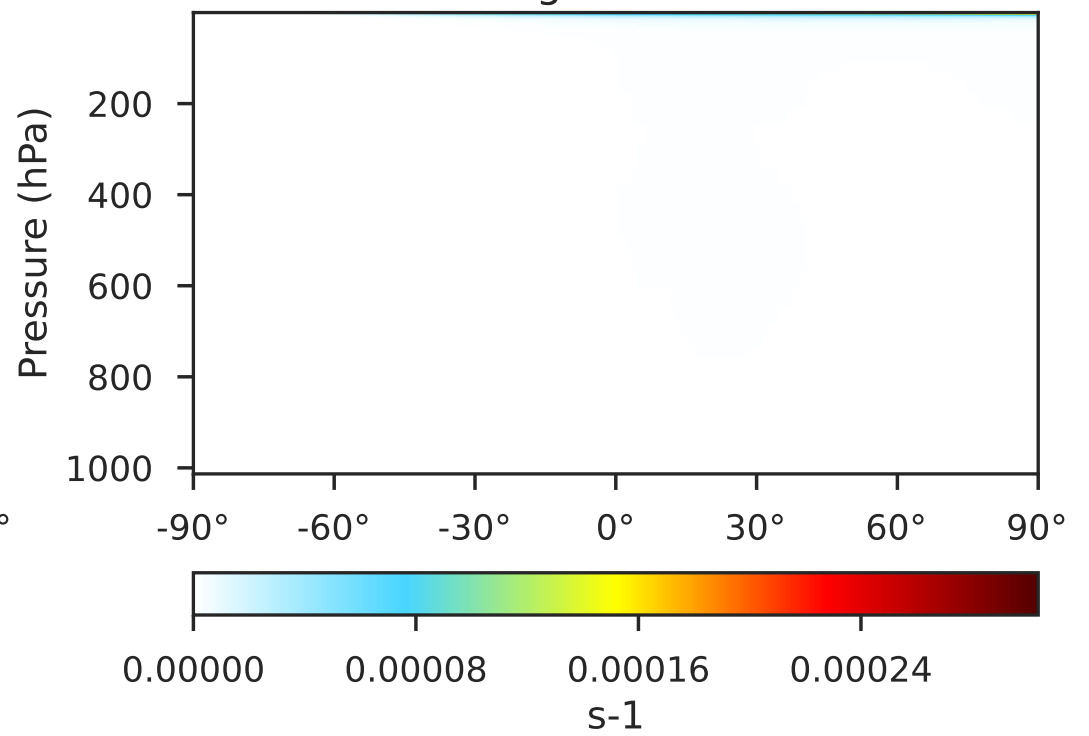
GCHP_14.2.0 (Dev) 1x1.25 regridted from c24
