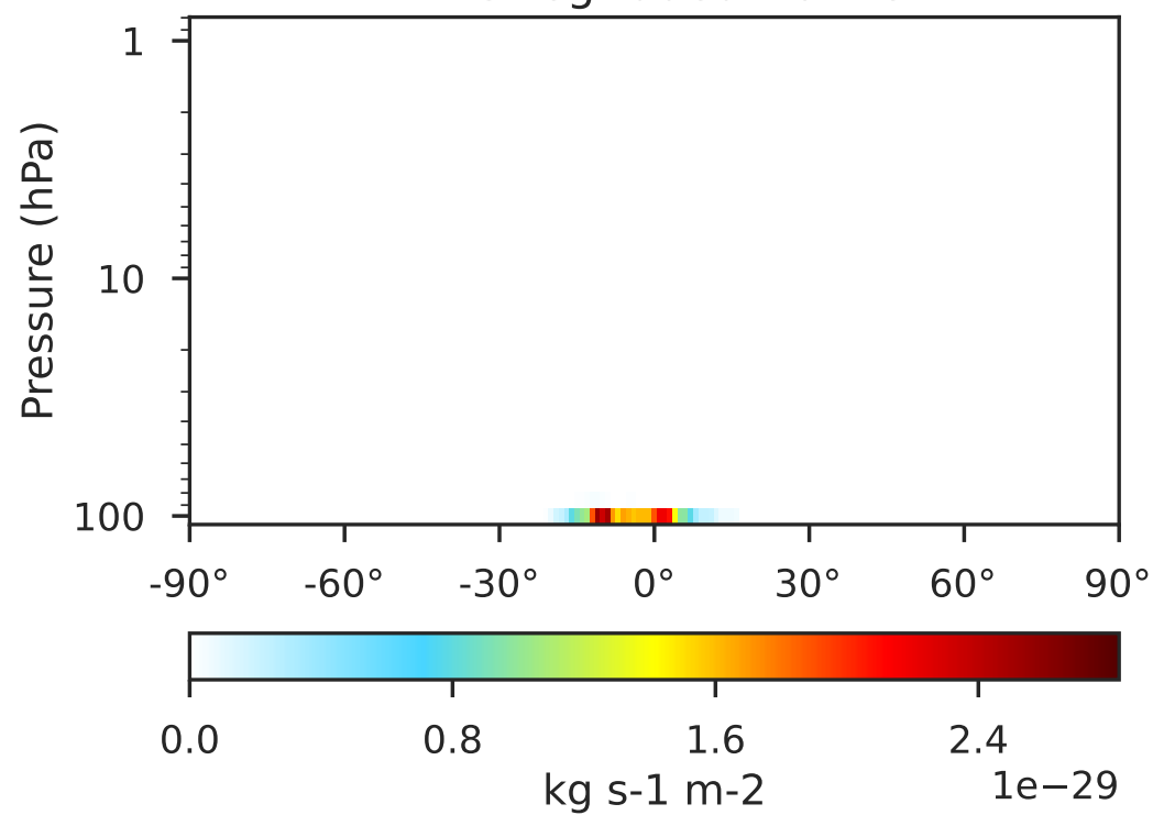
GCHP_14.2.0 (Dev), Normalized by Area 1x1.25 regridged from c24
