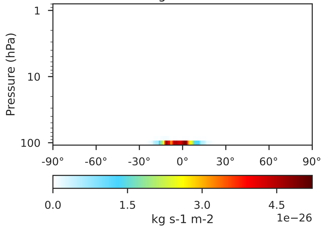
GCHP_14.2.0 (Dev), Normalized by Area 1x1.25 regridged from c24
