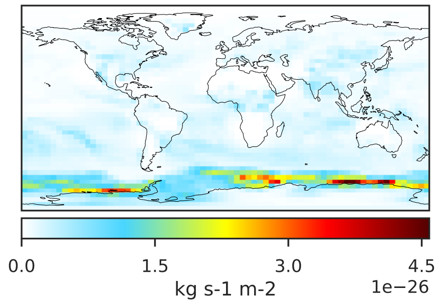
GCC_14.2.0 (Ref), Normalized by Area 4.0x5.0
