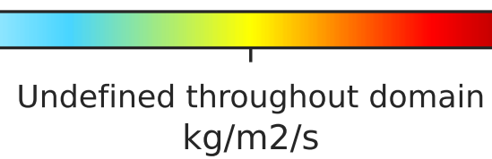
Difference (1x1.25) Dev - Ref, Restricted Range [5%,95%]
