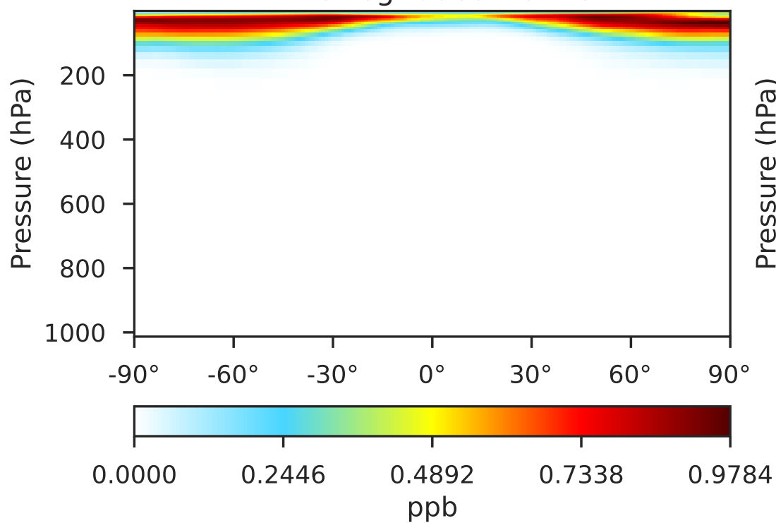
14.2.0-rc.2 (Ref) 1x1.25 regridded from c24
