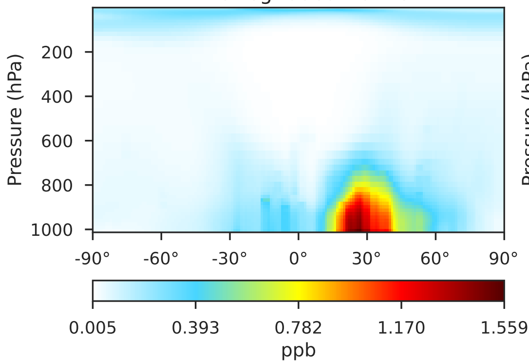
14.2.0-rc.2 (Ref) 1x1.25 regridded from c24
