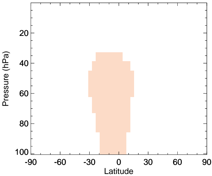
HCOOH - Strat zonal mean abs diff for Jan
