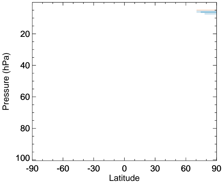
Cl2 - Strat zonal mean abs diff for Jan
