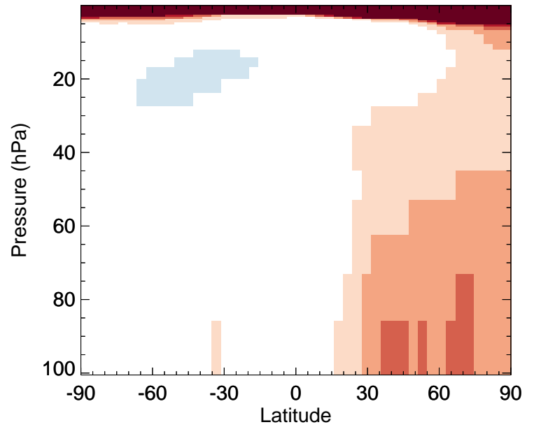
SO2 - Strat zonal mean % diff for Jan
