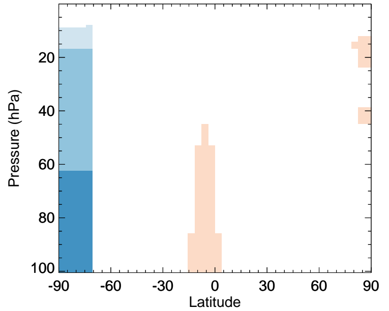
NO3 - Strat zonal mean % diff for Jan
