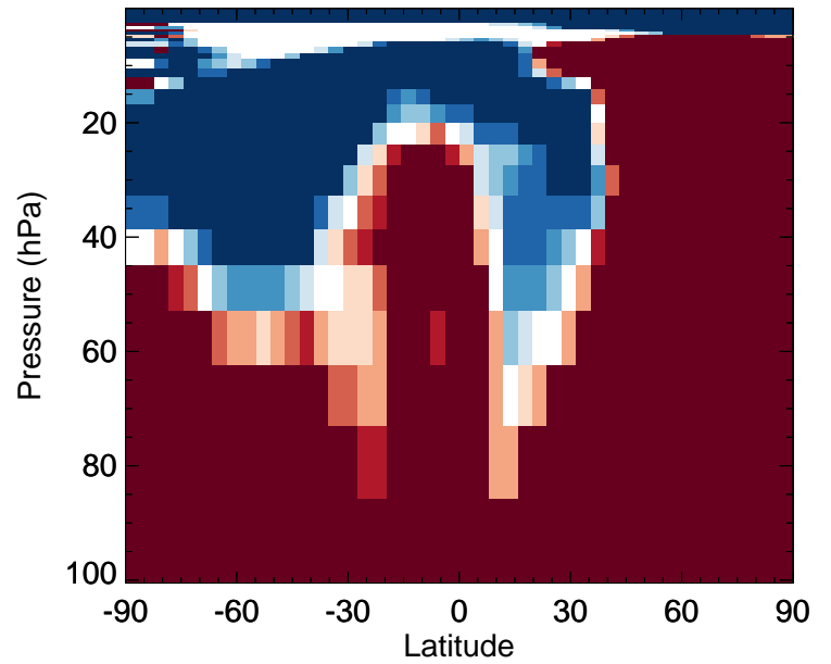
LVOC - Strat zonal mean % diff for Jan
