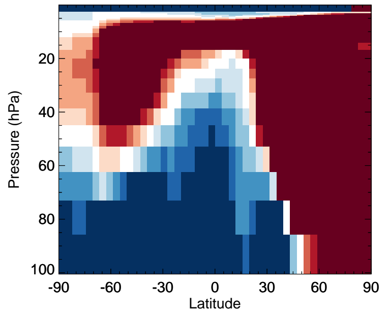
OCIO - Strat zonal mean % diff for Jan
