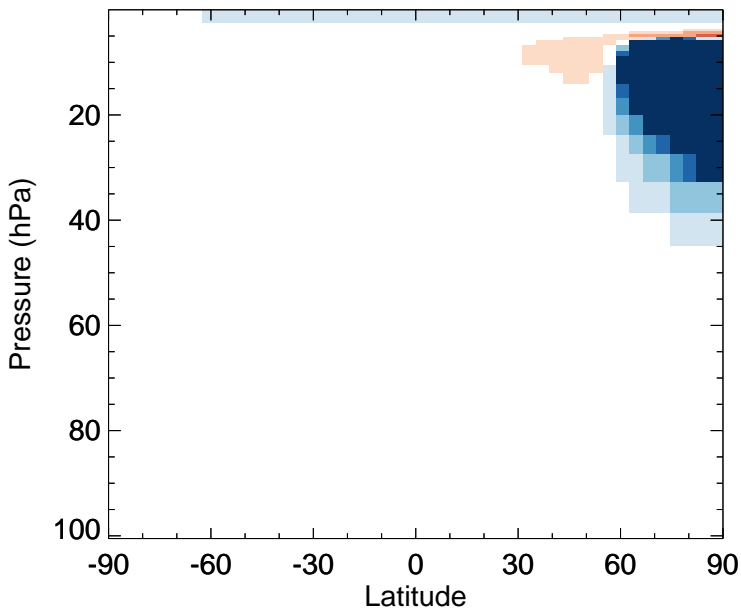
HOCl - Strat zonal mean abs diff for Jan
