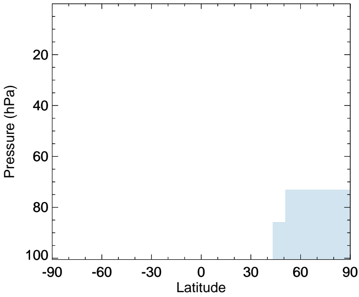
ACET - Strat zonal mean abs diff for Jan
