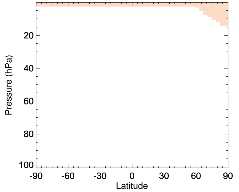
TSOG3 - Strat zonal mean % diff for Jan
