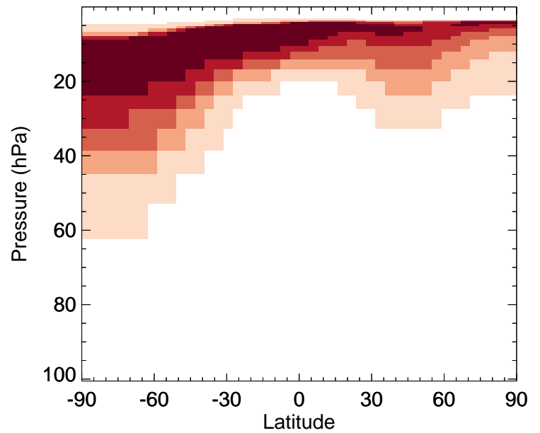
PAN - Strat zonal mean % diff for Jan
