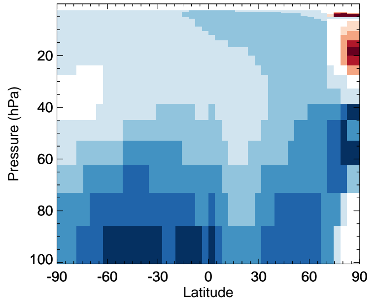
BrO - Strat zonal mean % diff for Jan
