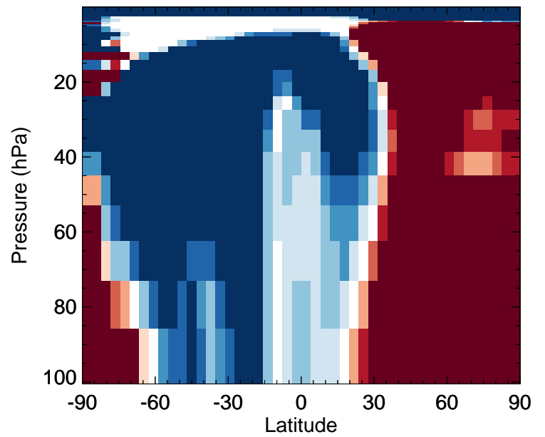
MVKN - Strat zonal mean % diff for Jan
