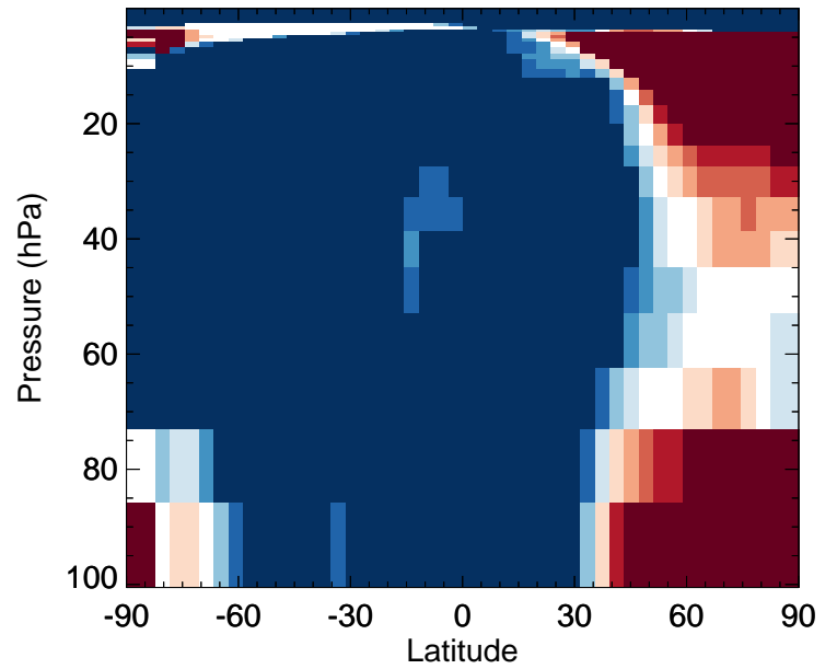
IEPOXA - Strat zonal mean % diff for Jan
