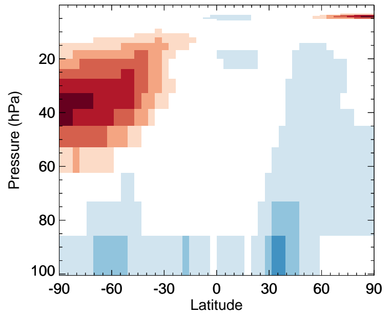
HOCl - Strat zonal mean % diff for Jan
