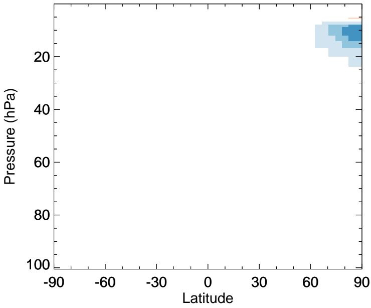
Cl2O2 - Strat zonal mean abs diff for Jan
