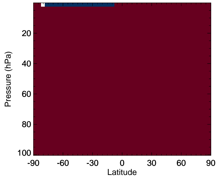
HCOOH - Strat zonal mean % diff for Jan
