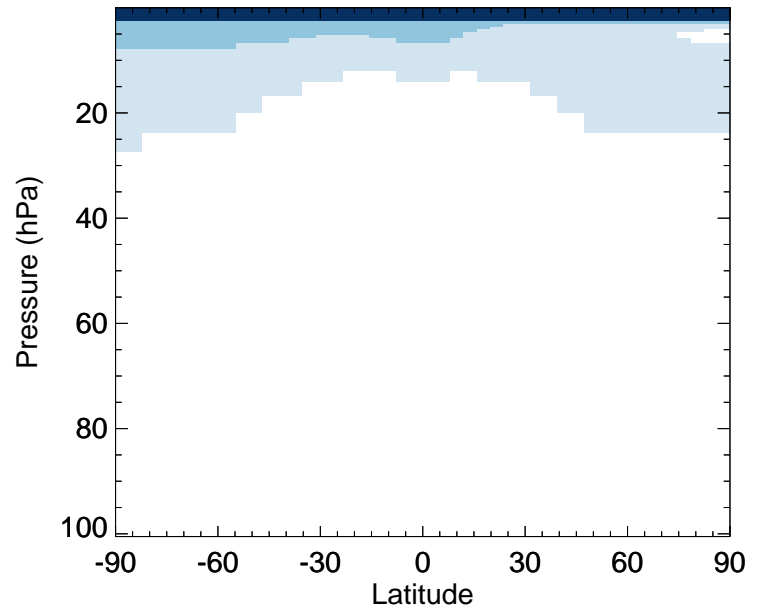
HCFC142b - Strat zonal mean % diff for Jan
