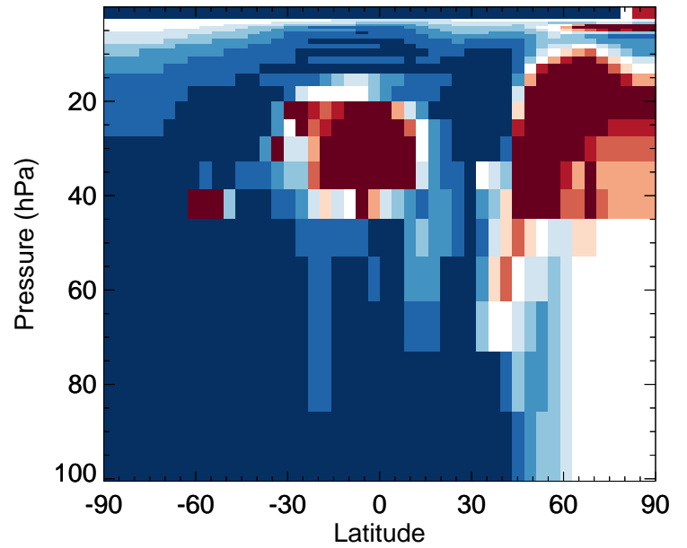
Cl2 - Strat zonal mean % diff for Jan
