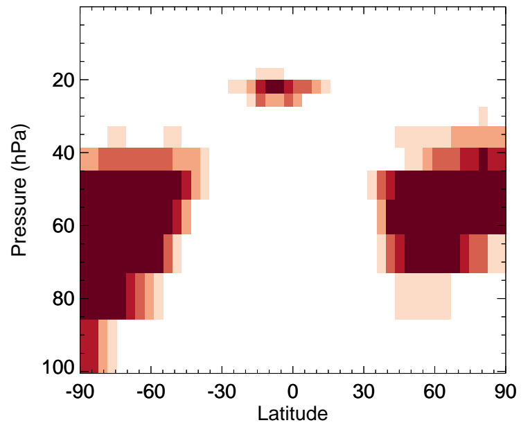
H2O - Strat zonal mean % diff for Jan
