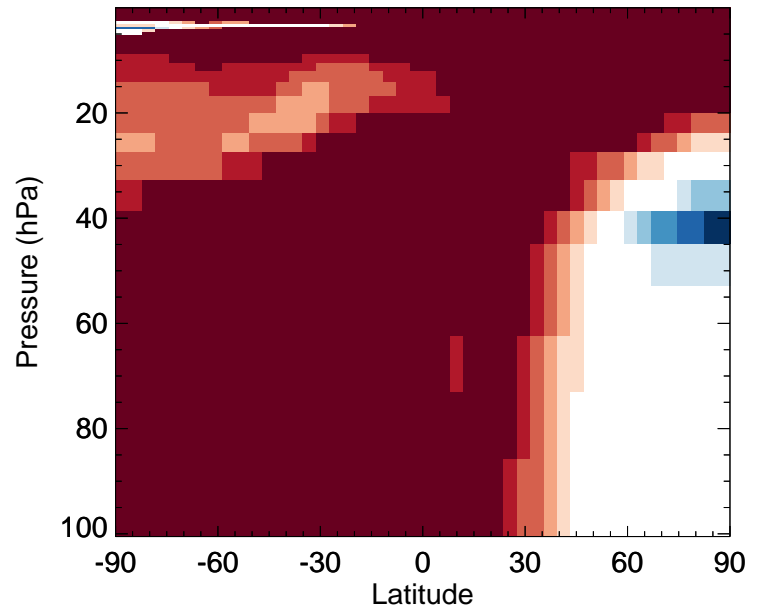
R4N2 - Strat zonal mean % diff for Jan
