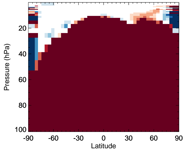
MONITU - Strat zonal mean % diff for Jan
