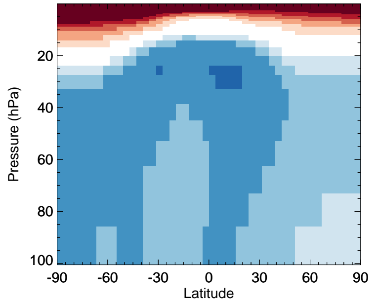
DHDN - Strat zonal mean % diff for Jan
