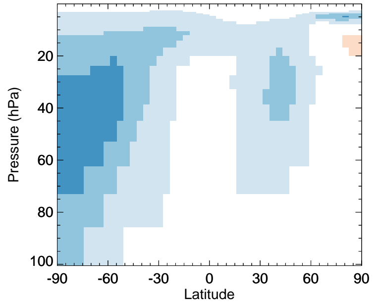
HNO2 - Strat zonal mean % diff for Jan
