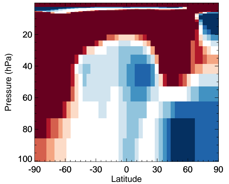
MGLY - Strat zonal mean % diff for Jan
