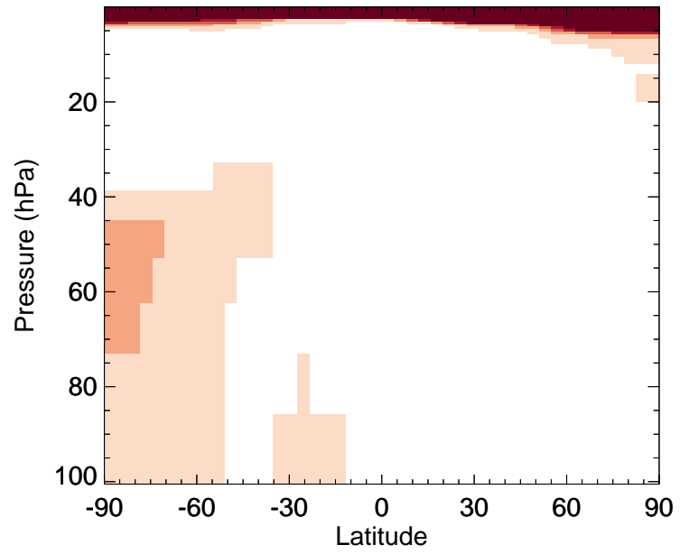
SO2 - Strat zonal mean % diff for Jan
