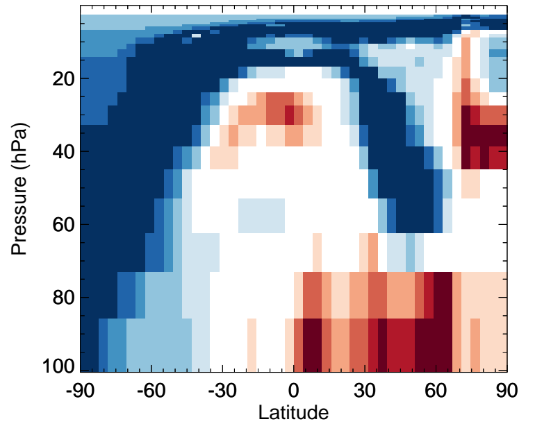
HBr - Strat zonal mean % diff for Jan
