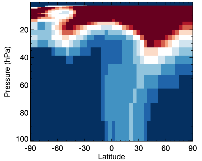
C3H8 - Strat zonal mean % diff for Jan
