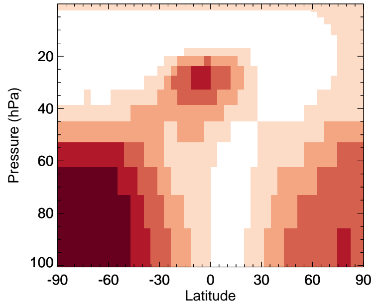
TSOG3 - Strat zonal mean % diff for Jan
