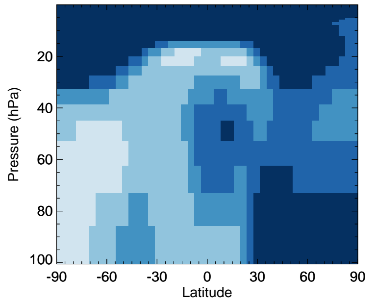
ISOA3 - Strat zonal mean % diff for Jan
