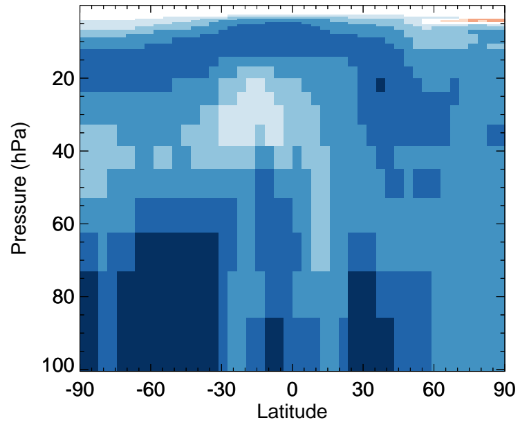
Cl2 - Strat zonal mean % diff for Jan
