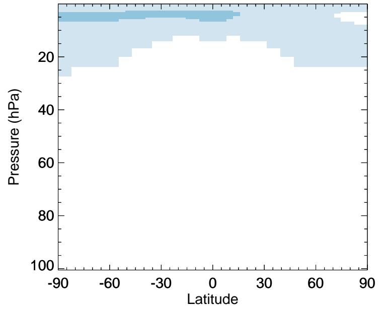
HCFC142b - Strat zonal mean % diff for Jan
