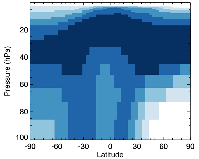
ISN10A - Strat zonal mean % diff for Jan
