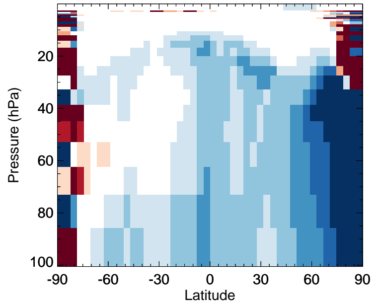
LIMO - Strat zonal mean % diff for Jan
