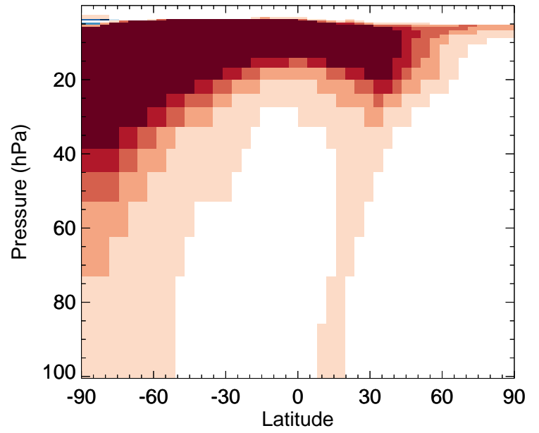
MEK - Strat zonal mean % diff for Jan
