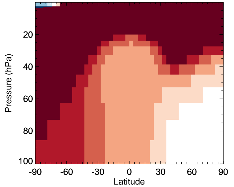
C2H6 - Strat zonal mean % diff for Jan
