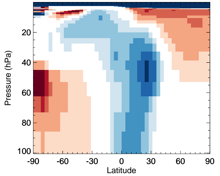
IEPOXA - Strat zonal mean % diff for Jan
