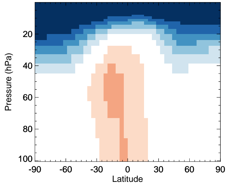
NH4 - Strat zonal mean % diff for Jan
