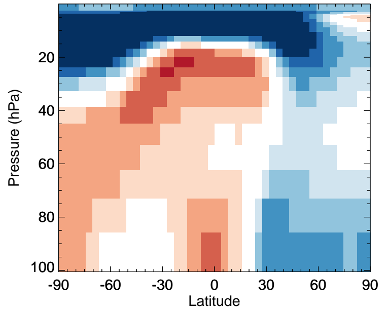
ASOA2 - Strat zonal mean % diff for Jan
