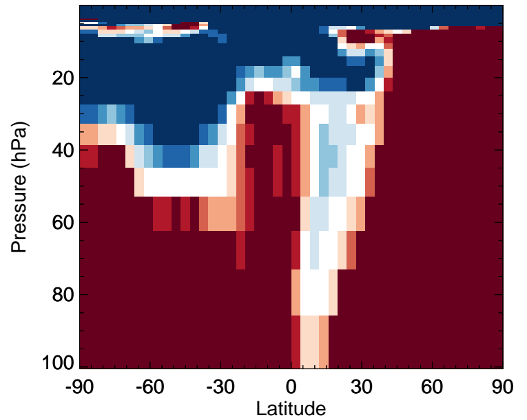
ISN1OG - Strat zonal mean % diff for Jan
