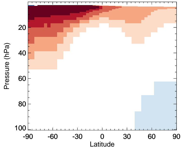
ACET - Strat zonal mean % diff for Jan
