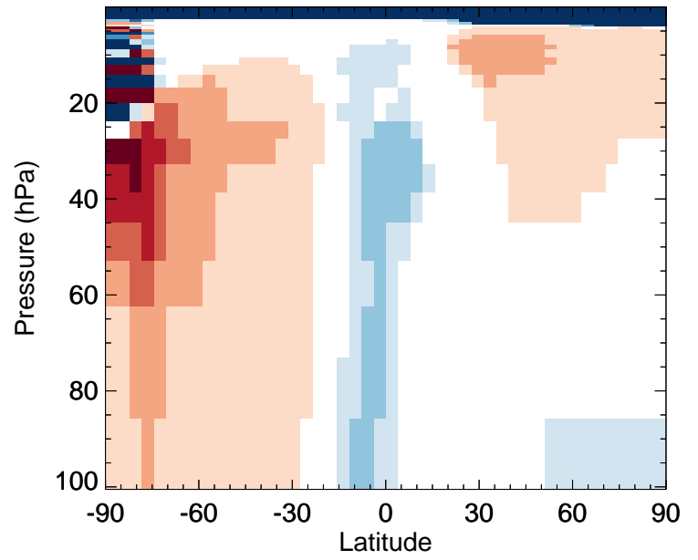
MVKN - Strat zonal mean % diff for Jan
