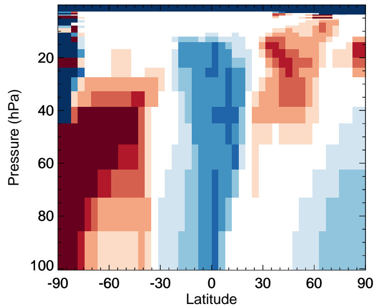
MOBA - Strat zonal mean % diff for Jan
