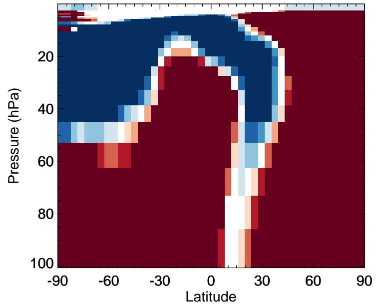
MONITS - Strat zonal mean % diff for Jan
