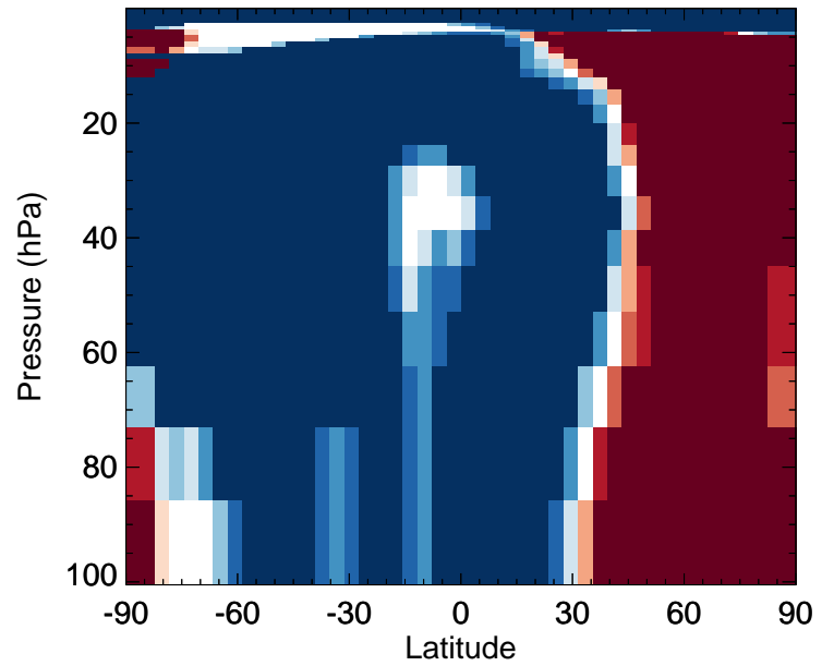
IEPOXB - Strat zonal mean % diff for Jan
