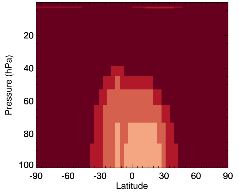
ASOG1 - Strat zonal mean % diff for Jan
