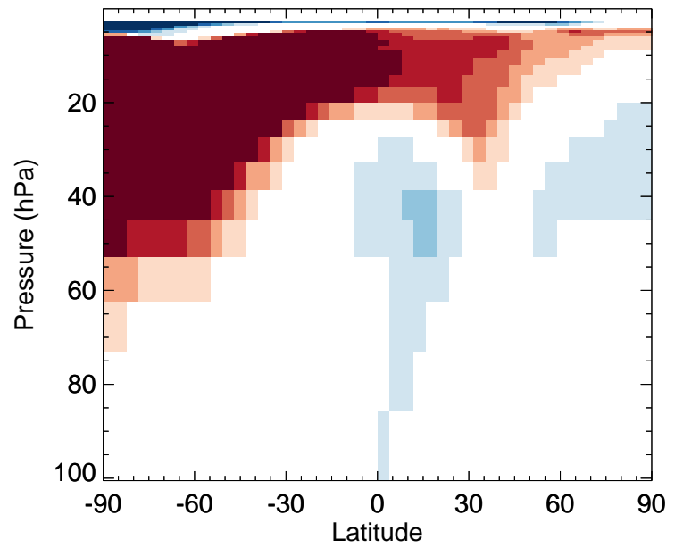
MGLY - Strat zonal mean % diff for Jan
