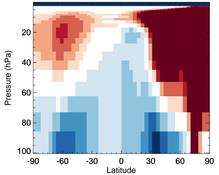
CIO - Strat zonal mean % diff for Jan
