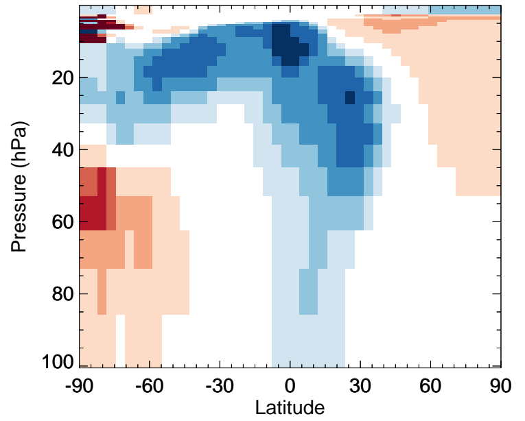
MONITS - Strat zonal mean % diff for Jan
