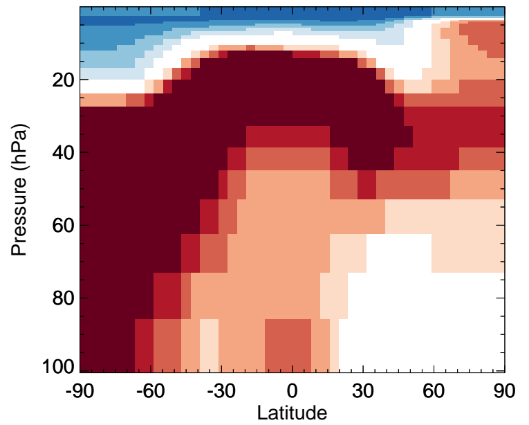
ASOA1 - Strat zonal mean % diff for Jan
