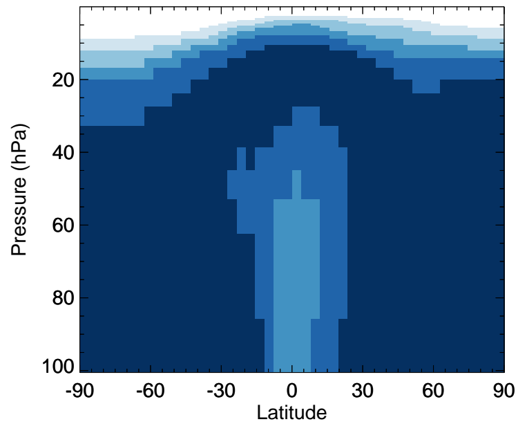
SOAGX - Strat zonal mean % diff for Jan
