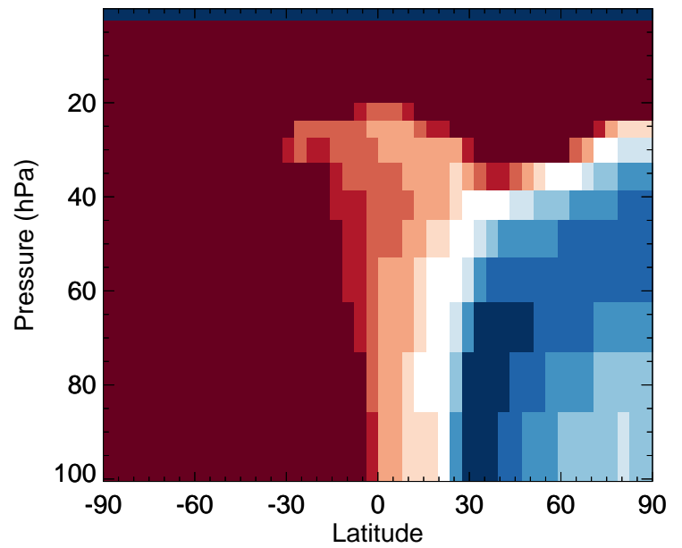
BENZ - Strat zonal mean % diff for Jan
