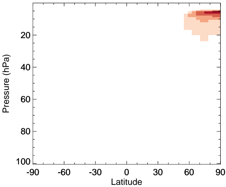
OCIO - Strat zonal mean abs diff for Jan
