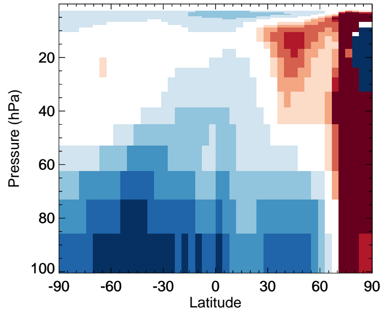
BrO - Strat zonal mean % diff for Jan
