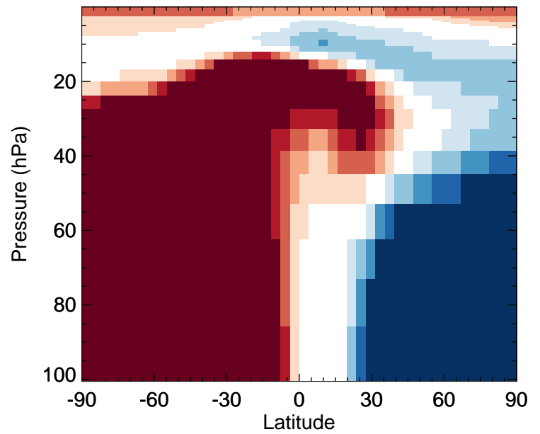
ASOAN - Strat zonal mean % diff for Jan
