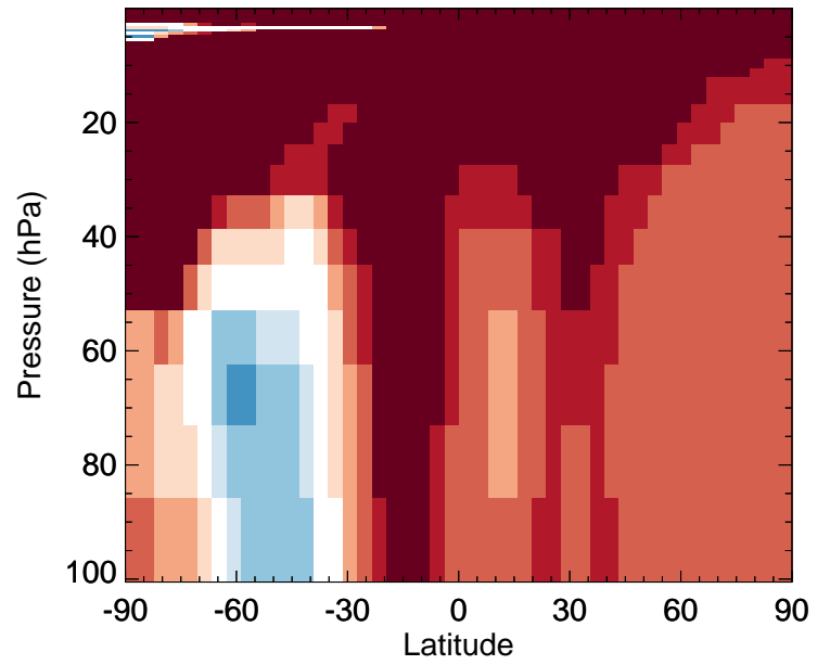
MEK - Strat zonal mean % diff for Jan
