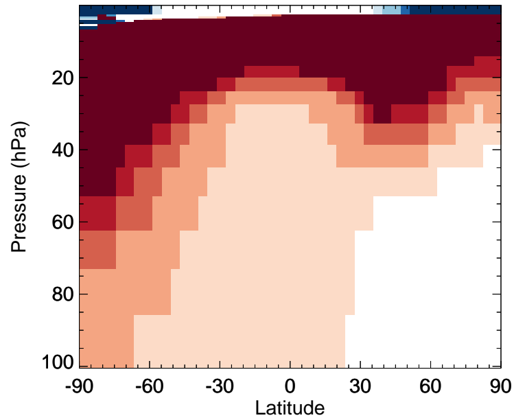
ALK4 - Strat zonal mean % diff for Jan
