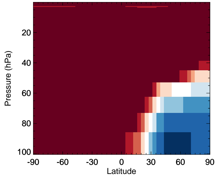
ASOG1 - Strat zonal mean % diff for Jan
