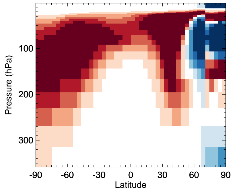
HO2 - Strat zonal mean % diff for Jan
