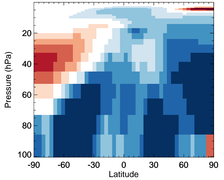
Cl2O2 - Strat zonal mean % diff for Jan
