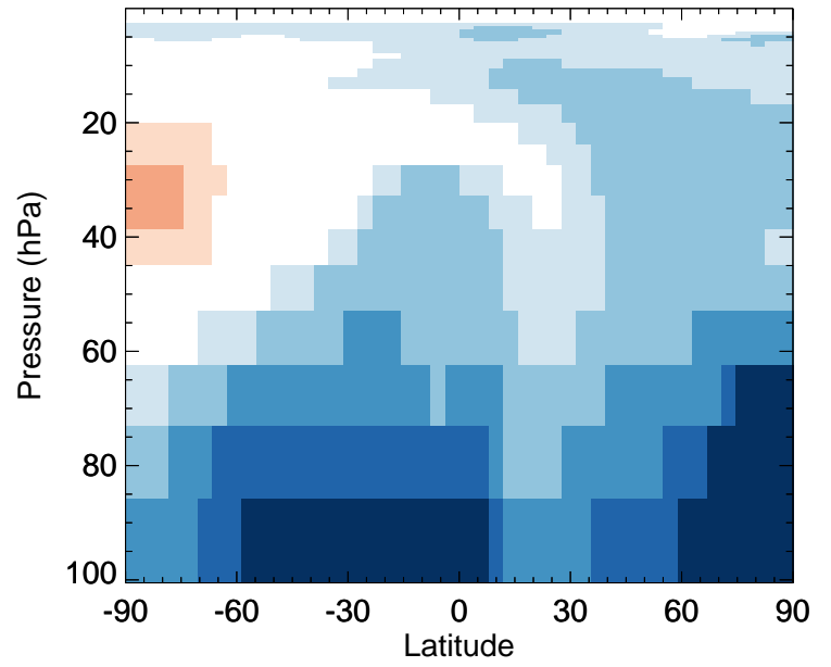
HOBr - Strat zonal mean % diff for Jan
