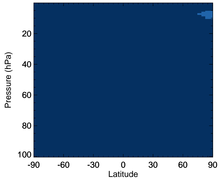
ISOA3 - Strat zonal mean % diff for Jan
