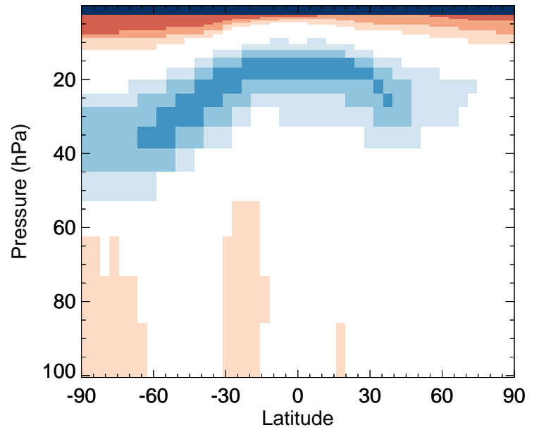
IONITA - Strat zonal mean % diff for Jan
