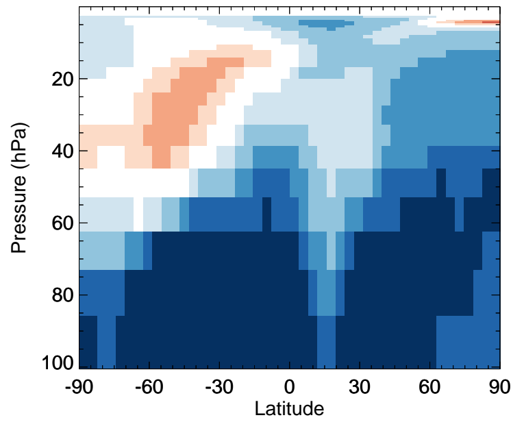
OCIO - Strat zonal mean % diff for Jan
