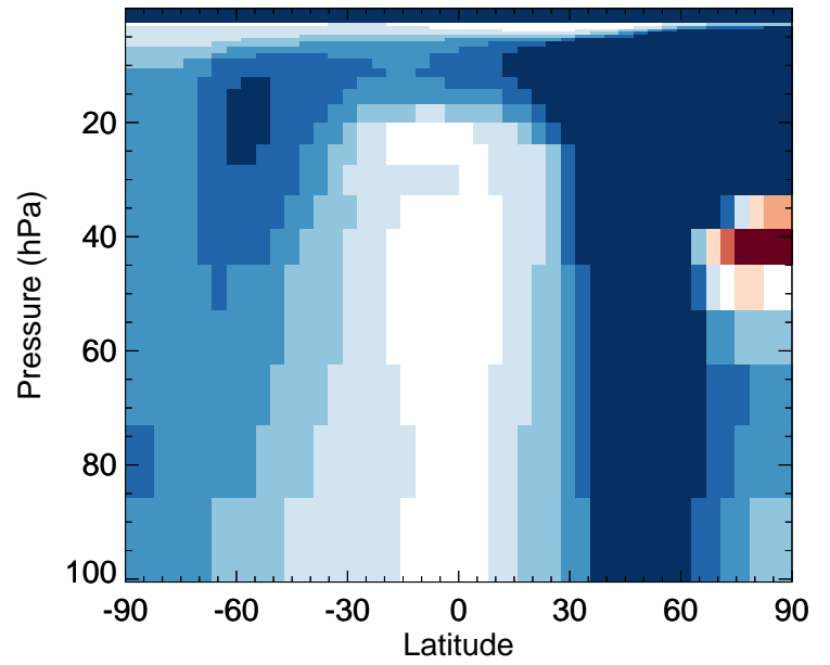
HNO2 - Strat zonal mean % diff for Jan
