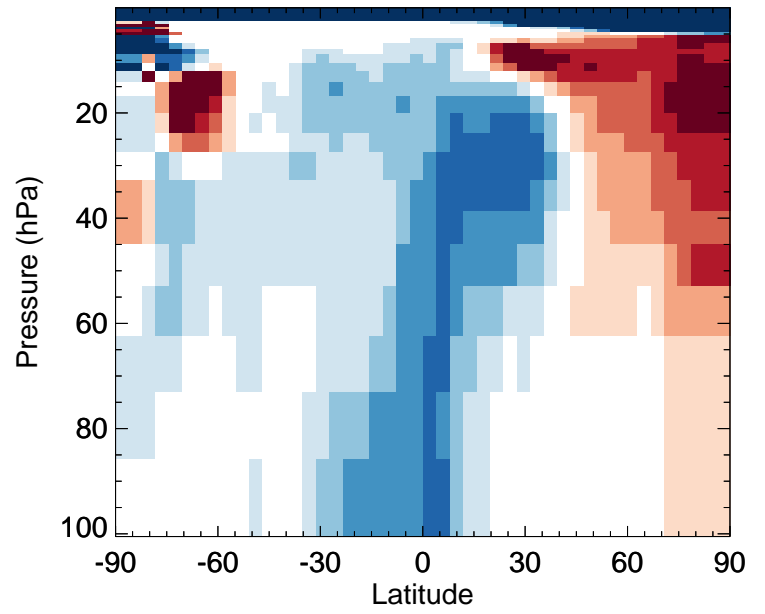
LVOC - Strat zonal mean % diff for Jan
