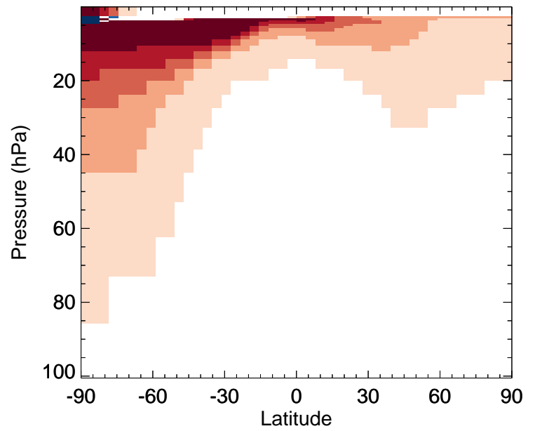
CHBr3 - Strat zonal mean % diff for Jan
