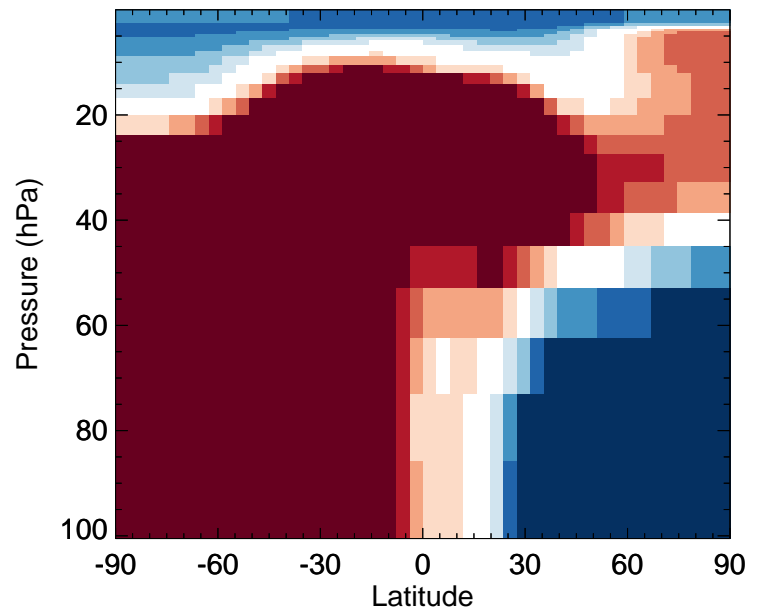
ASOA1 - Strat zonal mean % diff for Jan
