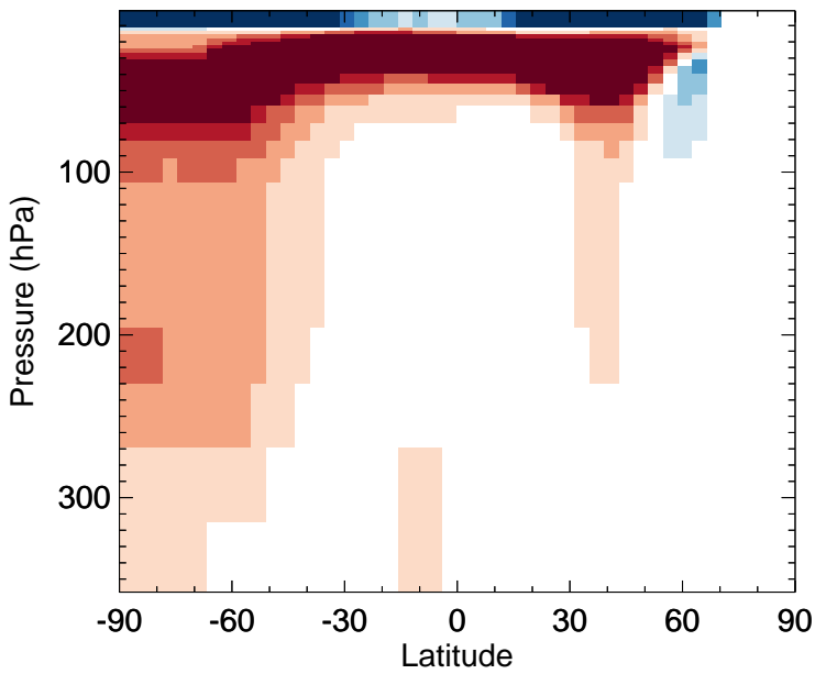
HO2 - Strat zonal mean abs diff for Jan
