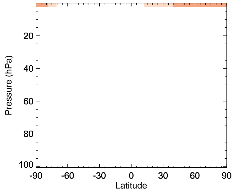
DST1 - Strat zonal mean % diff for Jan
