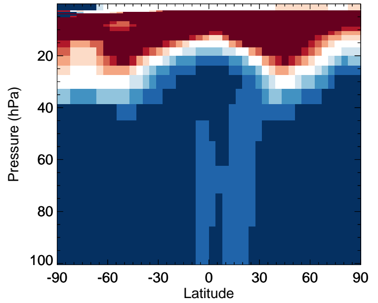
C3H8 - Strat zonal mean % diff for Jan
