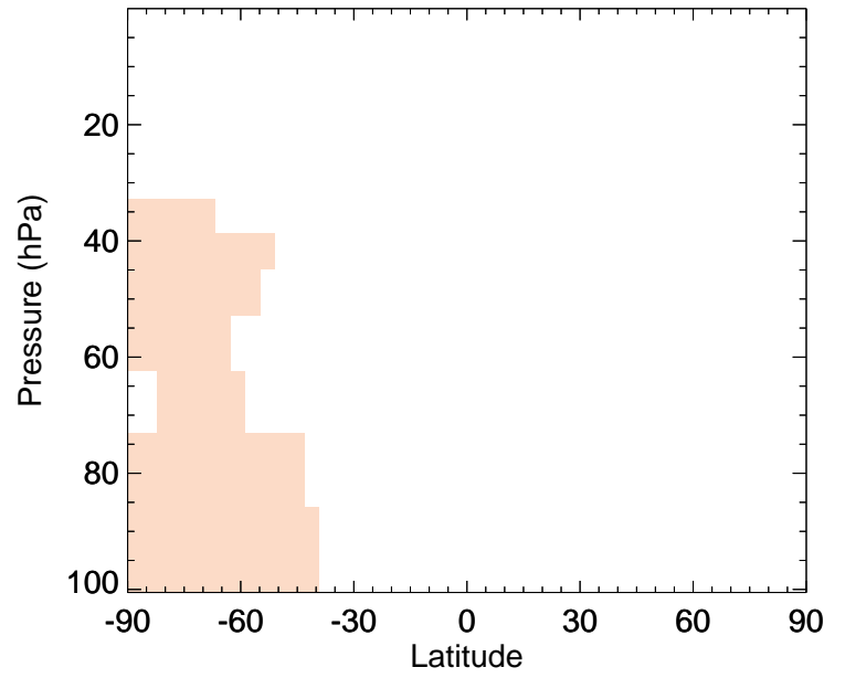
O3 - Strat zonal mean % diff for Jan
