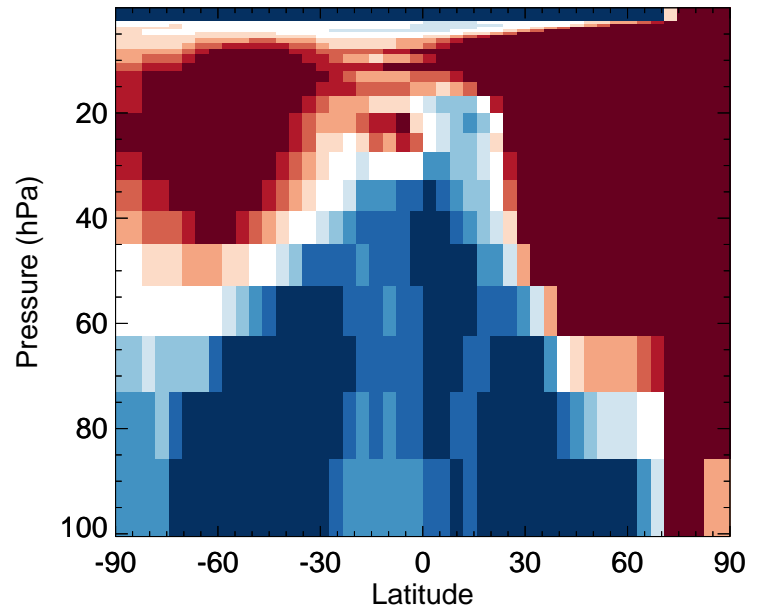
Cl2O2 - Strat zonal mean % diff for Jan
