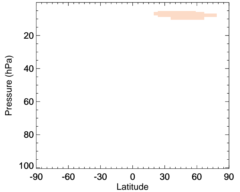
O3 - Strat zonal mean % diff for Jan
