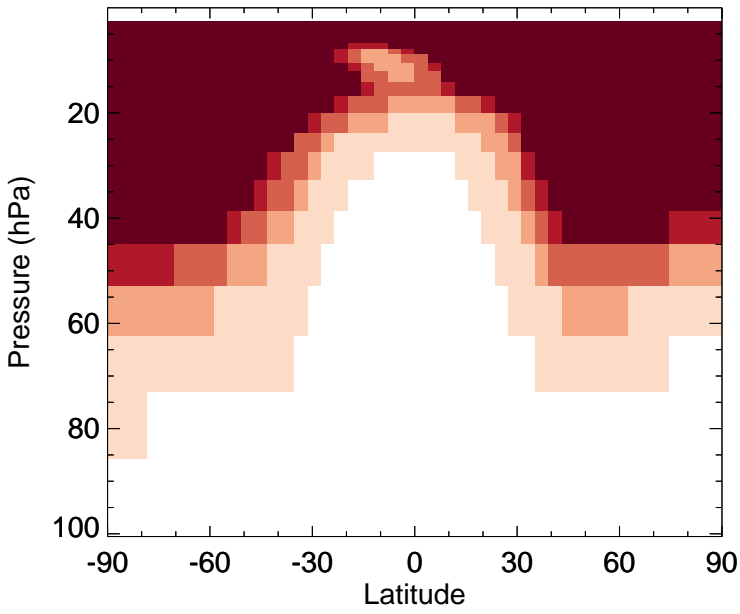
O3 - Strat zonal mean abs diff for Jan
