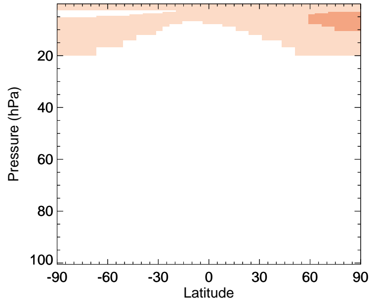
CFC12 - Strat zonal mean % diff for Jan
