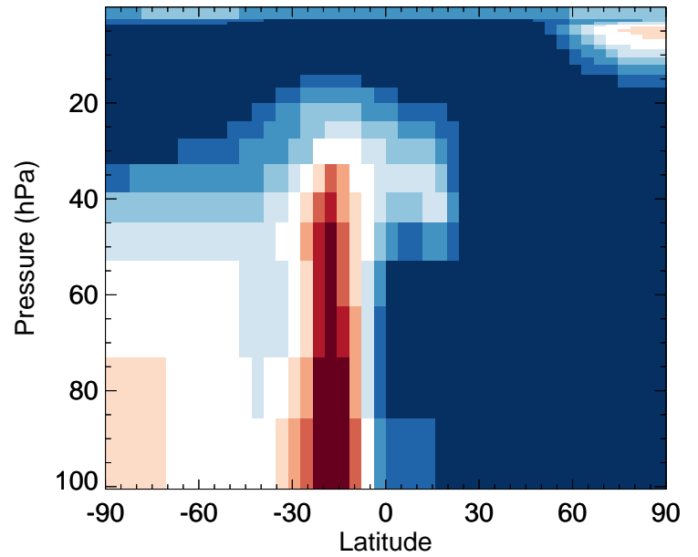
ASOA2 - Strat zonal mean % diff for Jan
