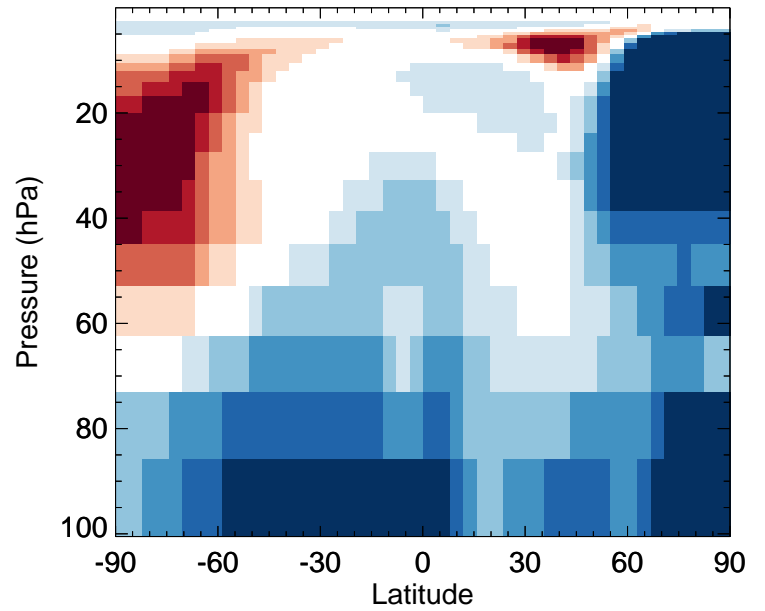
HOBr - Strat zonal mean % diff for Jan
