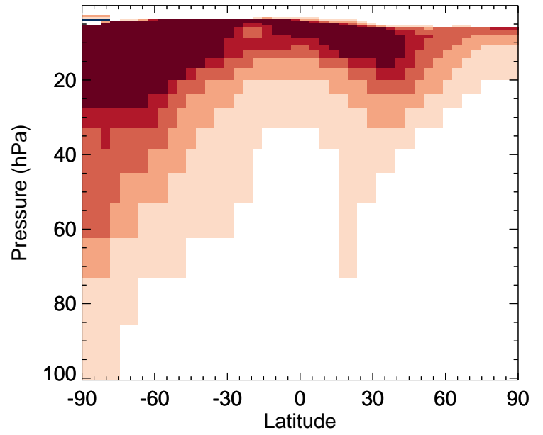
R4N2 - Strat zonal mean % diff for Jan
