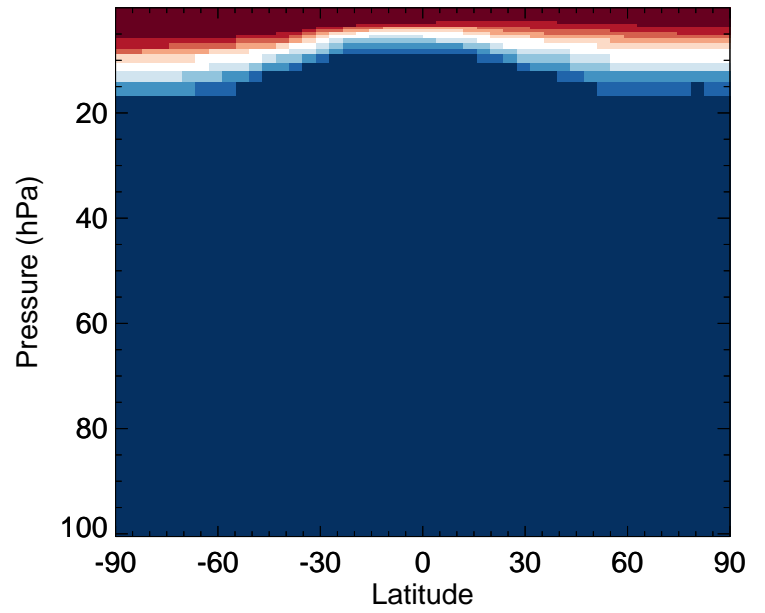
DHDN - Strat zonal mean % diff for Jan
