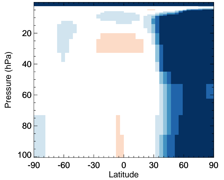
HNO4 - Strat zonal mean % diff for Jan
