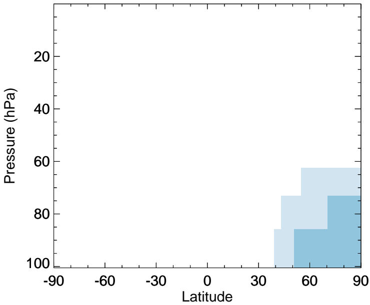
C3H8 - Strat zonal mean abs diff for Jan
