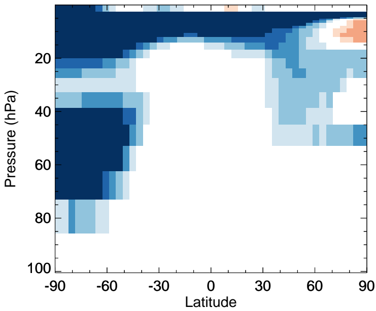
H2O - Strat zonal mean abs diff for Jan
