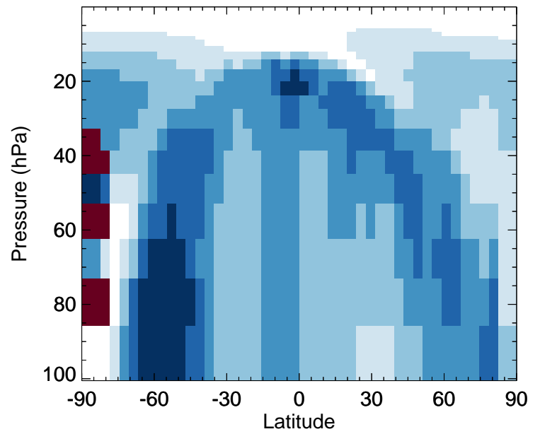
MTPO - Strat zonal mean % diff for Jan
