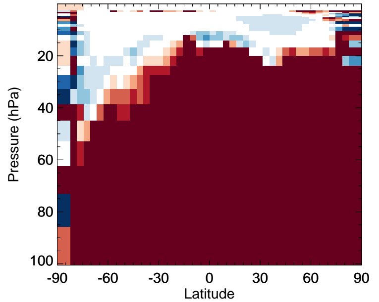
LIMO - Strat zonal mean % diff for Jan
