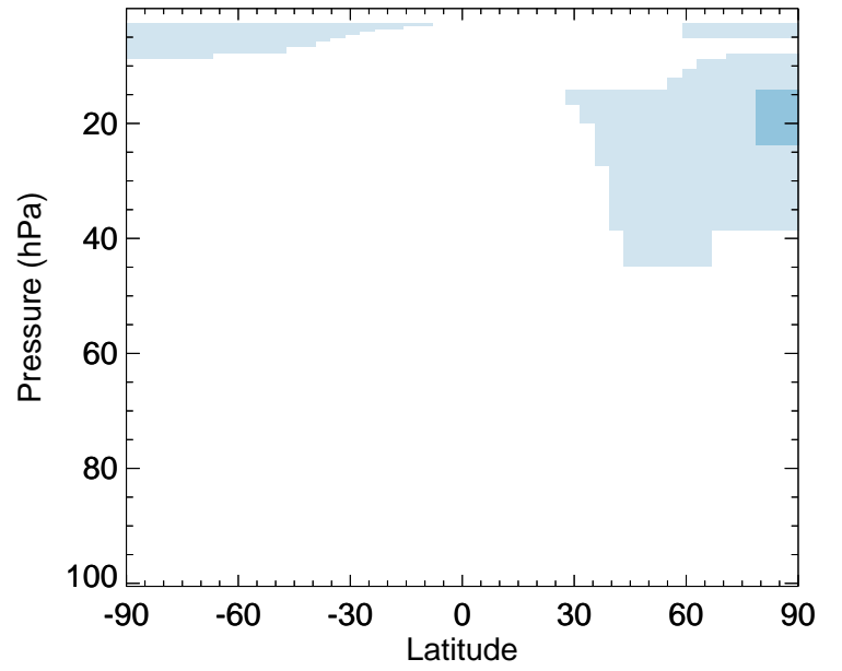
CH2O - Strat zonal mean % diff for Jan
