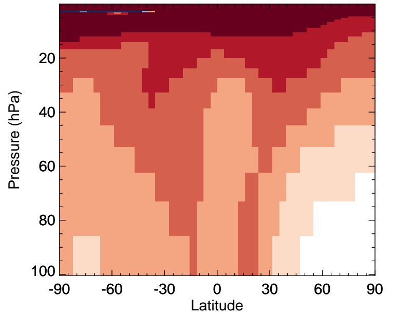
ACET - Strat zonal mean % diff for Jan
