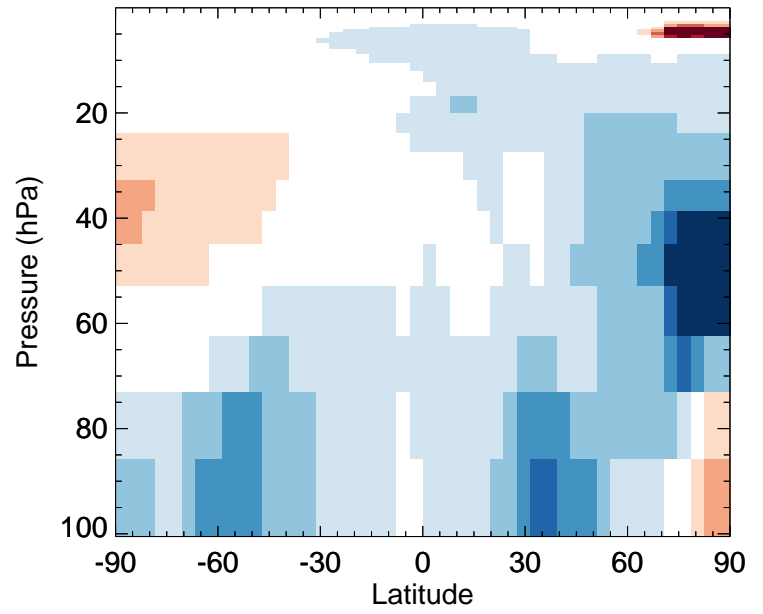
CIO - Strat zonal mean % diff for Jan
