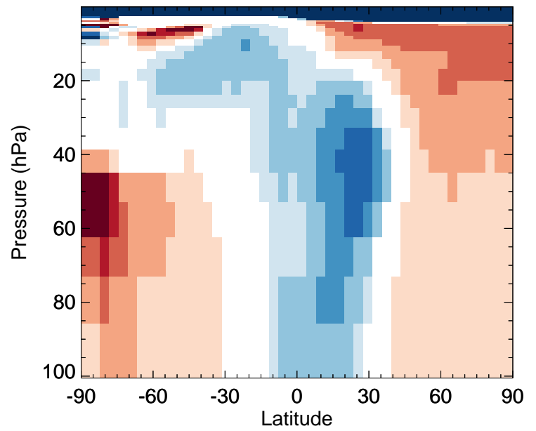
HC187 - Strat zonal mean % diff for Jan
