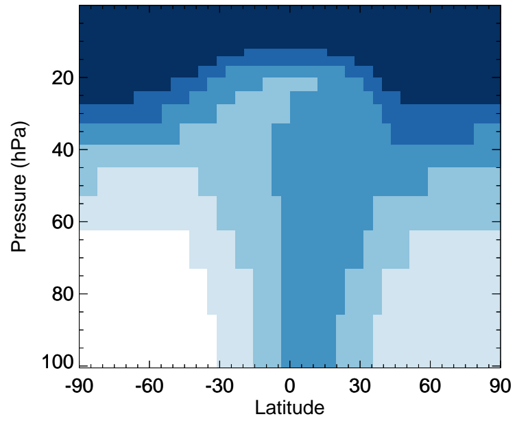
LVOCOA - Strat zonal mean % diff for Jan
