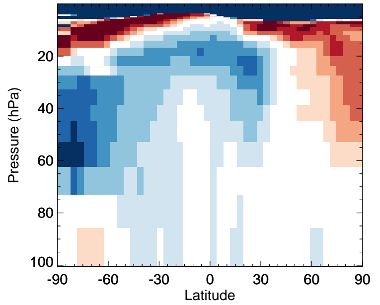
ISN1OG - Strat zonal mean % diff for Jan
