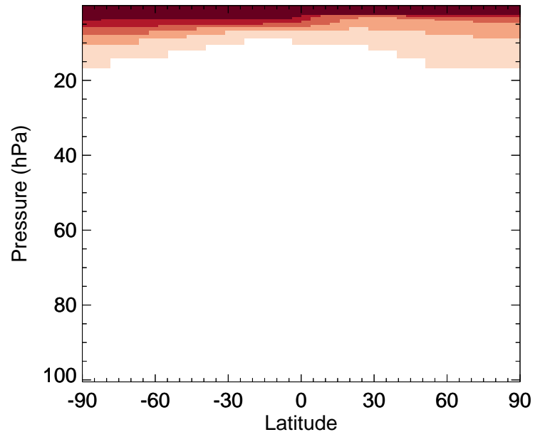
H1211 - Strat zonal mean % diff for Jan
