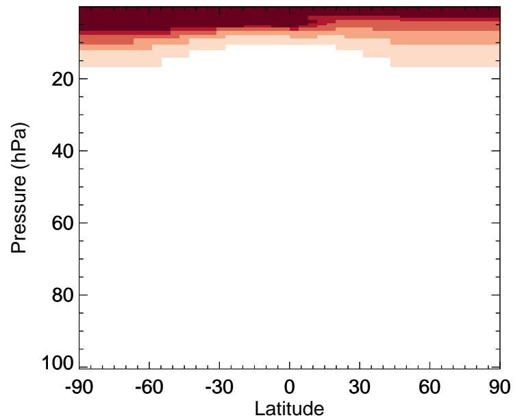
H1211 - Strat zonal mean % diff for Jan
