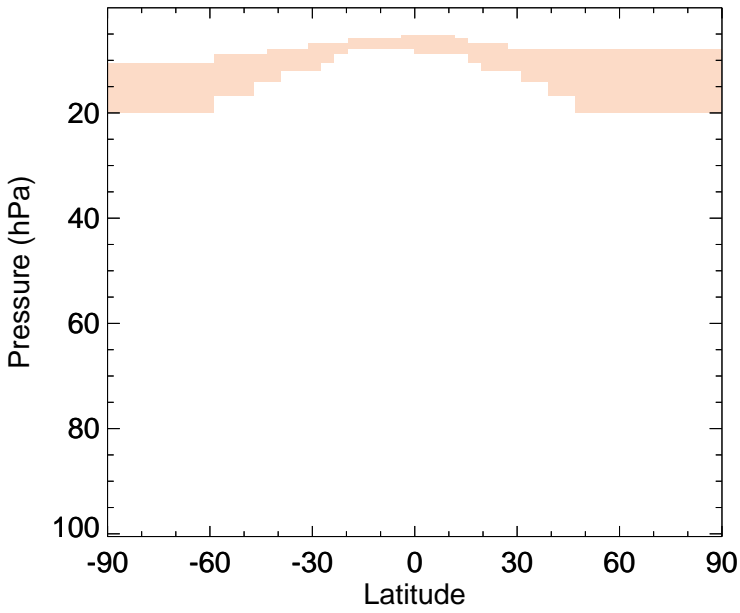
CFC12 - Strat zonal mean abs diff for Jan
