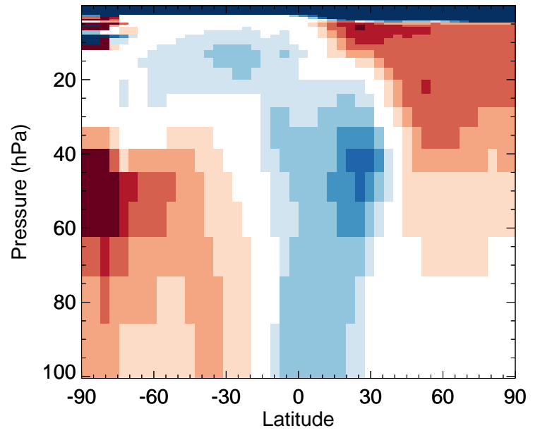
IEPOXB - Strat zonal mean % diff for Jan
