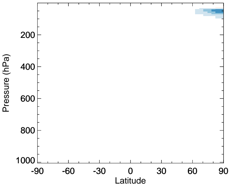
Cl2O2 - Zonal mean abs diff for Jan
