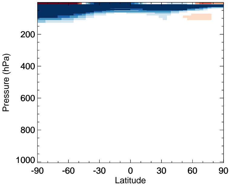
HCl - Zonal mean abs diff for Jan
