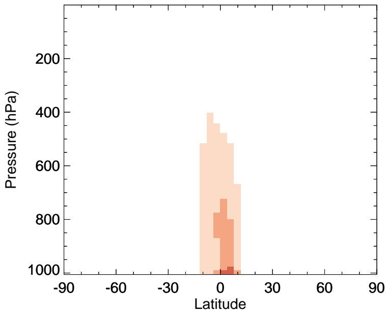
GC_12.0.0 - v11-02f-Run1 C2H6 - Zonal mean abs diff for Jan
