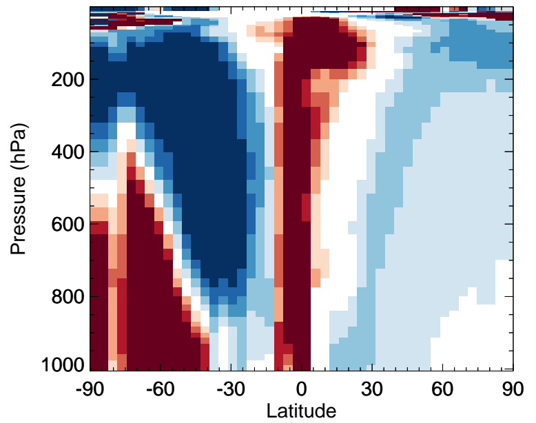
BCPO - Zonal mean % diff for Jan
