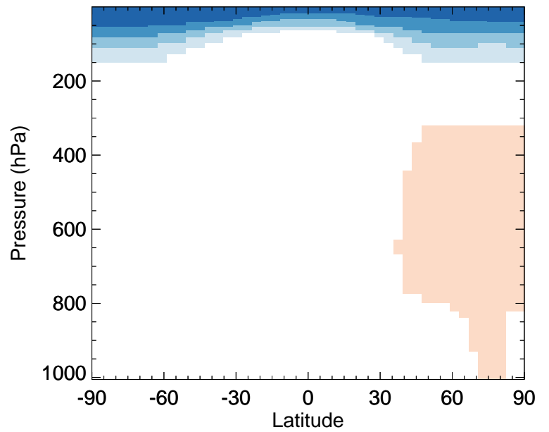
MSA - Zonal mean % diff for Jan
