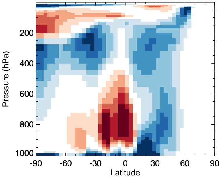
OH - Zonal mean abs diff for Jan
