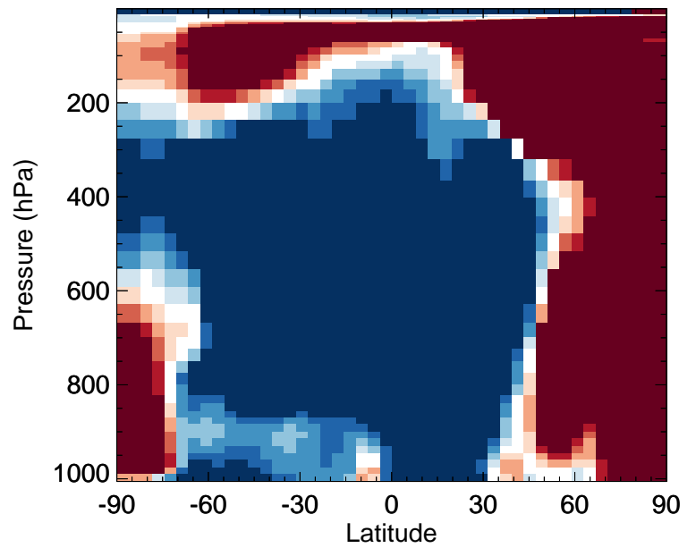
GC_12.0.0 / v11-02e-Run1 OCIO - Zonal mean % diff for Jan
