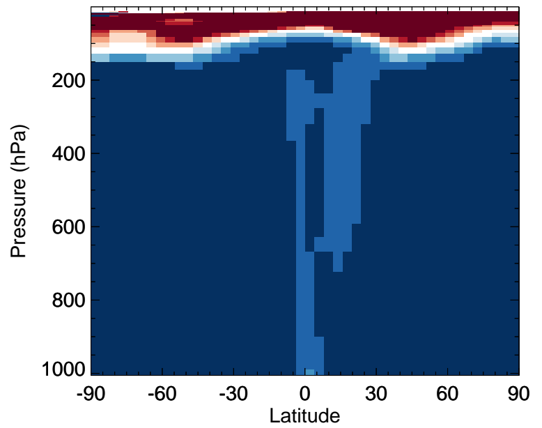
GC_12.0.0 / v11-02f-Run1 C3H8 - Zonal mean % diff for Jan
