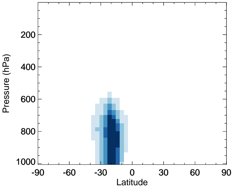
SOAIE - Zonal mean abs diff for Jan
