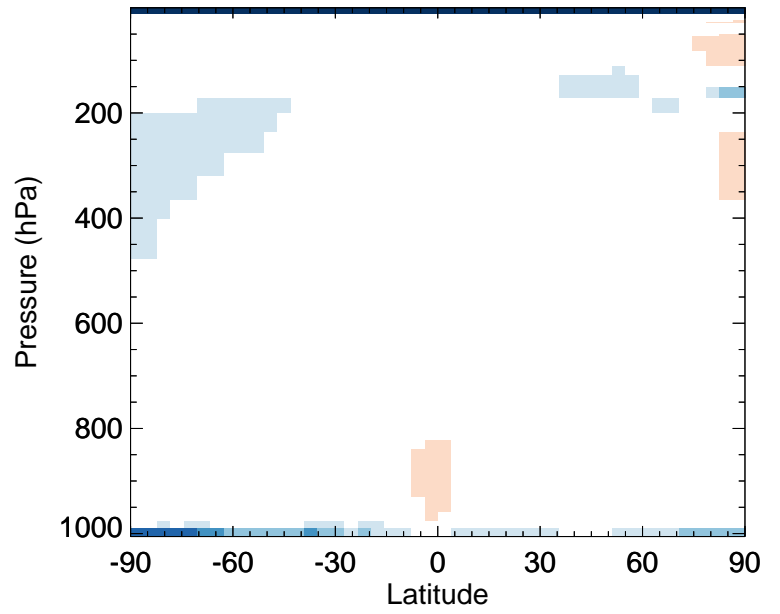
OH - Zonal mean % diff for Jan
