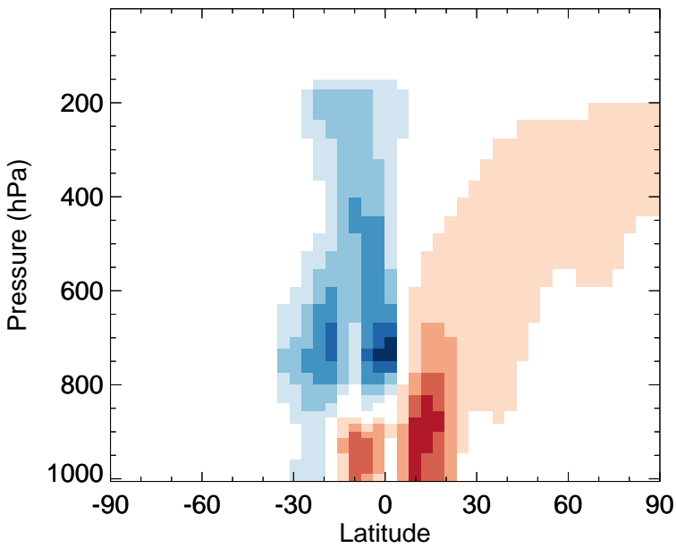
MAP - Zonal mean abs diff for Jan
