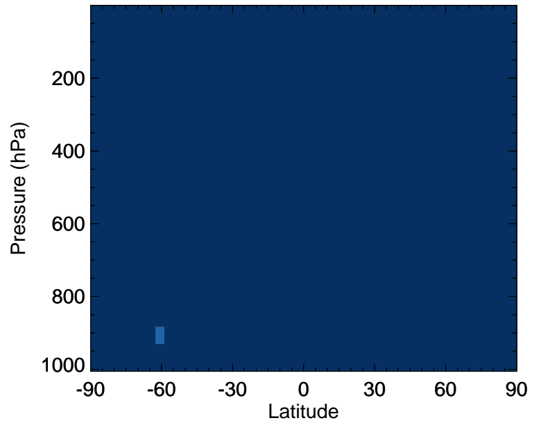
ISOA2 - Zonal mean % diff for Jan
