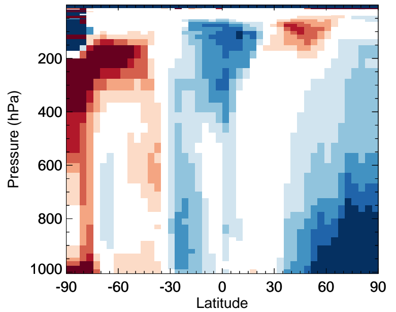
ISOPND - Zonal mean % diff for Jan
