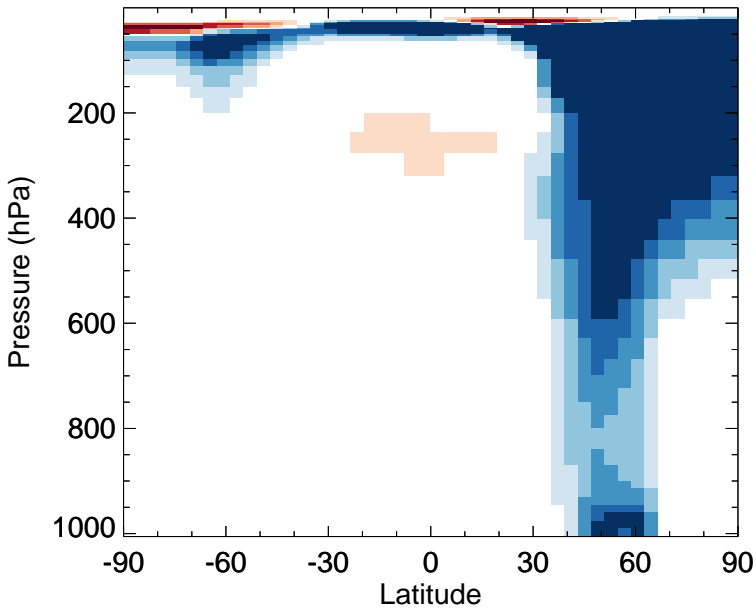
HNO 4 - Zonal mean abs diff for Jan
