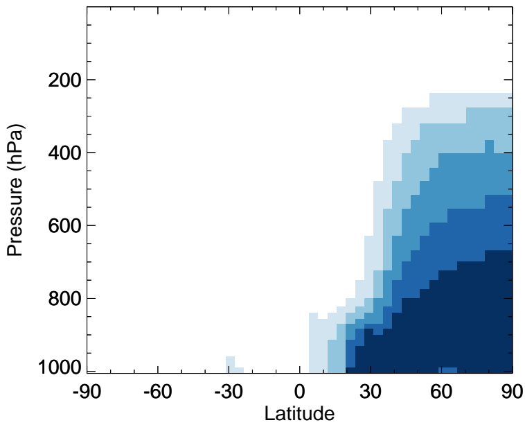
GC_12.0.0 - v11-02e-Run1 C3H8 - Zonal mean abs diff for Jan
