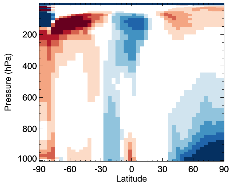
ETHLN - Zonal mean % diff for Jan
