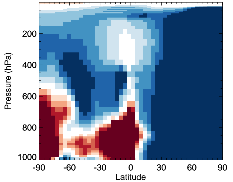
CINO3 - Zonal mean % diff for Jan
