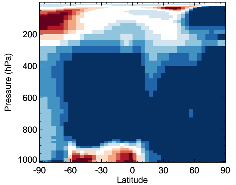
HOBr - Zonal mean % diff for Jan
