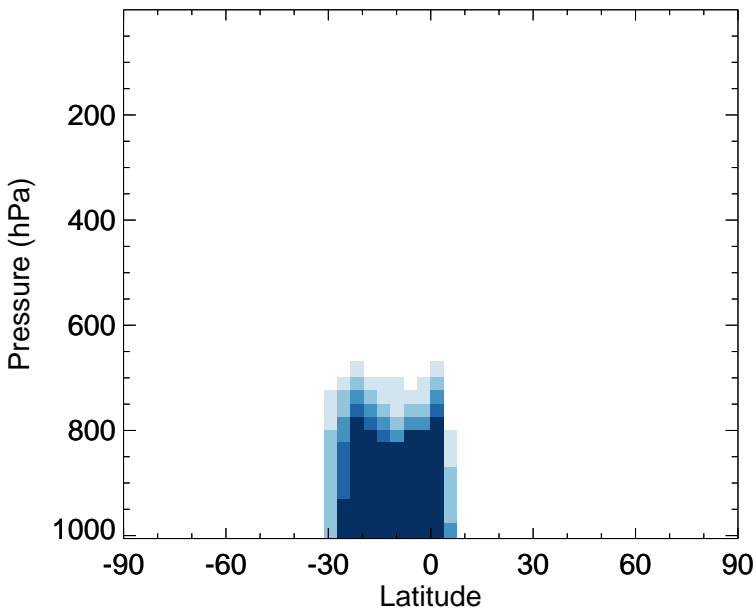
GC_12.0.0 - v11-02e-Run1 ISOP - Zonal mean abs diff for Jan
