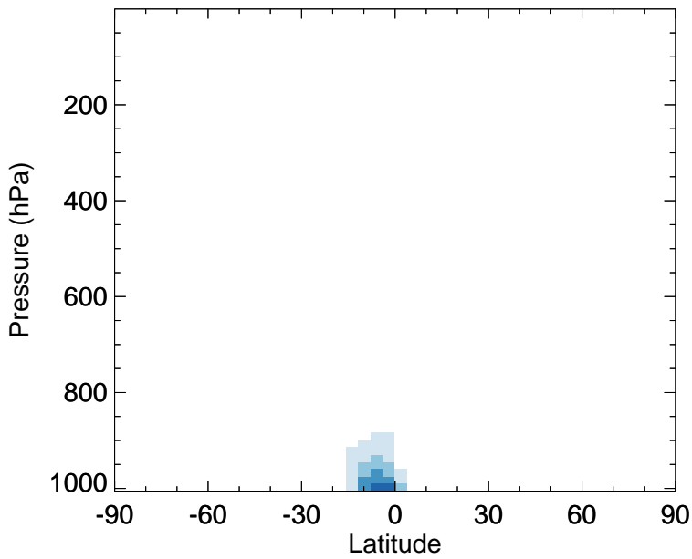
MTPA - Zonal mean abs diff for Jan
