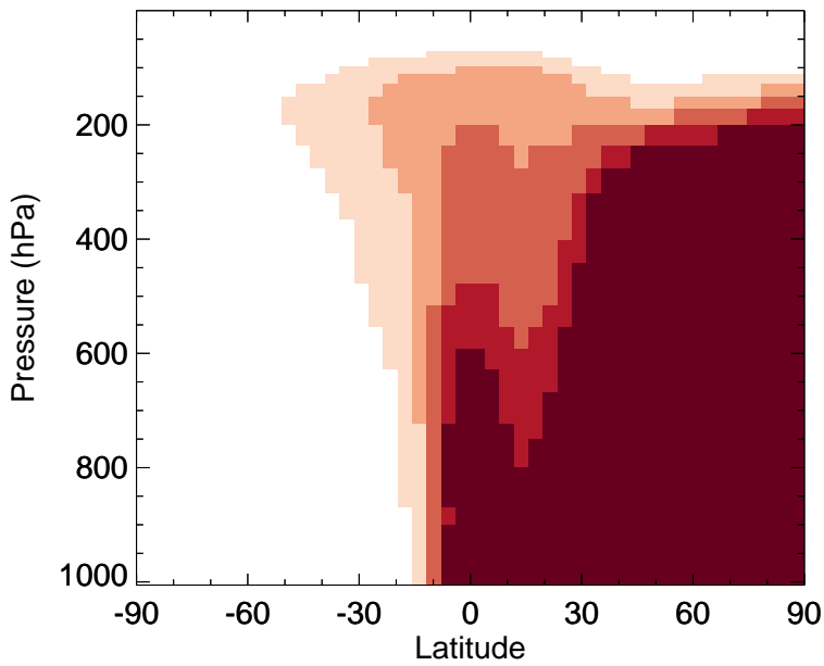
GC_12.0.0 - v11-02e-Run1 C2H6 - Zonal mean abs diff for Jan
