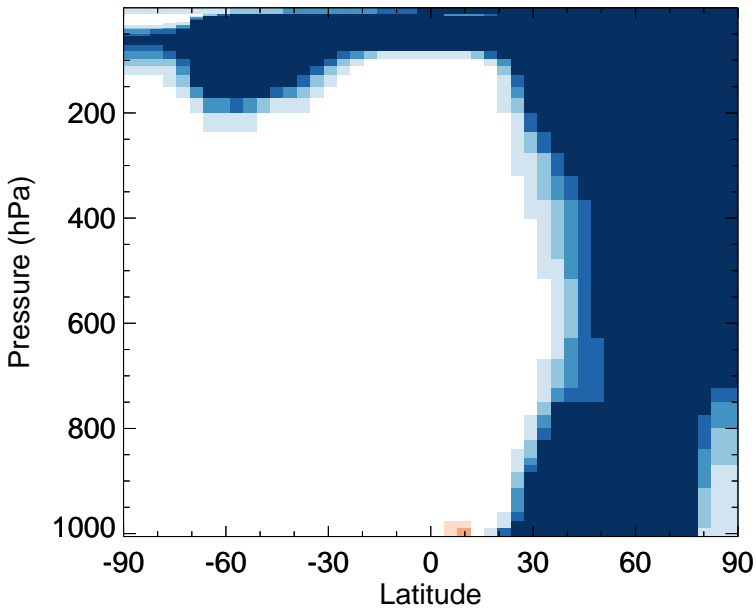
N2O5 - Zonal mean abs diff for Jan
