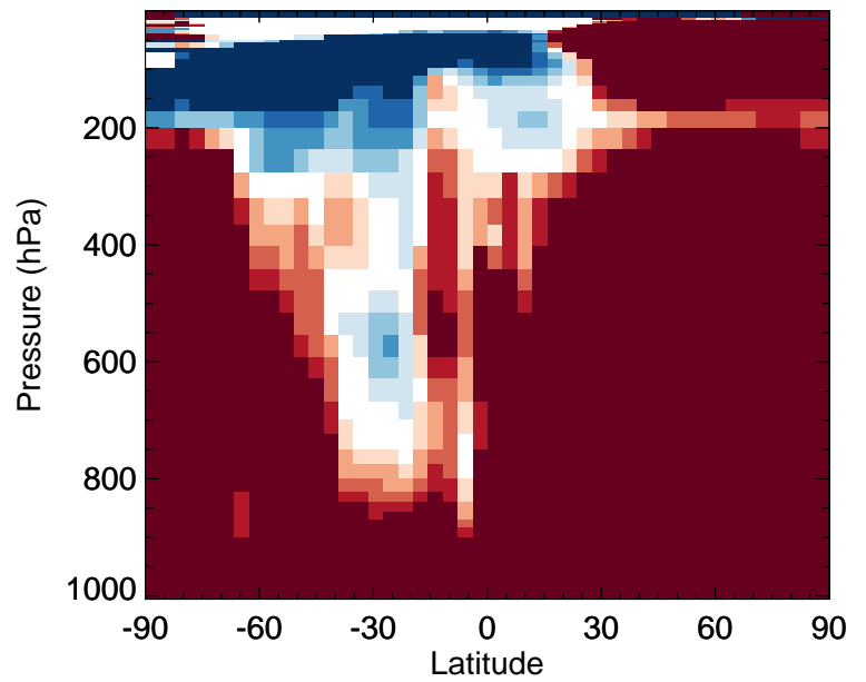
MACR - Zonal mean % diff for Jan
