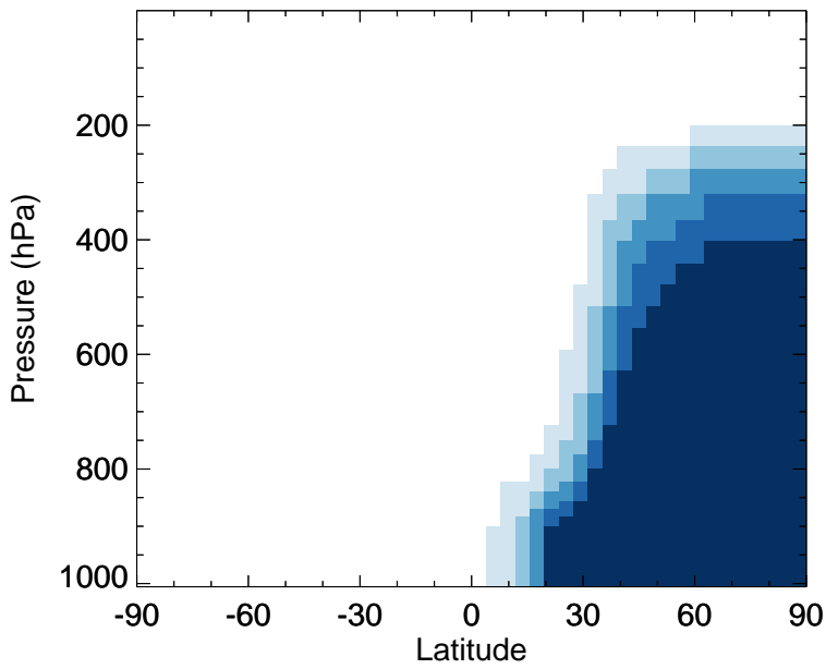
GC_12.0.0 - v11-02f-Run1 C3H8 - Zonal mean abs diff for Jan
