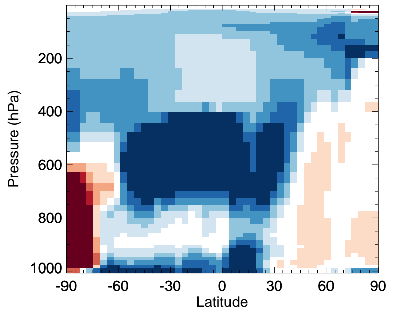
GC_12.0.0 / v11-02f-Run1 C100 - Zonal mean % diff for Jan
