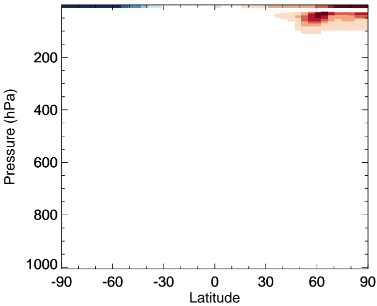
GC_12.0.0 - v11-02e-Run1 ClO - Zonal mean abs diff for Jan
