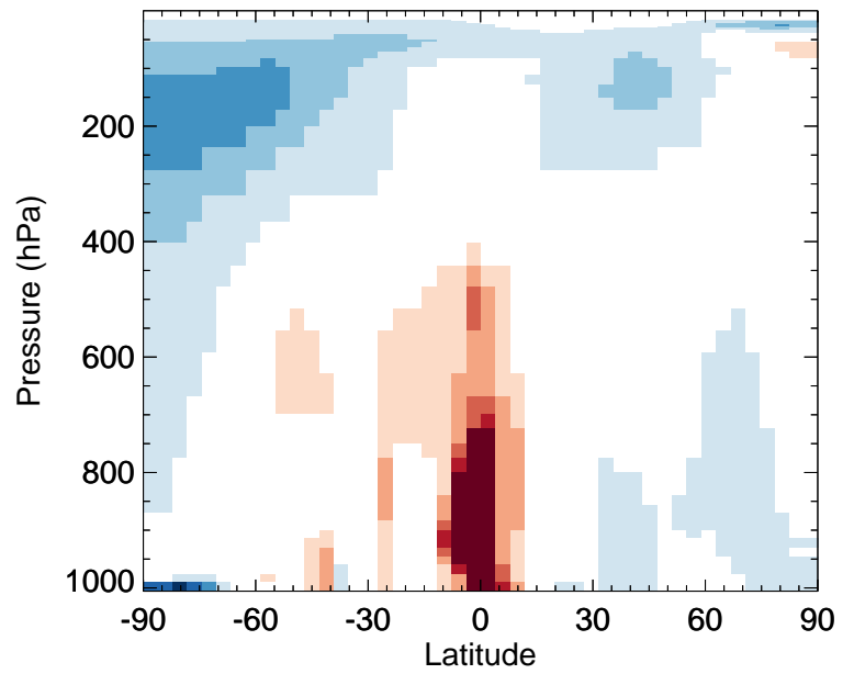
HNO2 - Zonal mean % diff for Jan
