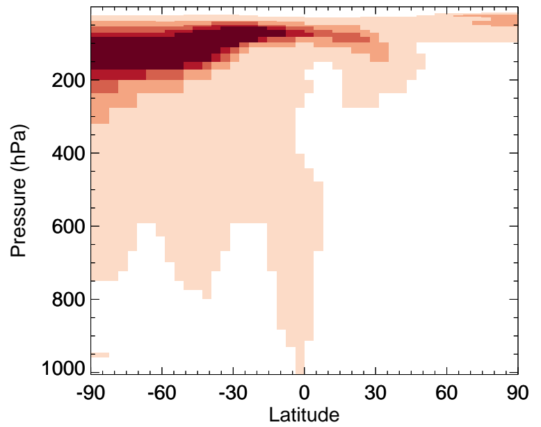
H2O2 - Zonal mean % diff for Jan
