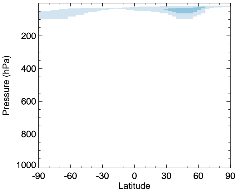
BrNO3 - Zonal mean abs diff for Jan
