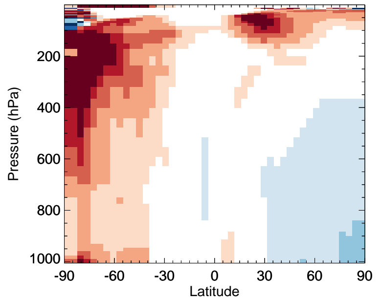
PRPE - Zonal mean % diff for Jan
