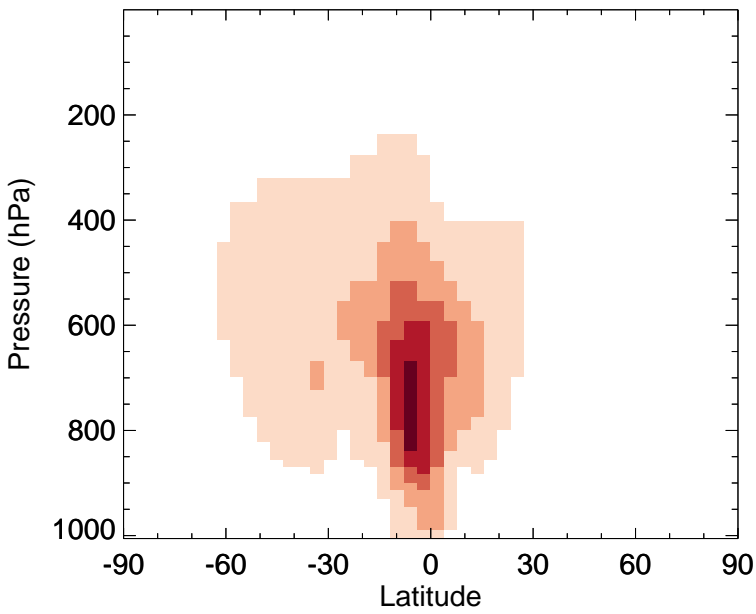
H2O2 - Zonal mean abs diff for Jan
