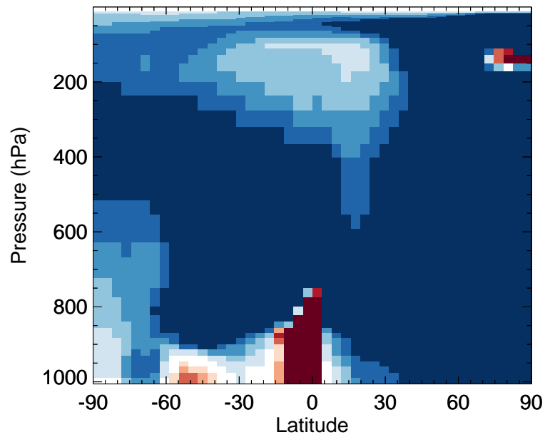
BrNO3 - Zonal mean % diff for Jan
