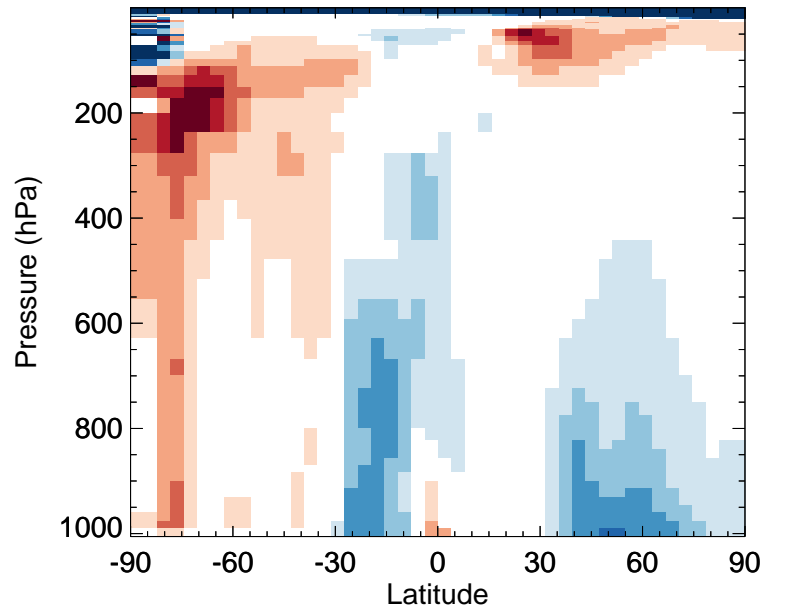
MACRN - Zonal mean % diff for Jan
