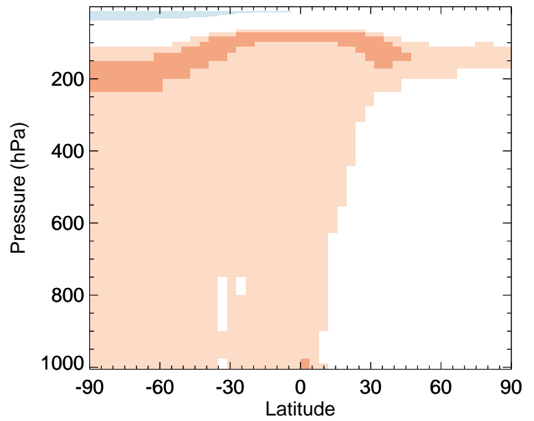
GC_12.0.0 / v11-02f-Run1 CO - Zonal mean % diff for Jan
