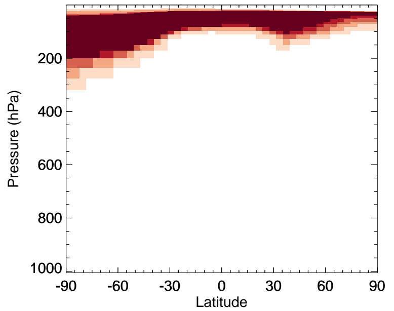
MAP - Zonal mean % diff for Jan
