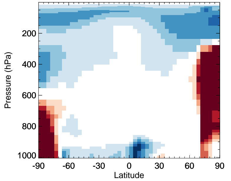
HCl - Zonal mean % diff for Jan
