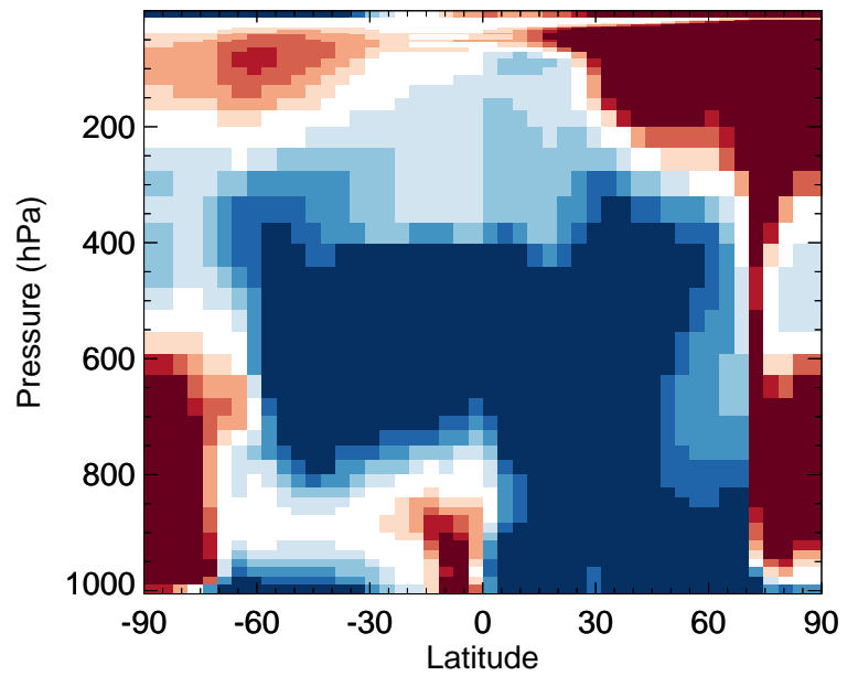
GC_12.0.0 / v11-02e-Run1 ClO - Zonal mean % diff for Jan
