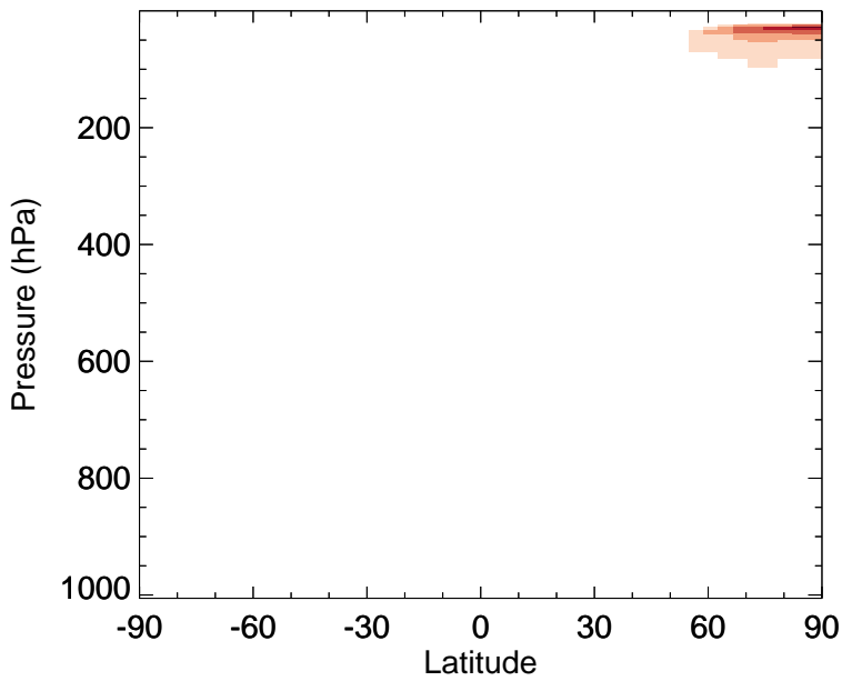
GC_12.0.0 - v11-02e-Run1 OCIO - Zonal mean abs diff for Jan
