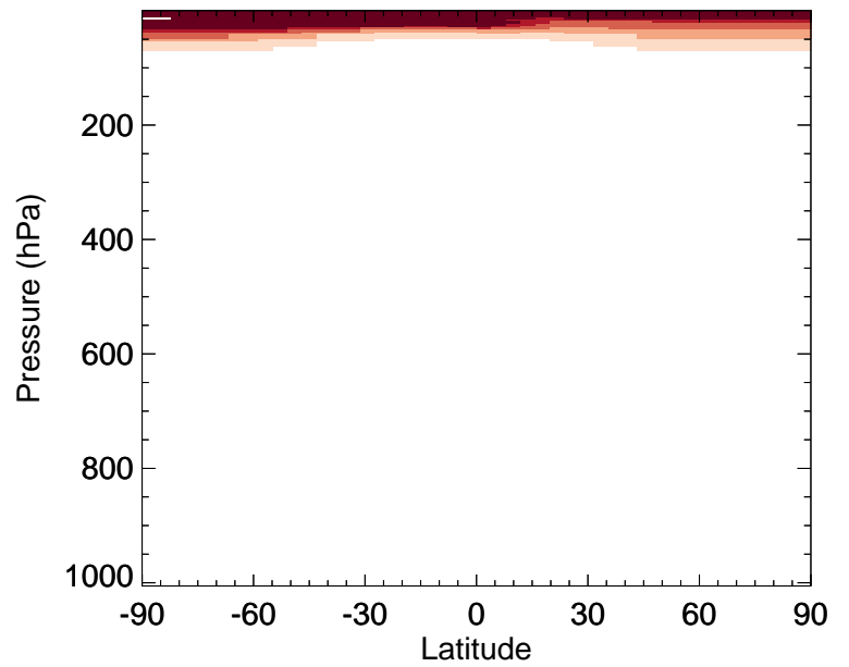
H1211 - Zonal mean % diff for Jan
