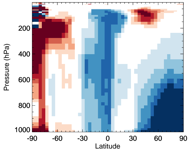
GC_12.0.0 / v11-02f-Run1 ISOP - Zonal mean % diff for Jan
