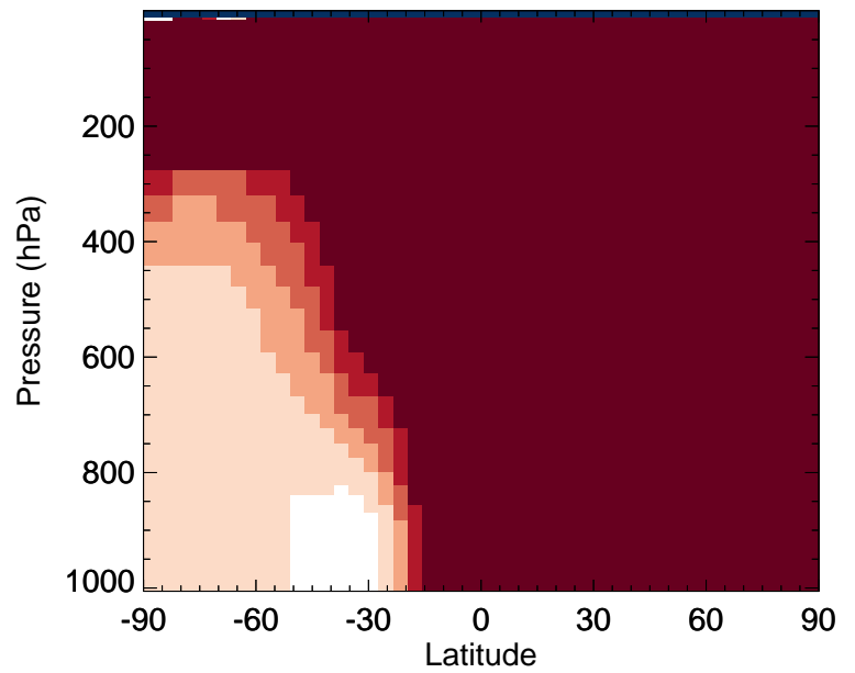
GC_12.0.0 / v11-02e-Run1 C2H6 - Zonal mean % diff for Jan
