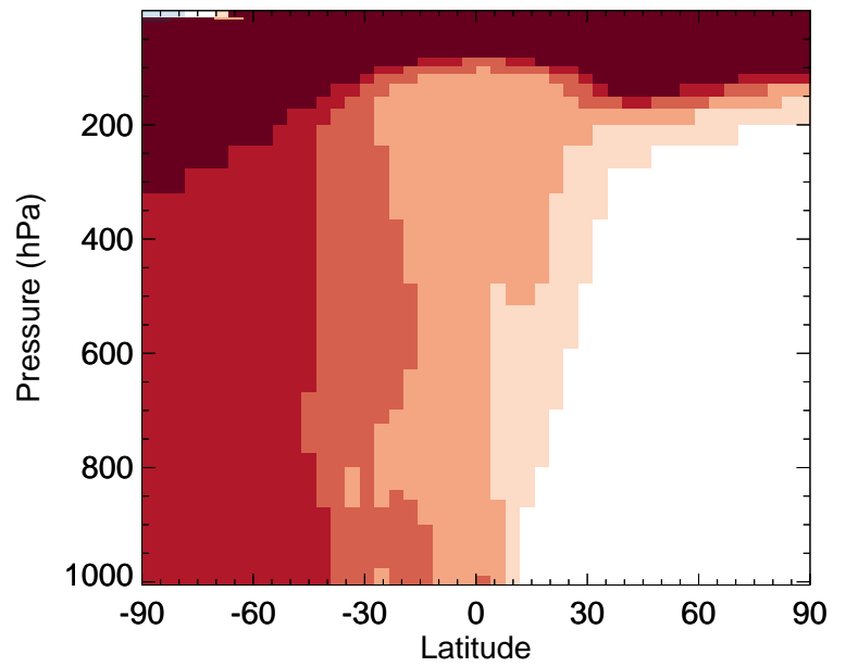
GC_12.0.0 / v11-02f-Run1 C2H6 - Zonal mean % diff for Jan
