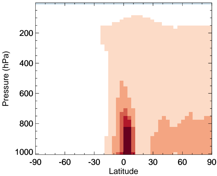
GC_12.0.0 - v11-02e-Run1 CO - Zonal mean abs diff for Jan
