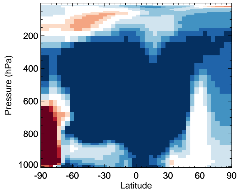
GC_12.0.0 / v11-02f-Run1 OCIO - Zonal mean % diff for Jan
