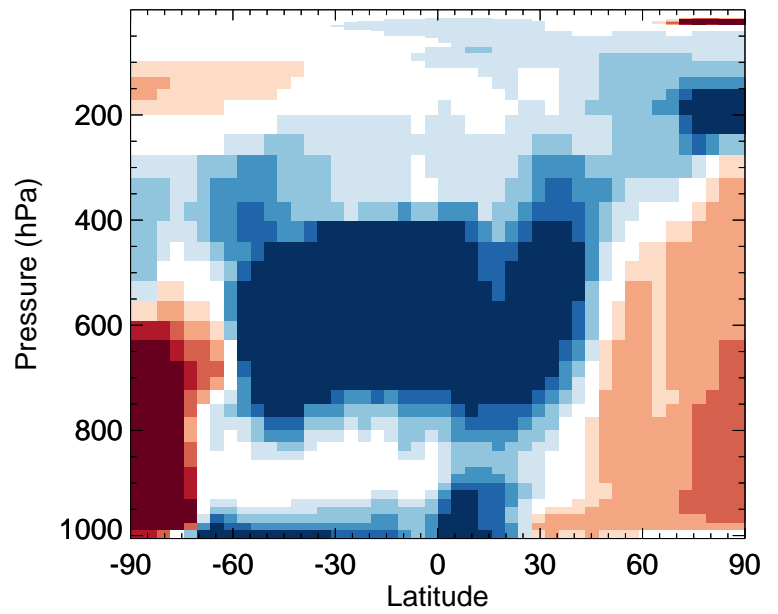
GC_12.0.0 / v11-02f-Run1 ClO - Zonal mean % diff for Jan
