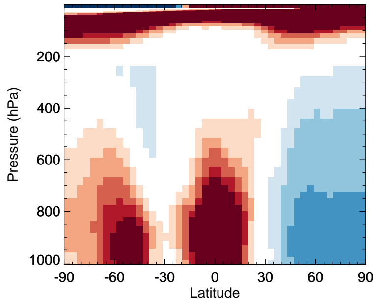
PAN - Zonal mean % diff for Jan
