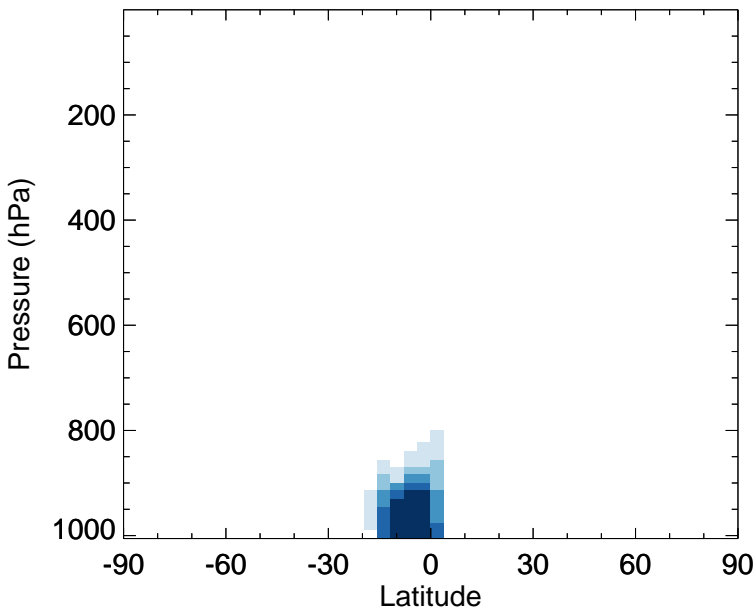
GC_12.0.0 - v11-02f-Run1 ISOP - Zonal mean abs diff for Jan
