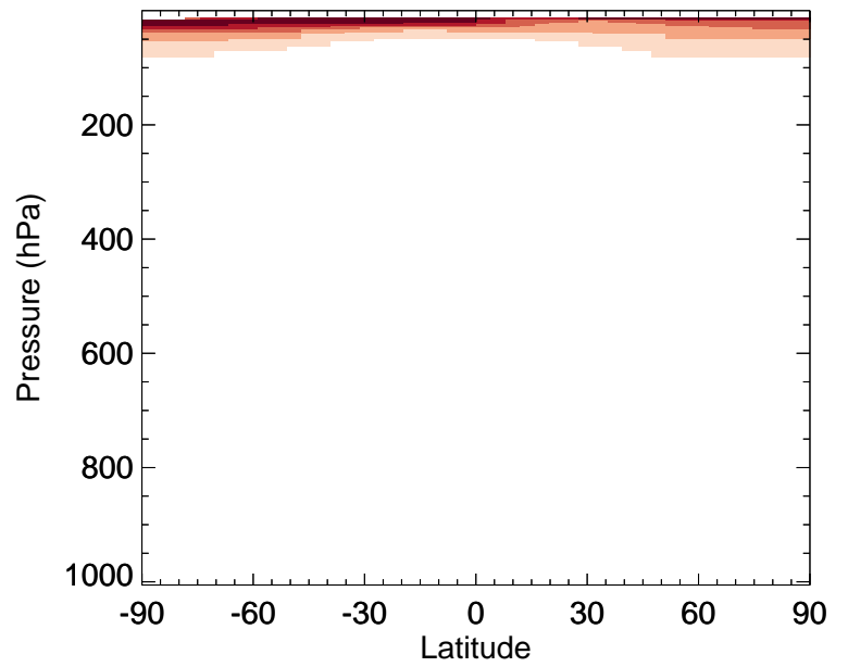
H2402 - Zonal mean % diff for Jan
