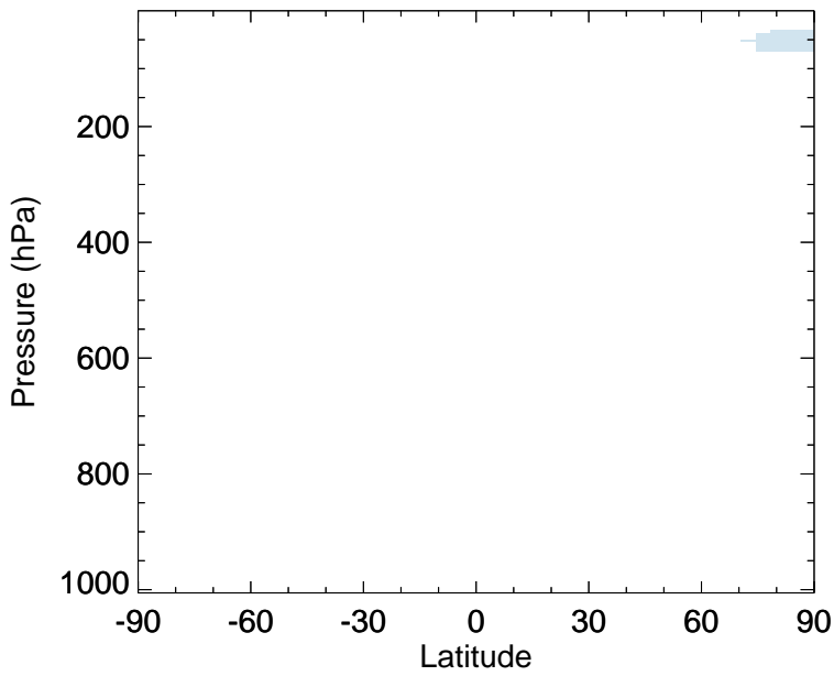
GC_12.0.0 - v11-02f-Run1 OCIO - Zonal mean abs diff for Jan
