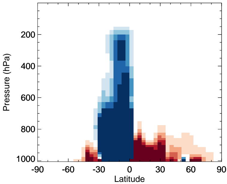
PRPE - Zonal mean abs diff for Jan
