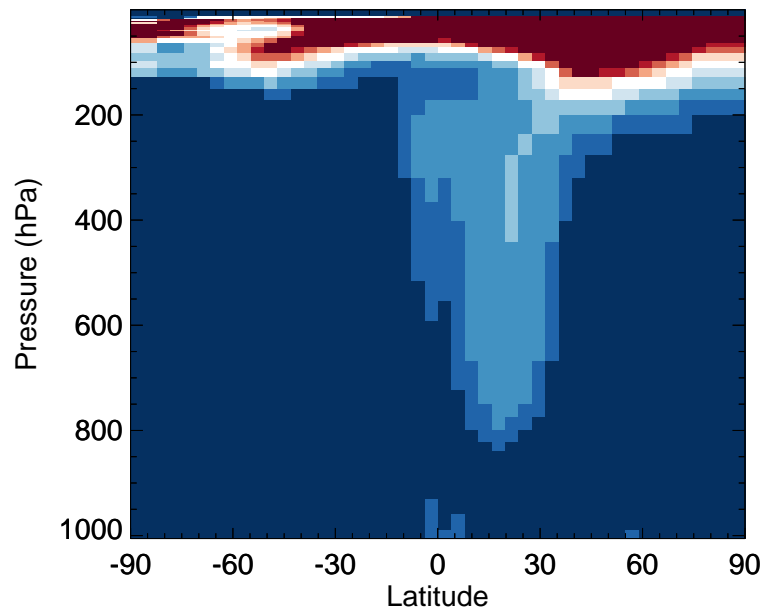
GC_12.0.0 / v11-02e-Run1 C3H8 - Zonal mean % diff for Jan
