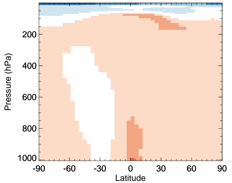
GC_12.0.0 / v11-02e-Run1 CO - Zonal mean % diff for Jan
