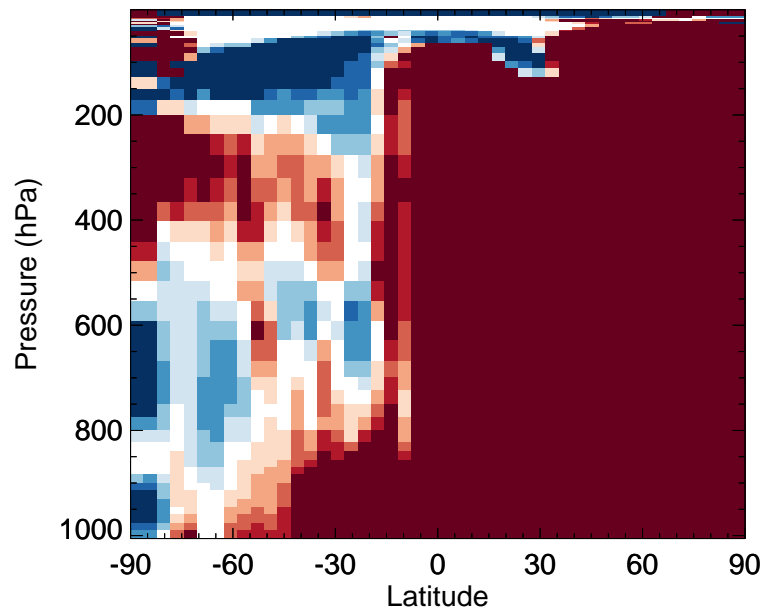
GC_12.0.0 / v11-02e-Run1 ISOP - Zonal mean % diff for Jan
