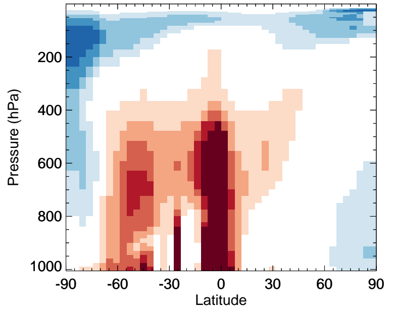
N2O5 - Zonal mean % diff for Jan
