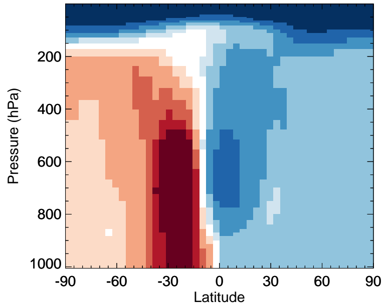
SOAIE - Zonal mean % diff for Jan
