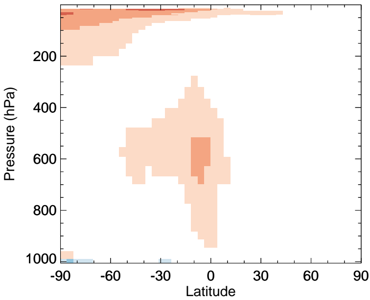
HO2 - Zonal mean abs diff for Jan
