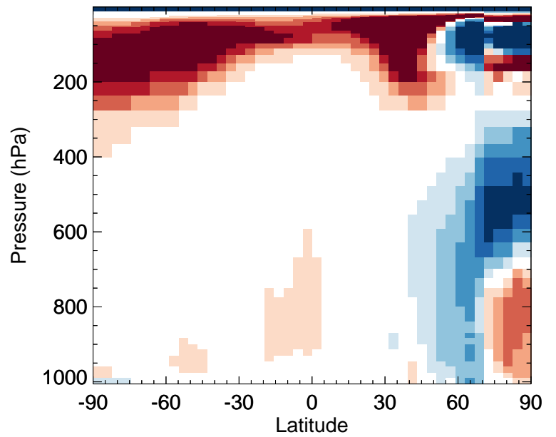
HO2 - Zonal mean % diff for Jan
