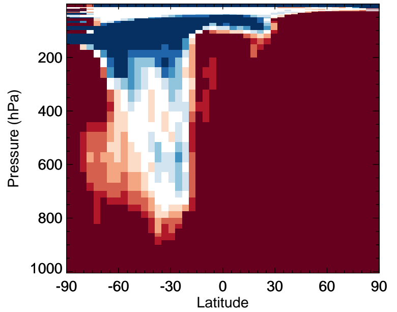
ISN1 - Zonal mean % diff for Jan
