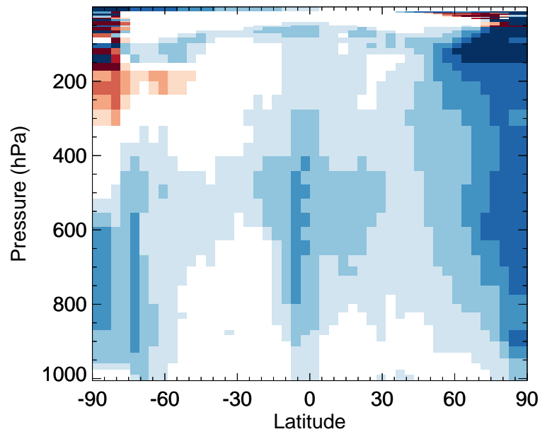
MTPA - Zonal mean % diff for Jan
