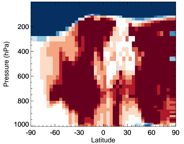
NH3 - Zonal mean % diff for Jan
