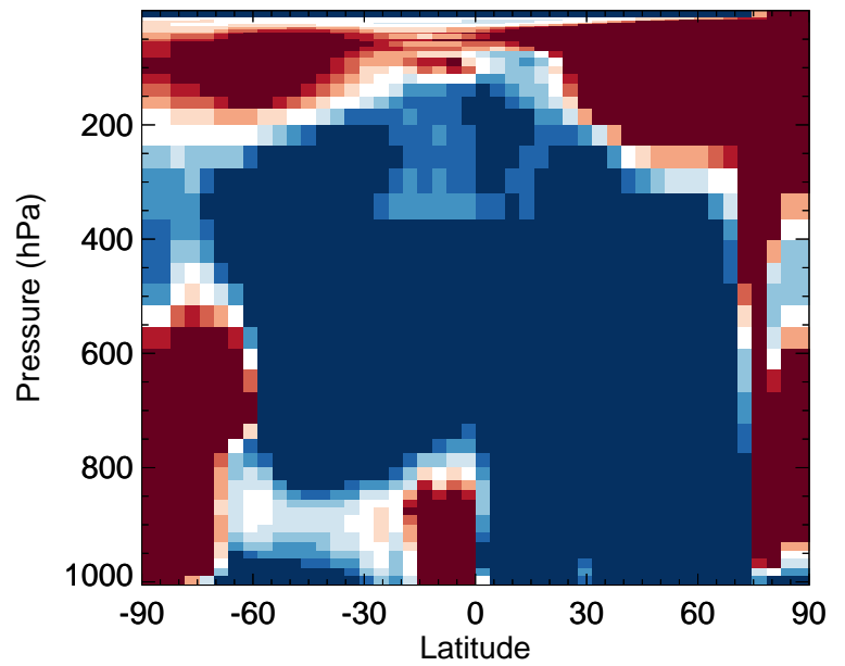
Cl2O2 - Zonal mean % diff for Jan
