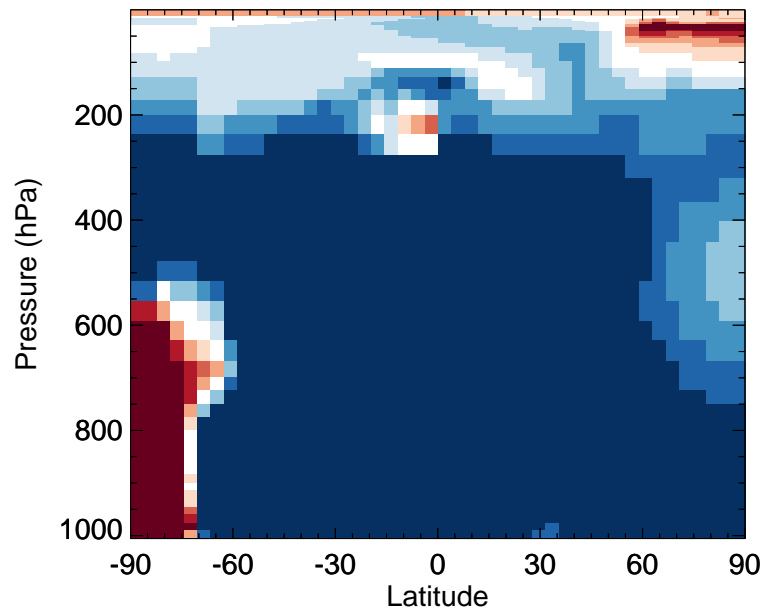
BrCl - Zonal mean % diff for Jan
