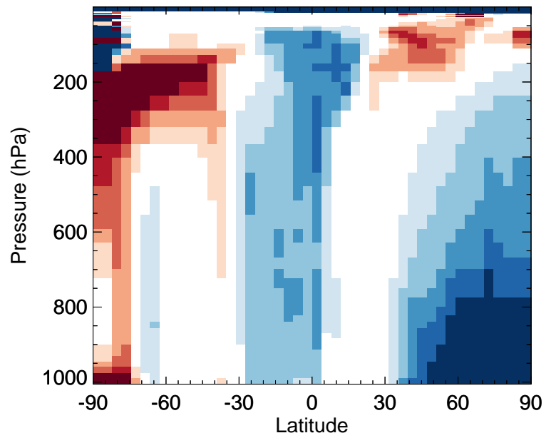
MOBA - Zonal mean % diff for Jan
