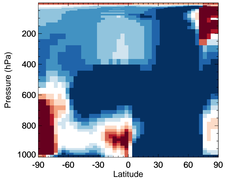
GC_12.0.0 / v11-02e-Run1 C100 - Zonal mean % diff for Jan
