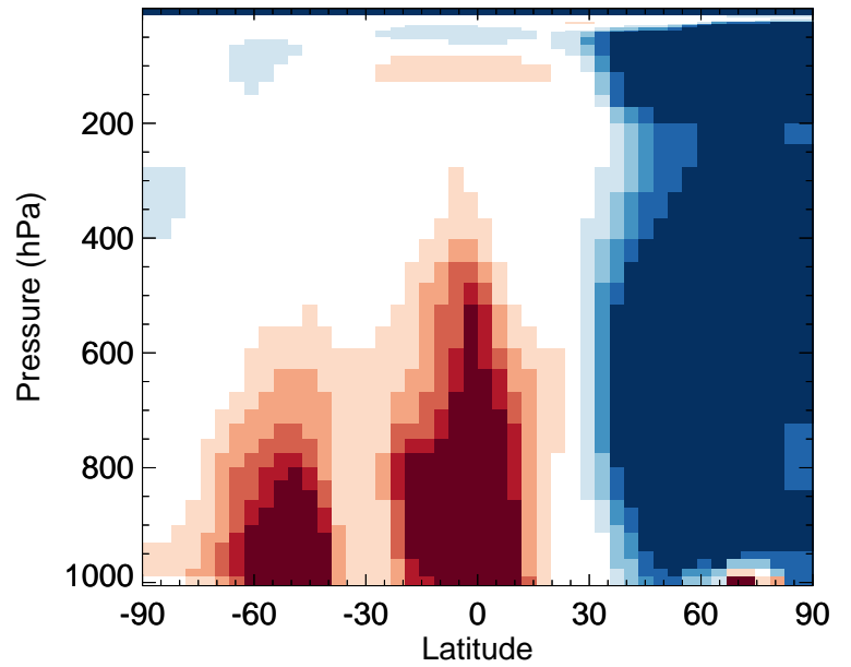
HNO 4 - Zonal mean % diff for Jan
