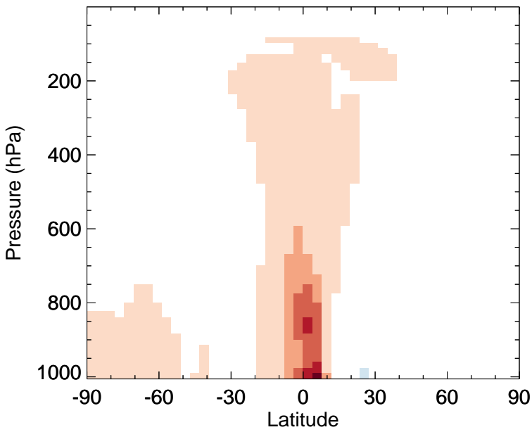
GC_12.0.0 - v11-02f-Run1 CO - Zonal mean abs diff for Jan
