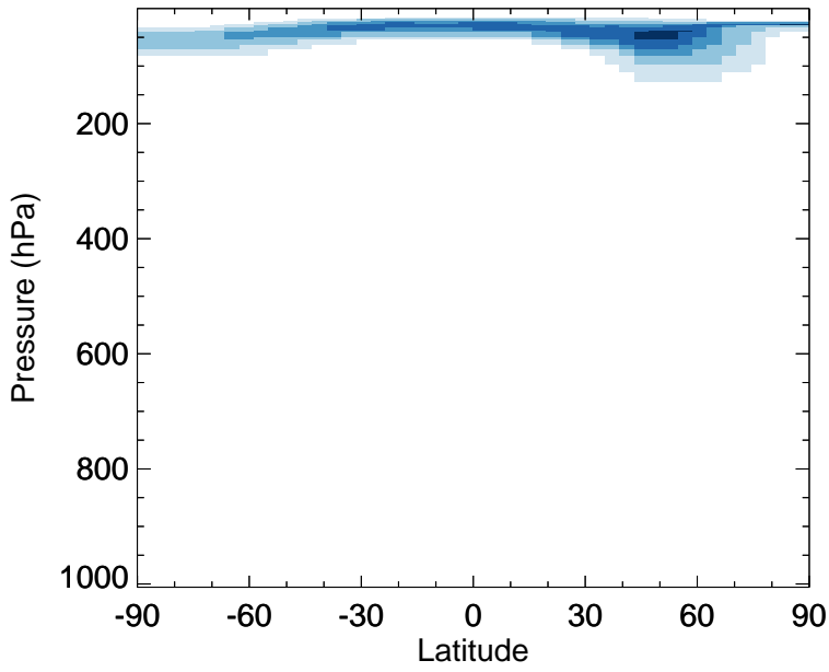
CINO3 - Zonal mean abs diff for Jan
