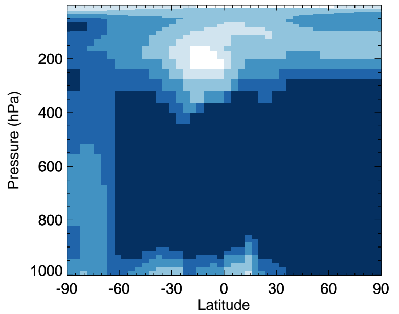
BrNO2 - Zonal mean % diff for Oct
