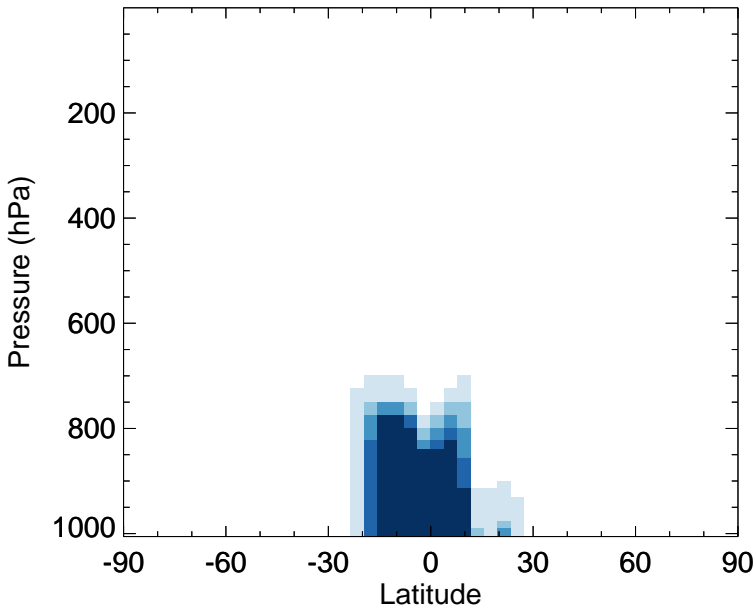
ISOP - Zonal mean abs diff for Oct
