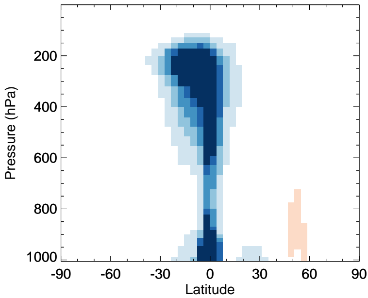
BENZ - Zonal mean abs diff for Oct
