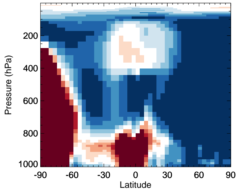
CINO3 - Zonal mean % diff for Oct
