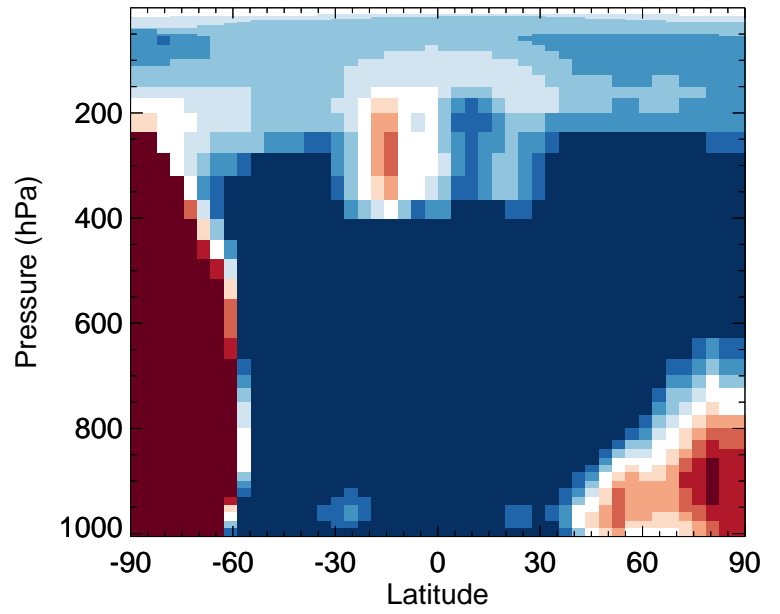
Cl2 - Zonal mean % diff for Oct
