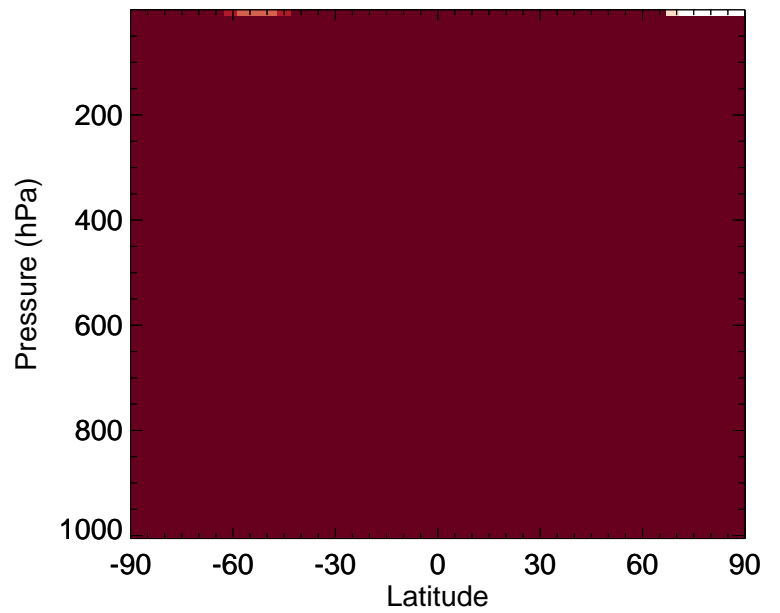
HCOOH - Zonal mean % diff for Oct
