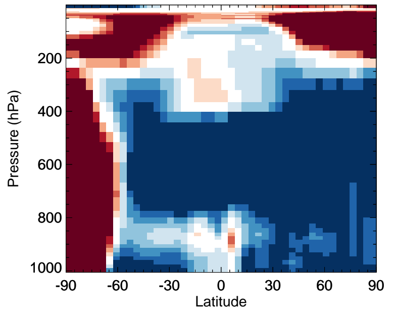
CIO - Zonal mean % diff for Oct
