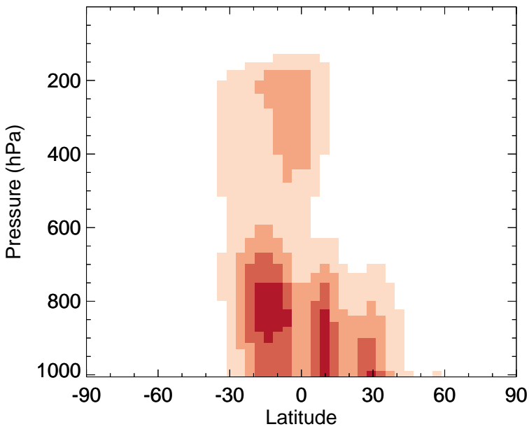
HCOOH - Zonal mean abs diff for Oct
