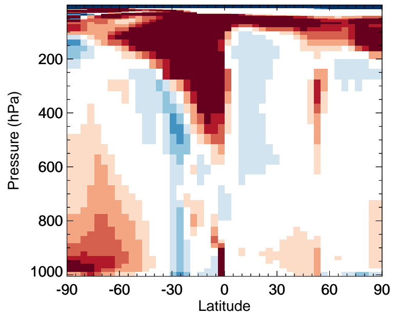
LVOC - Zonal mean % diff for Oct
