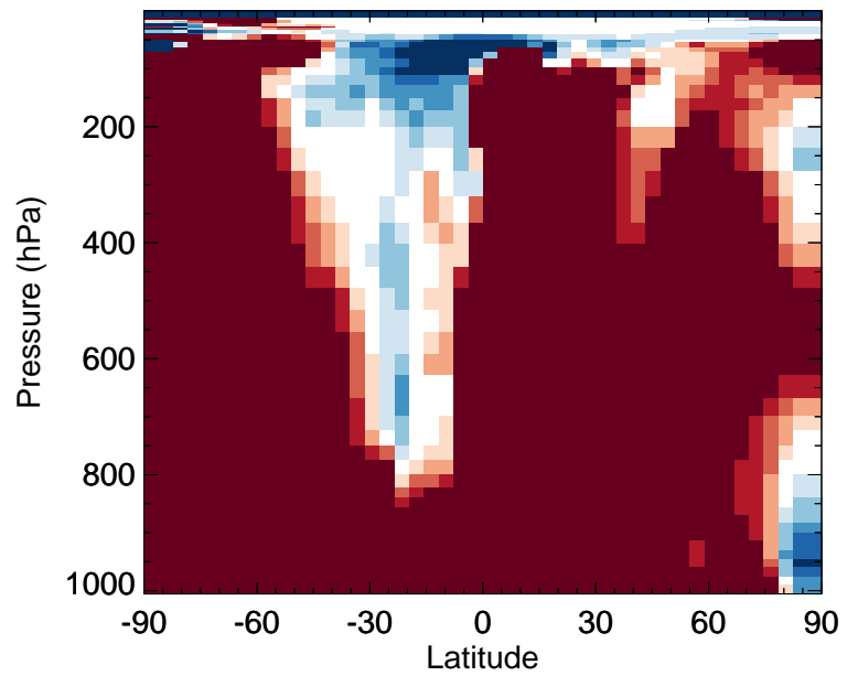
ISN1 - Zonal mean % diff for Oct
