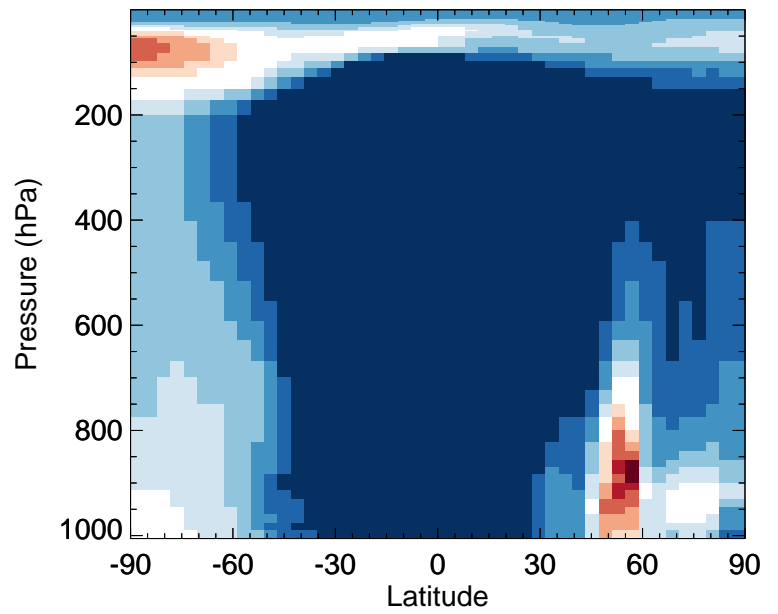
ASOA3 - Zonal mean % diff for Oct
