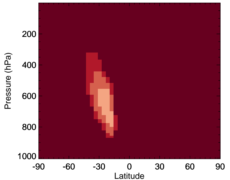
INDIOL - Zonal mean % diff for Oct
