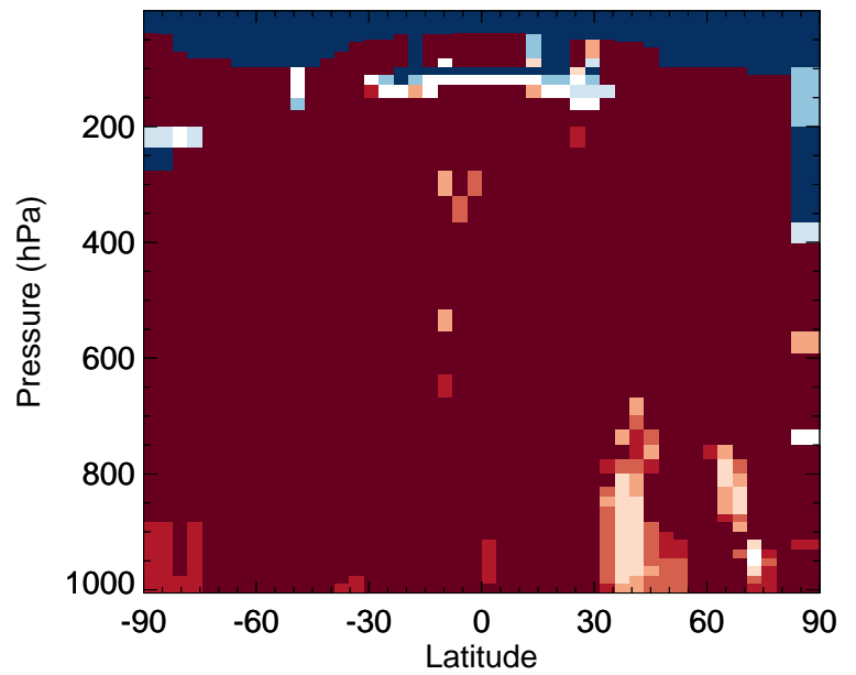
NIT - Zonal mean % diff for Oct
