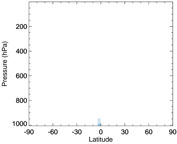
CH2O - Zonal mean abs diff for Oct
