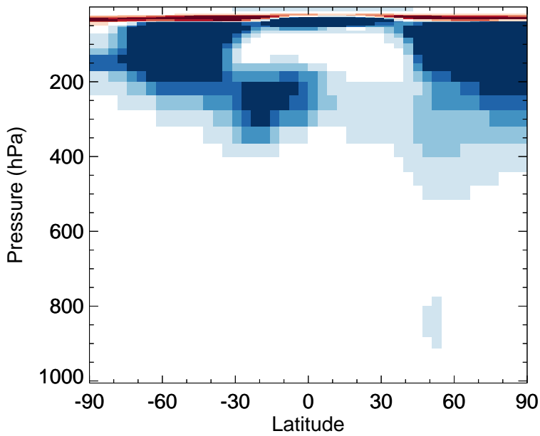
HNO4 - Zonal mean abs diff for Oct
