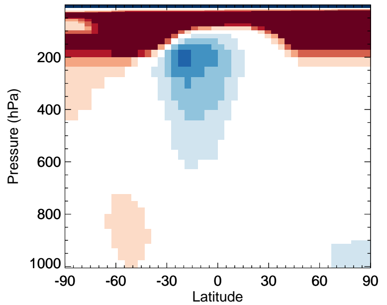
H2O2 - Zonal mean % diff for Oct
