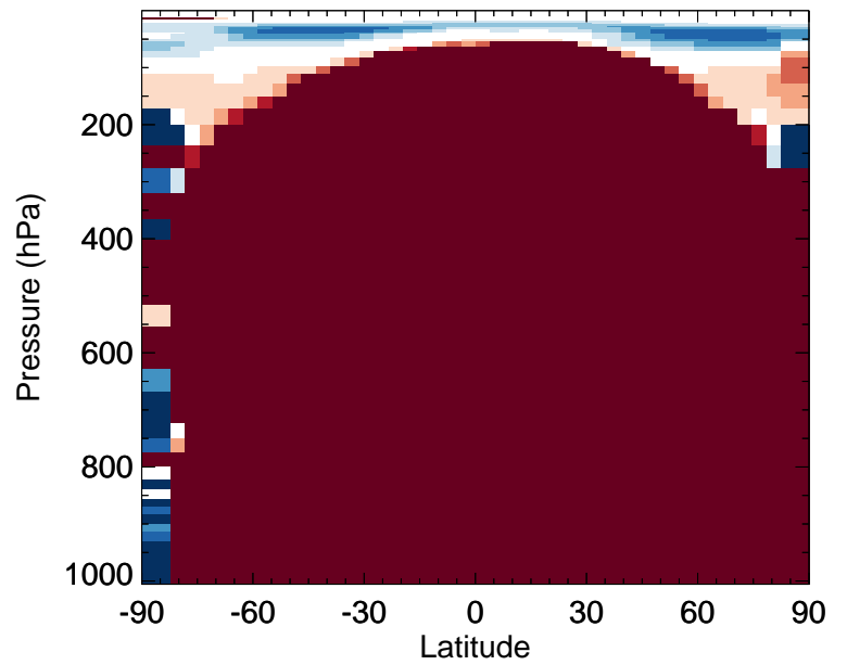
MTPO - Zonal mean % diff for Oct
