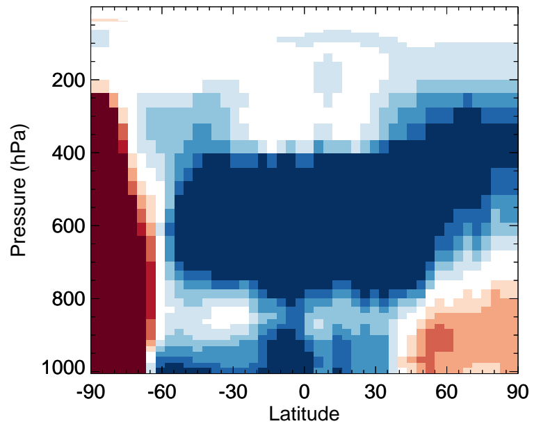
HOCl - Zonal mean % diff for Oct
