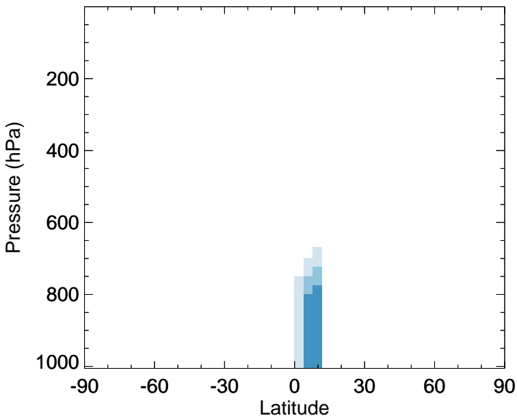
SOAIE - Zonal mean abs diff for Oct
