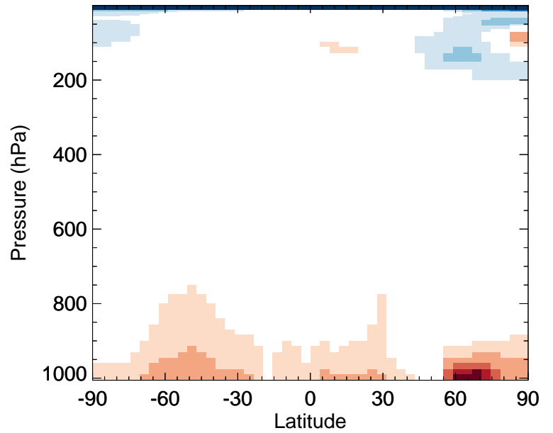
CH2O - Zonal mean % diff for Oct
