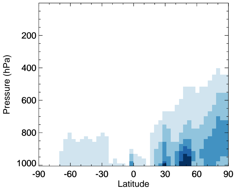
GC_12.0.0 - v11-02e-Run1 C3H8 - Zonal mean abs diff for Oct
