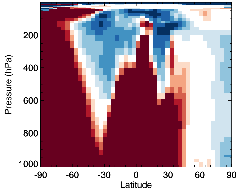
PROPNN - Zonal mean % diff for Oct
