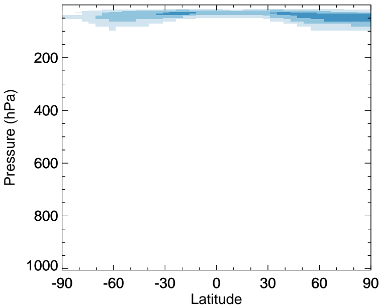
CINO3 - Zonal mean abs diff for Oct
