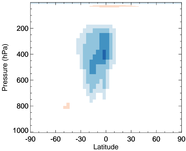
H2O2 - Zonal mean abs diff for Oct
