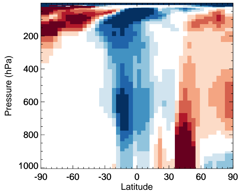
DMS - Zonal mean % diff for Oct
