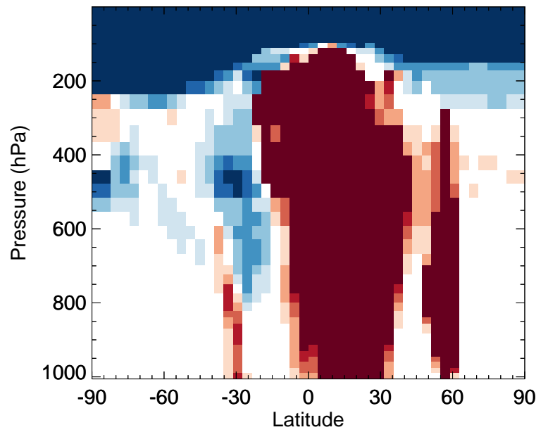
NH3 - Zonal mean % diff for Oct
