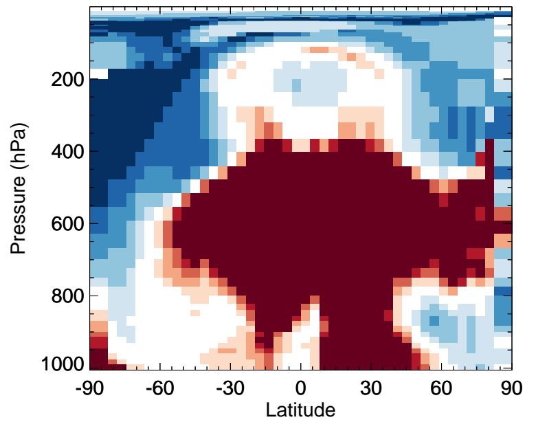
HBr - Zonal mean % diff for Oct
