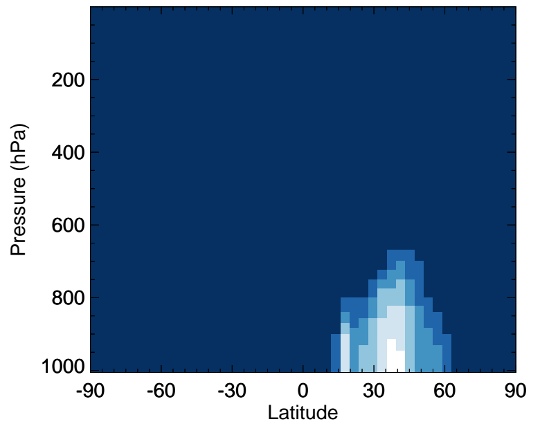
SOAIE - Zonal mean % diff for Oct
