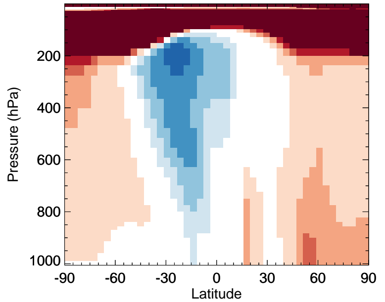
MAP - Zonal mean % diff for Oct
