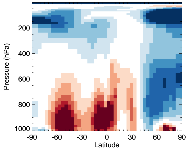
HNO4 - Zonal mean % diff for Oct
