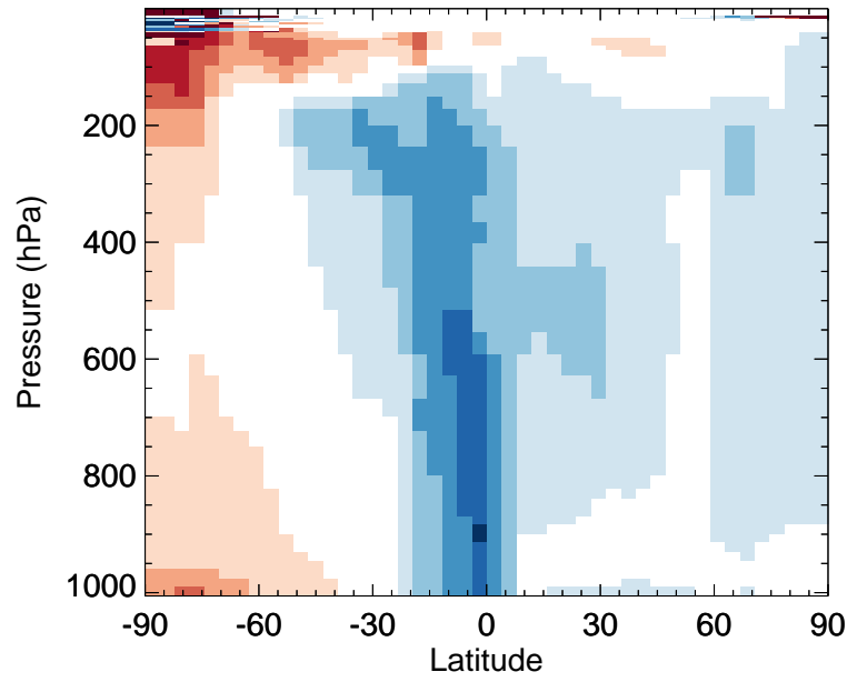
MVK - Zonal mean % diff for Oct
