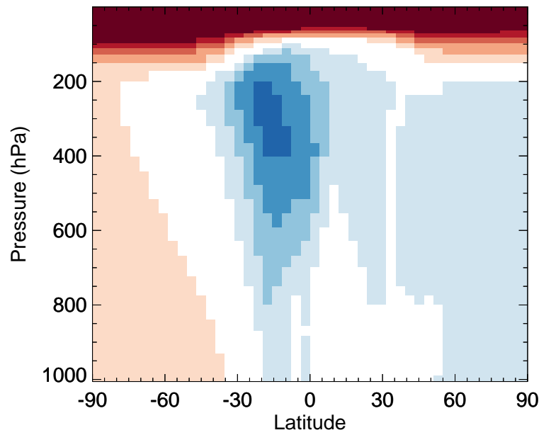
C2H6 - Zonal mean % diff for Oct
