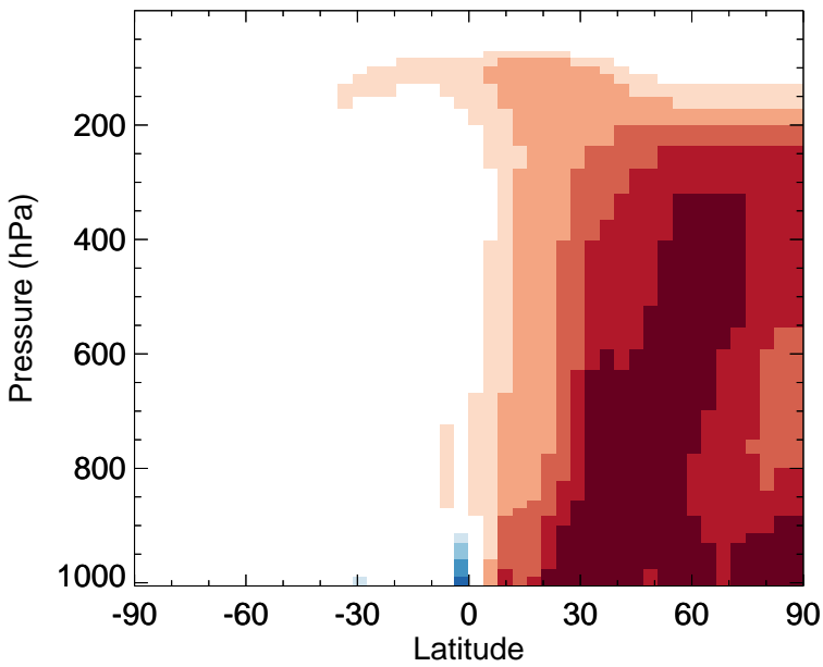
C2H6 - Zonal mean abs diff for Oct
