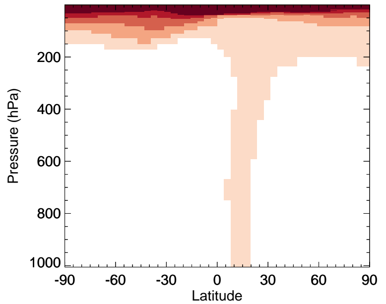
ACET - Zonal mean % diff for Oct
