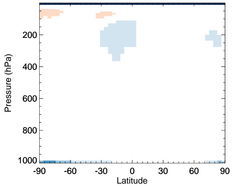
HO2 - Zonal mean % diff for Oct
