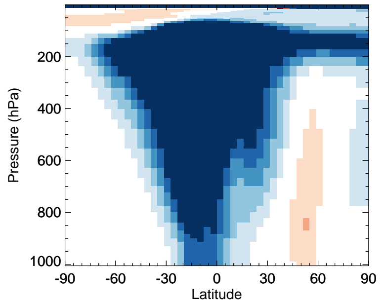
BENZ - Zonal mean % diff for Oct
