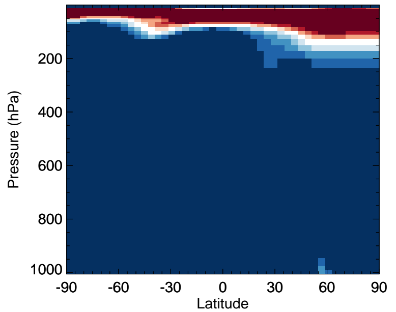
GC_12.0.0 / v11-02e-Run1 C3H8 - Zonal mean % diff for Oct
