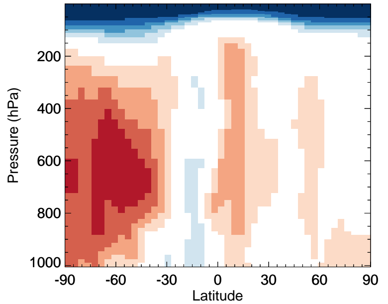
NH4 - Zonal mean % diff for Oct
