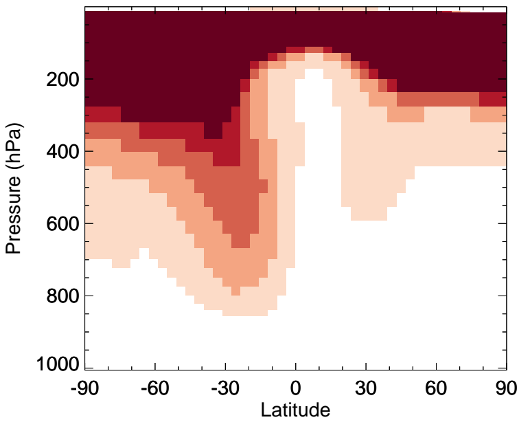
N2O - Zonal mean abs diff for Oct
