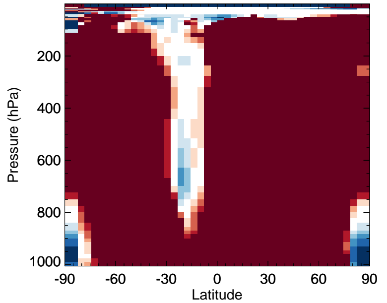
ISOP - Zonal mean % diff for Oct
