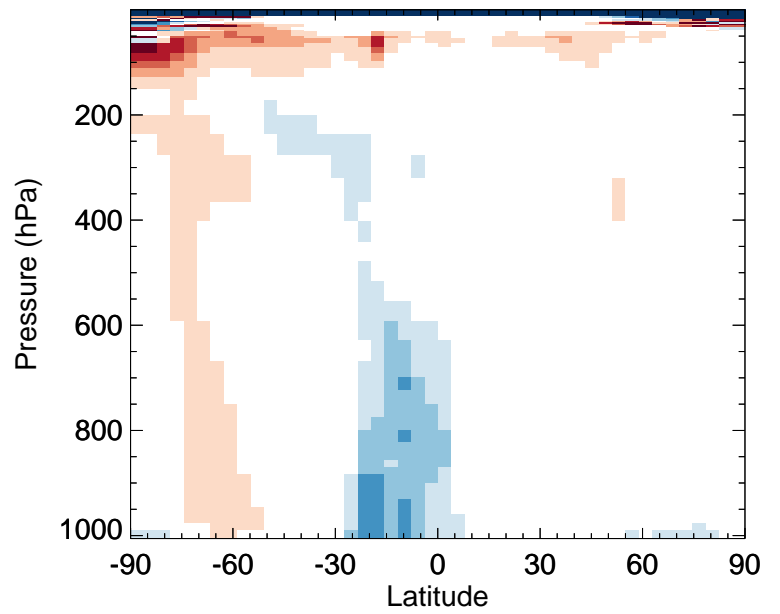
MACRN - Zonal mean % diff for Oct
