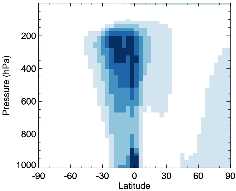
CO - Zonal mean abs diff for Oct
