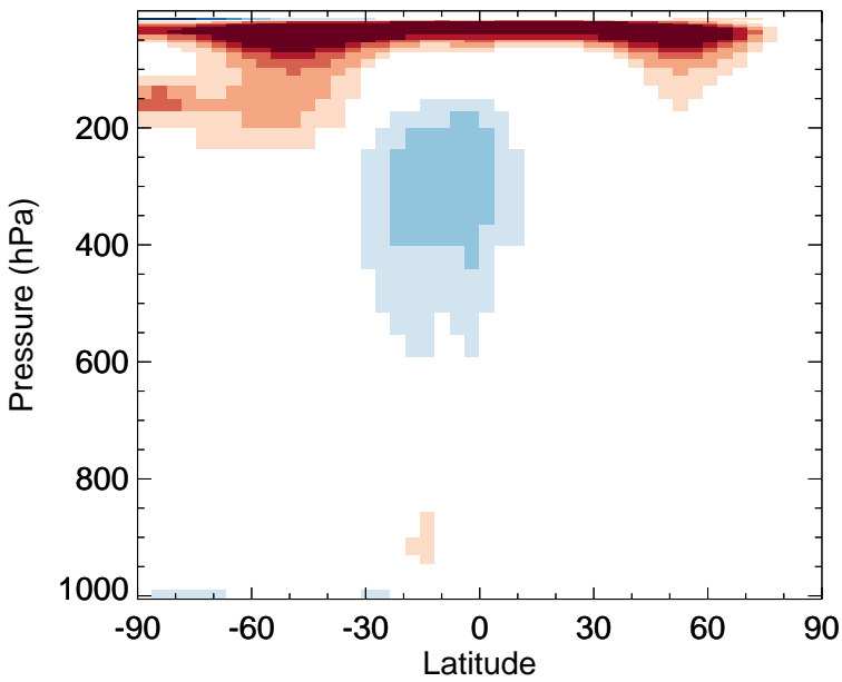
HO2 - Zonal mean abs diff for Oct
