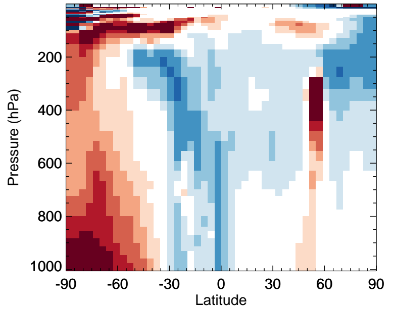
RIPB - Zonal mean % diff for Oct
