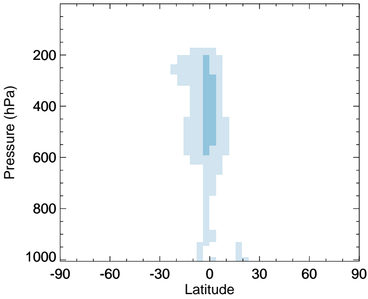
MAP - Zonal mean abs diff for Oct
