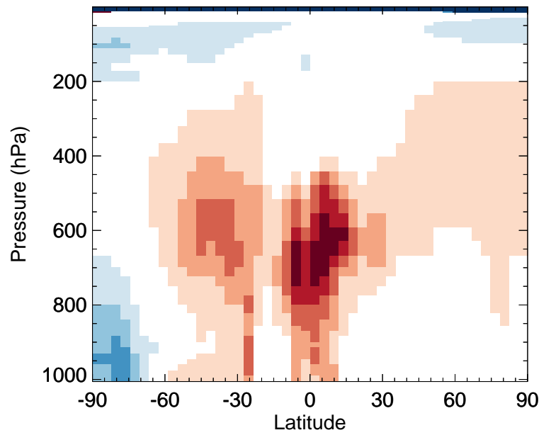
CINO2 - Zonal mean % diff for Oct
