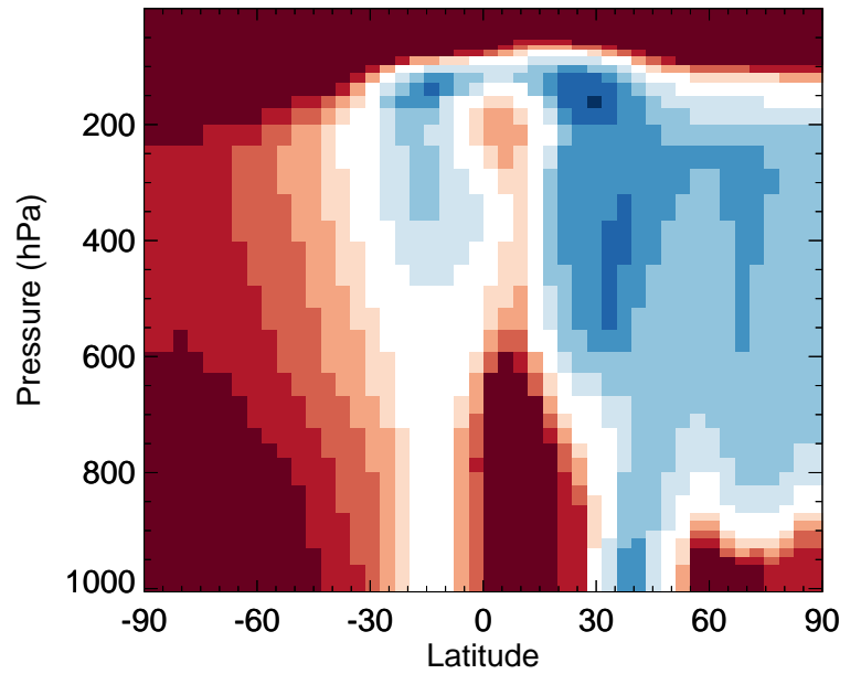
ASOG3 - Zonal mean % diff for Oct
