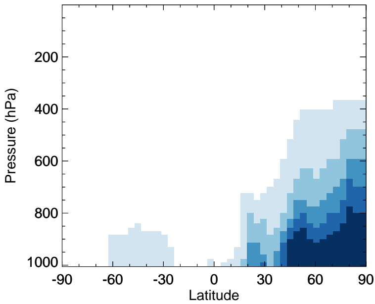
GC_12.0.0 - v11-02f-Run1 C3H8 - Zonal mean abs diff for Oct
