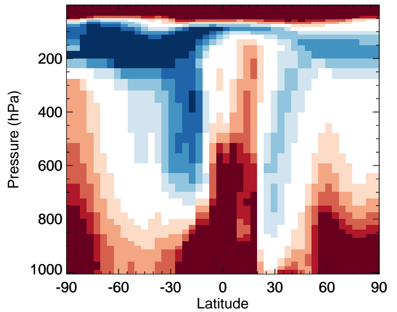
RCHO - Zonal mean % diff for Oct
