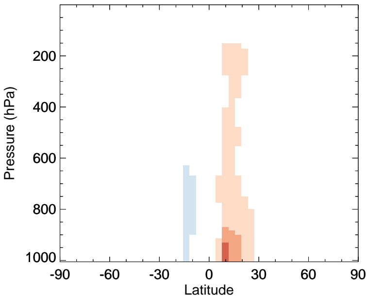
ACET - Zonal mean abs diff for Oct
