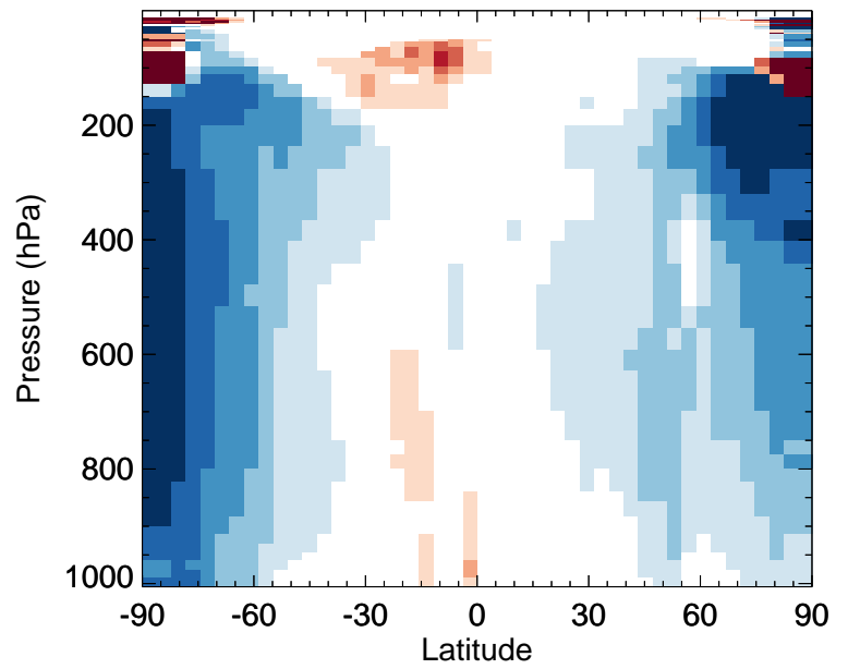
MONITU - Zonal mean % diff for Oct
