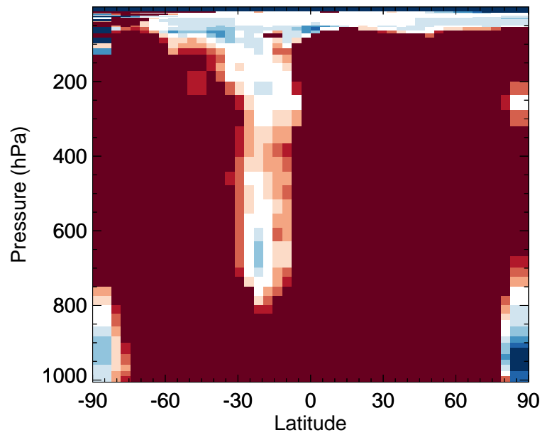
ISOPND - Zonal mean % diff for Oct
