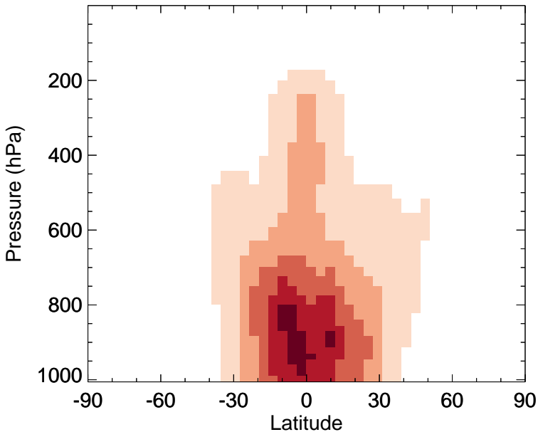
ACTA - Zonal mean abs diff for Oct
