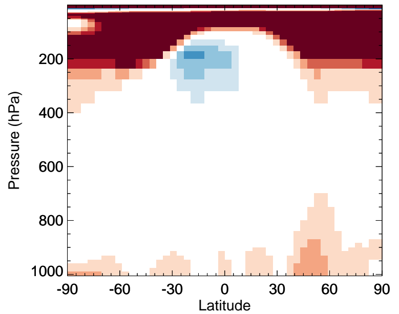
MP - Zonal mean % diff for Oct
