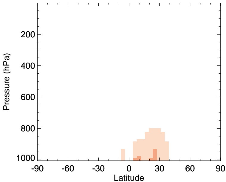
INDIOL - Zonal mean abs diff for Oct
