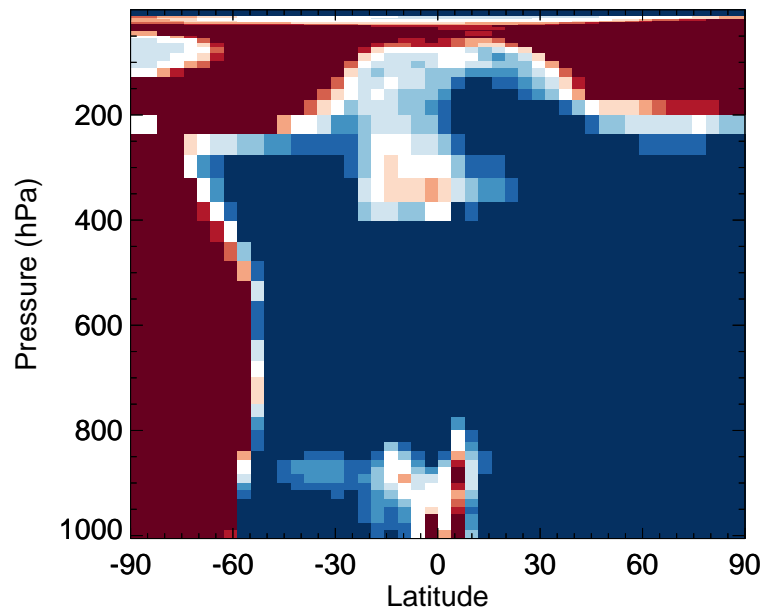
Cl2O2 - Zonal mean % diff for Oct
