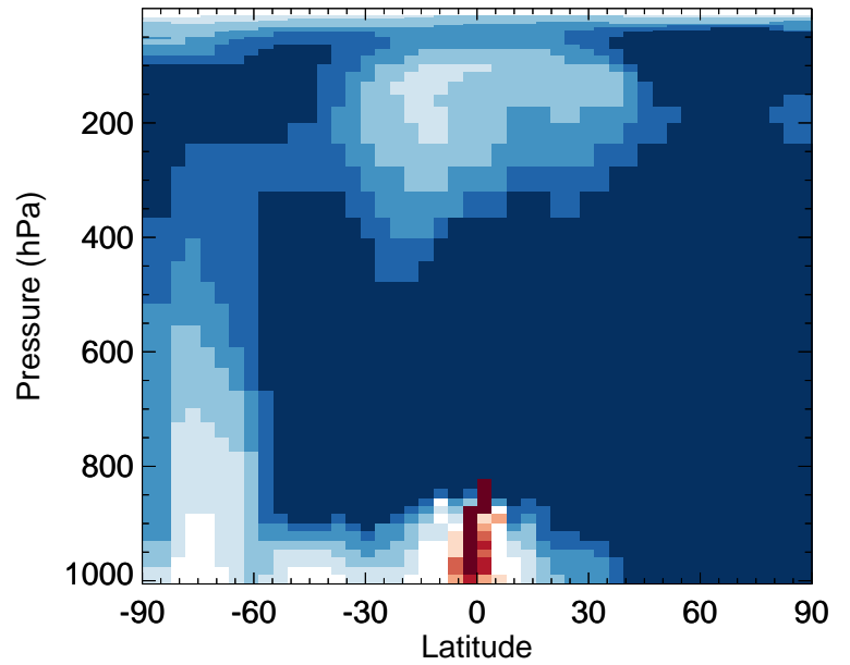
BrNO3 - Zonal mean % diff for Oct
