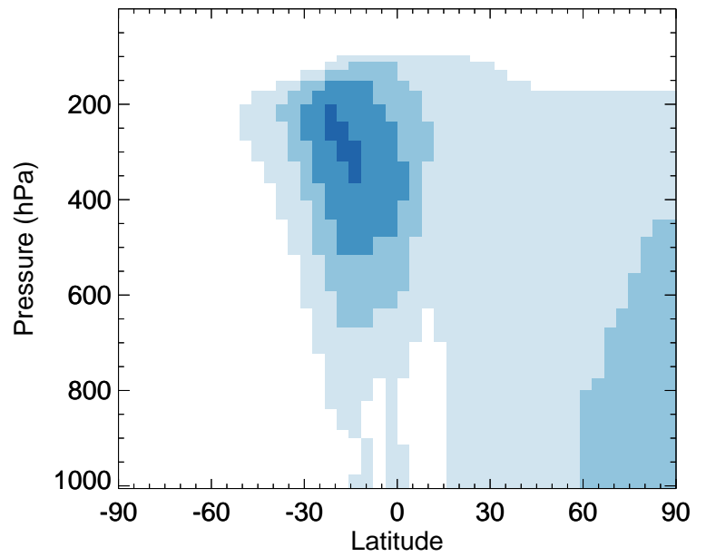
CO - Zonal mean % diff for Oct
