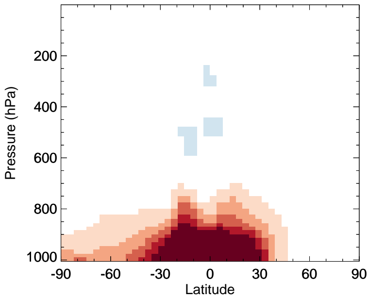
MP - Zonal mean abs diff for Oct
