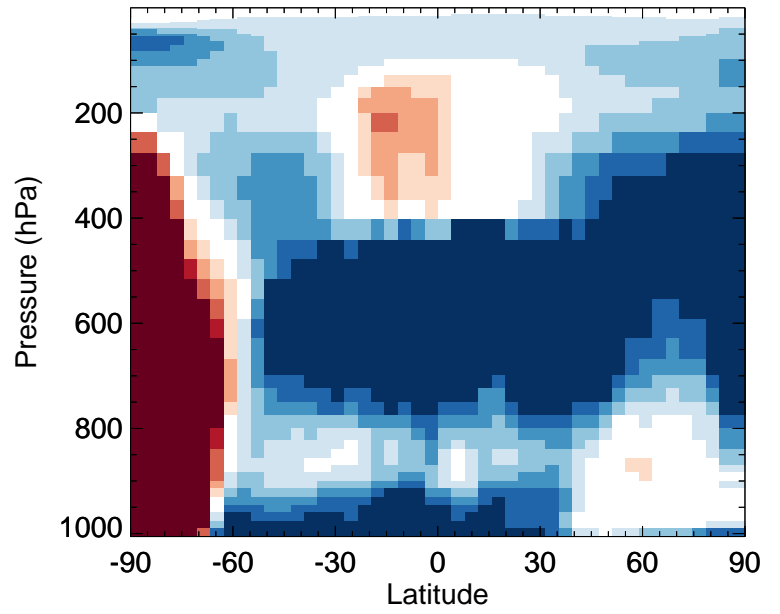
CIOO - Zonal mean % diff for Oct
