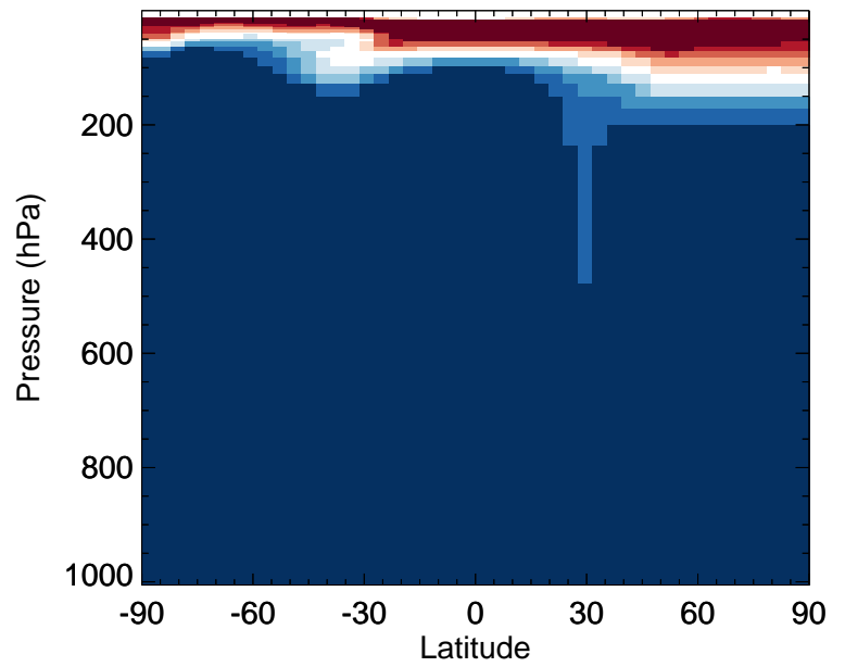
GC_12.0.0 / v11-02f-Run1 C3H8 - Zonal mean % diff for Oct
