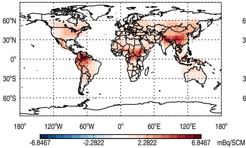
Abs Diff @ Surface - Rn222
