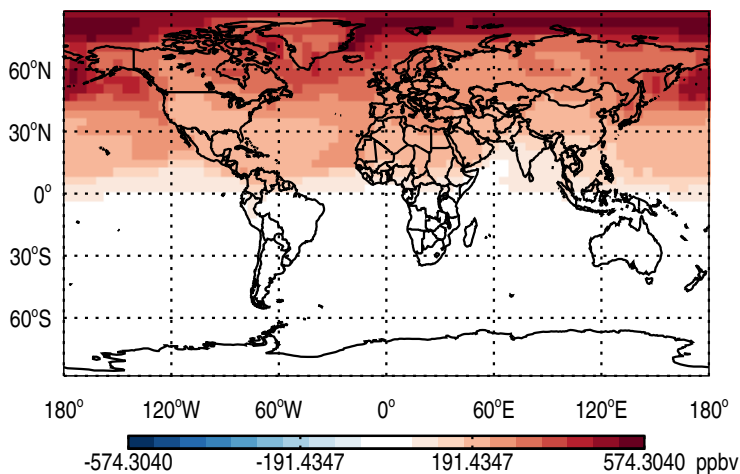
Abs Diff @ Surface - NHEmis90dayTracer
