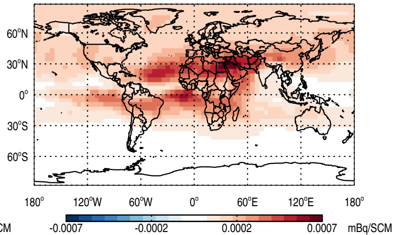
Abs Diff @ 500 hPa - Pb210
