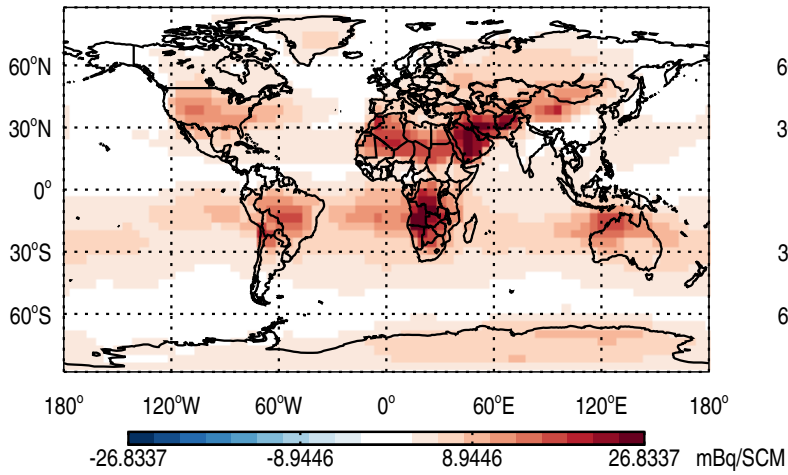
Abs Diff @ Surface - Be10Strat
