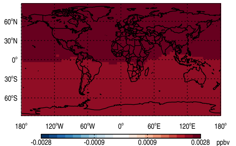
Abs Diff @ 500 hPa - SF6Tracer
