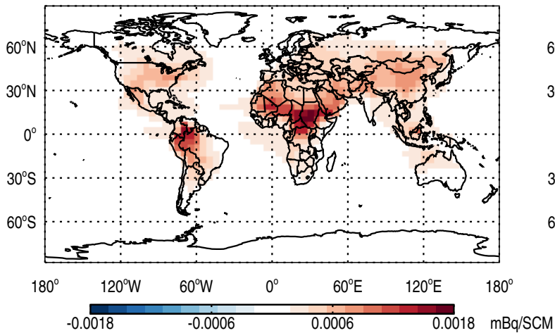
Abs Diff @ Surface - Pb210
