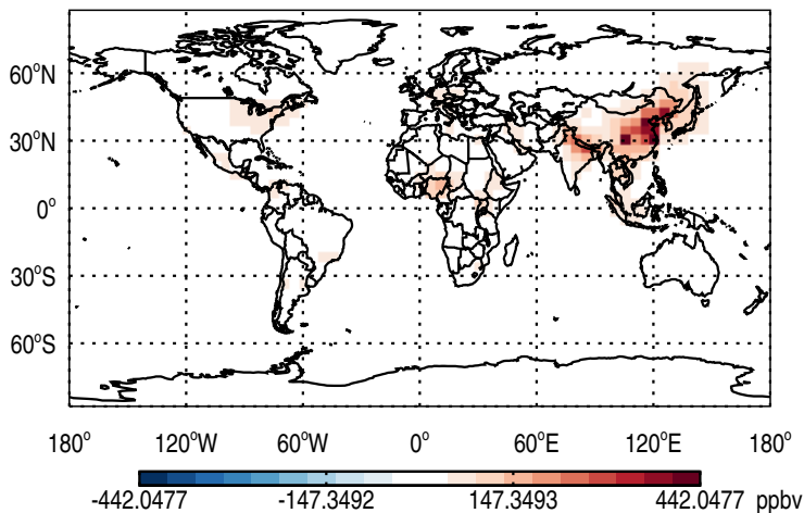
Abs Diff @ Surface - COAnthroEmis50dayTracer
