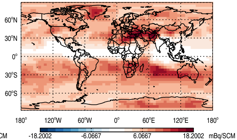
Abs Diff @ 500 hPa - Be7Strat
