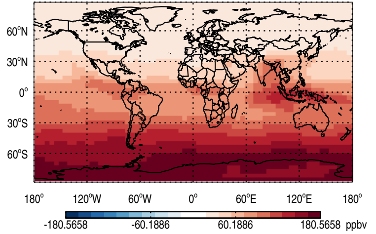
Abs Diff @ 500 hPa - SHEmis90dayTracer
