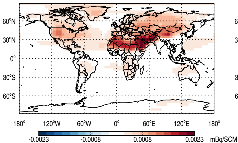
Abs Diff @ Surface - Pb210Strat
