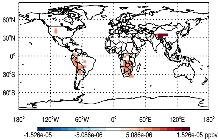
Abs Diff @ Surface - PassiveTracer
