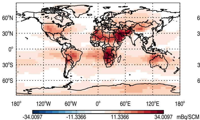
Abs Diff @ Surface - Be10
