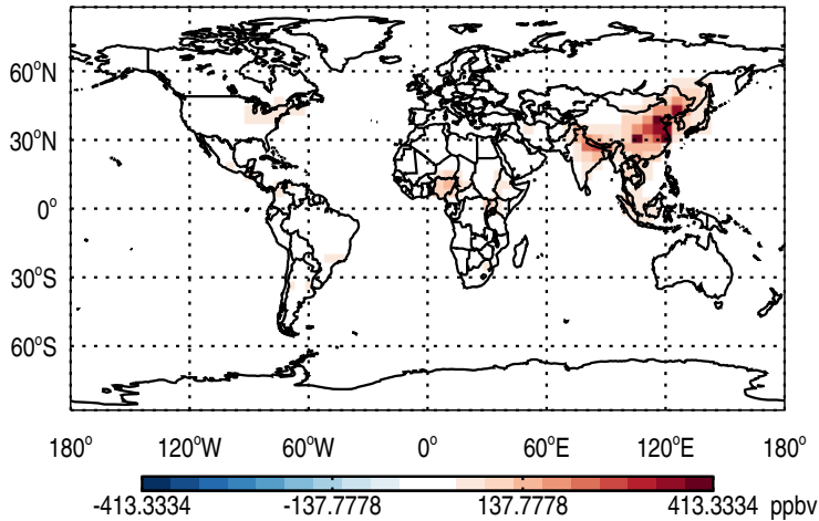
Abs Diff @ Surface - COAnthroEmis25dayTracer
