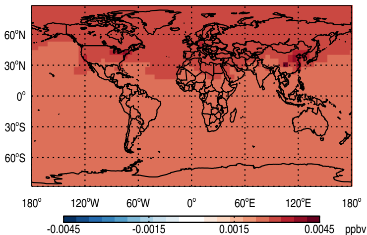
Abs Diff @ Surface - SF6Tracer
