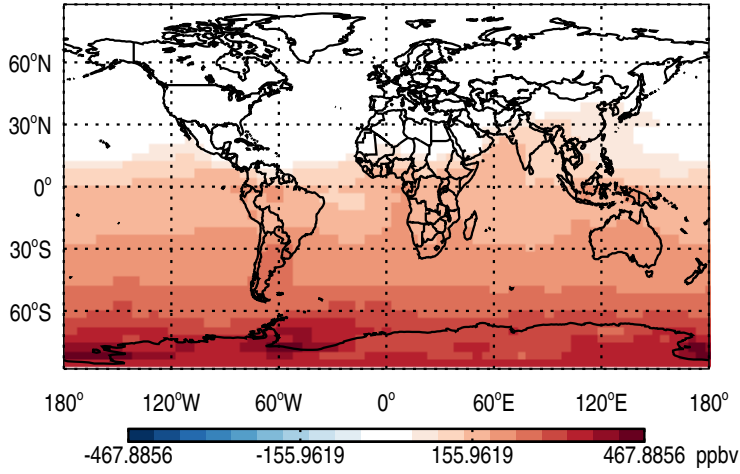
Abs Diff @ Surface - SHEmis90dayTracer
