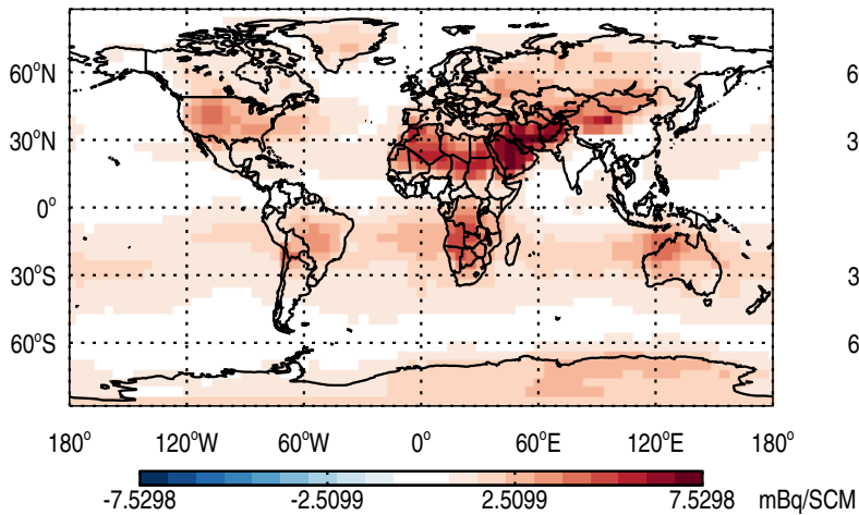
Abs Diff @ Surface - Be7Strat
