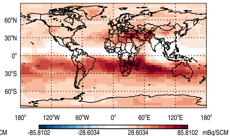
Abs Diff @ 500 hPa - Be10
