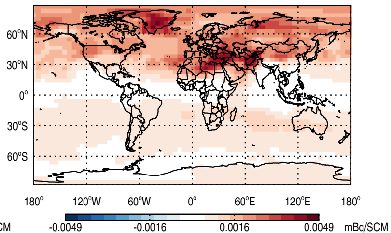
Abs Diff @ 500 hPa - Pb210Strat
