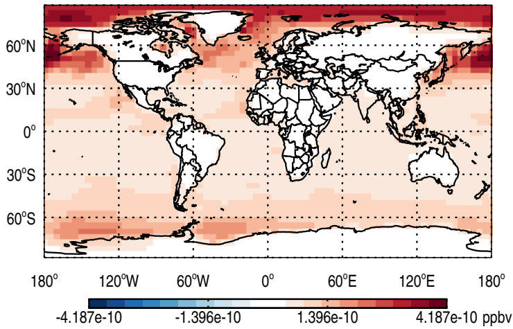
Abs Diff @ Surface - CH3ITracer
