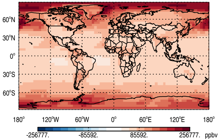
Abs Diff @ Surface - COUniformEmis25dayTracer
