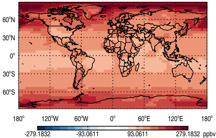
Abs Diff @ Surface - GlobEmis90dayTracer
