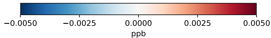
Fractional Difference (Dev-Ref)/Ref, Fixed Range
