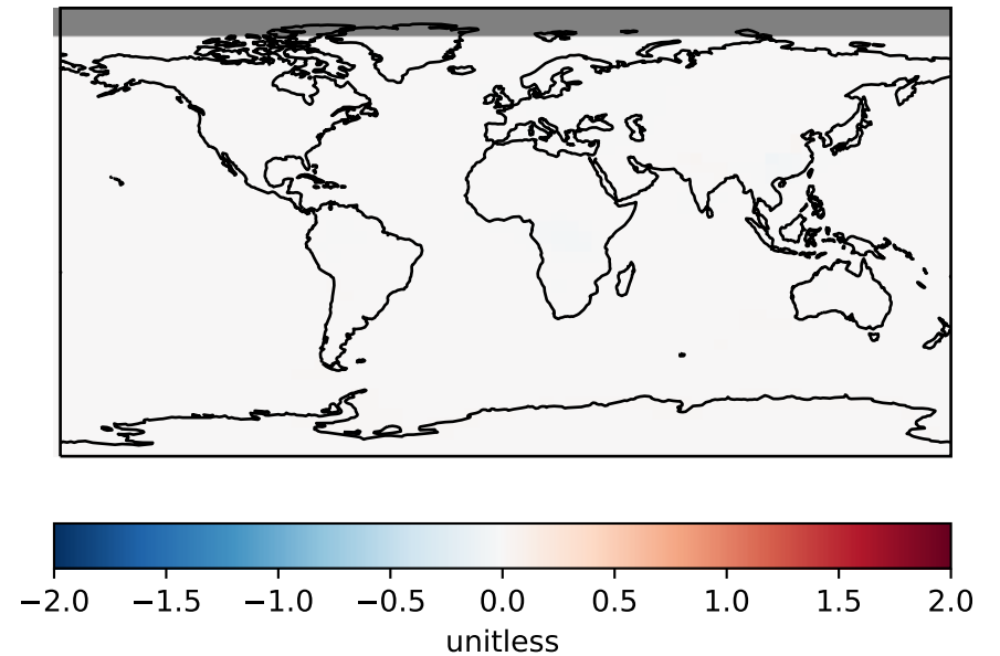
Fractional Difference (Dev-Ref)/Ref, Fixed Range
