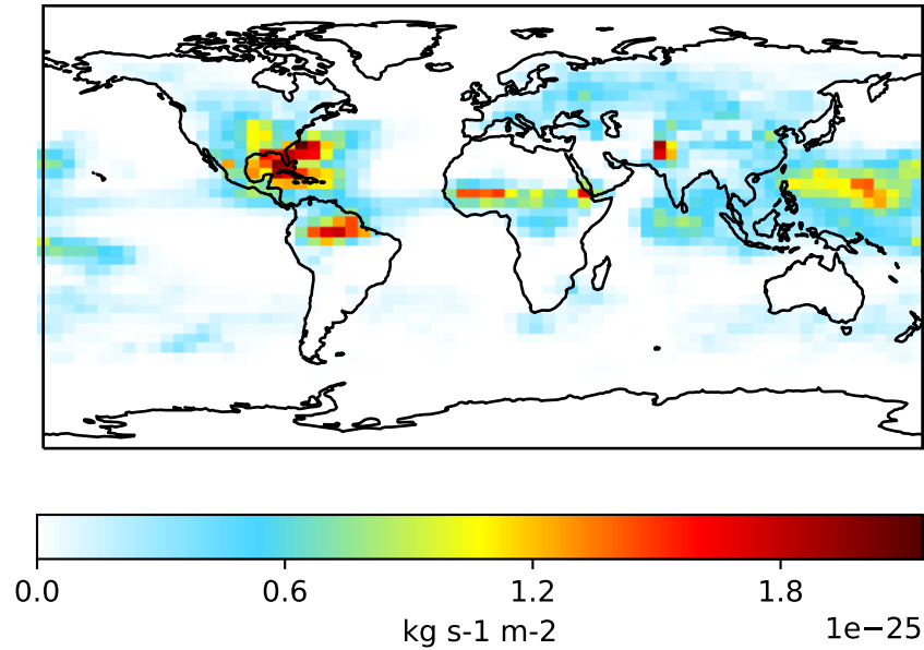
TransportTracers-StdWetdep (Ref), Normalized by Area 4.0x5.0
