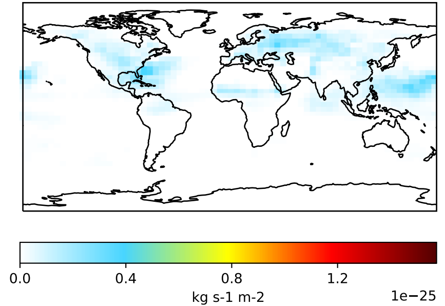
TransportTracers-LuoWetdep (Dev), Normalized by Area 4.0x5.0
