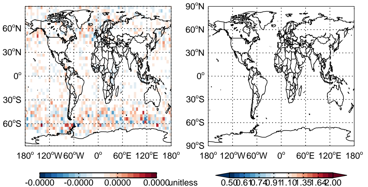
v11-01 - v10-01 Abs Diff: Sum opt depth (OPTD*CLDTOT) below 500hPa v11-01 / v10-01 Ratio: Sum opt depth (OPTD*CLDTOT) below 500hPa
