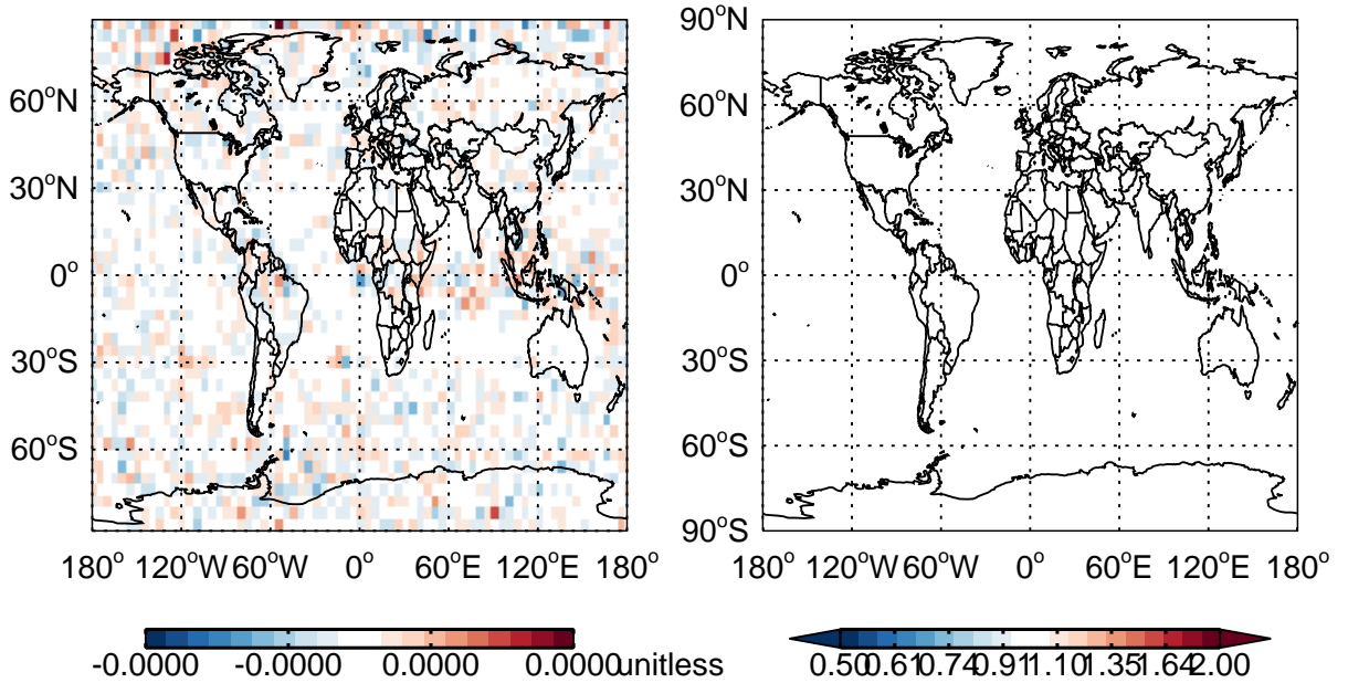
v11-01 - v10-01 Abs Diff: Max cloud fraction (CLDTOT) in column v11-01 / v10-01 Ratio: Max cloud fraction (CLDTOT) in column
