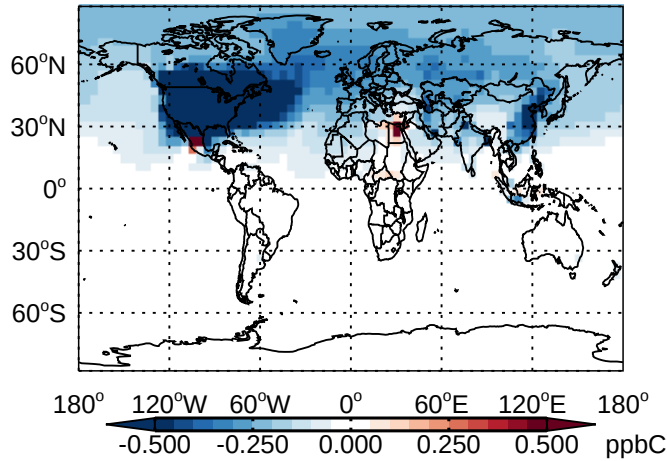
v11-01 - v10-01 ALK4 - Diff @ Surface for Jan
