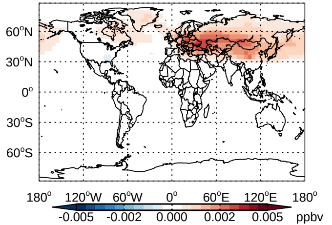
v11-01 - v10-01 HNO4- Diff @ 500 hPa for Jan
