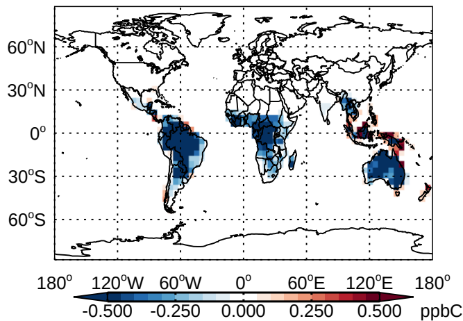
v11-01 - v10-01 ISOP - Diff @ Surface for Jan
