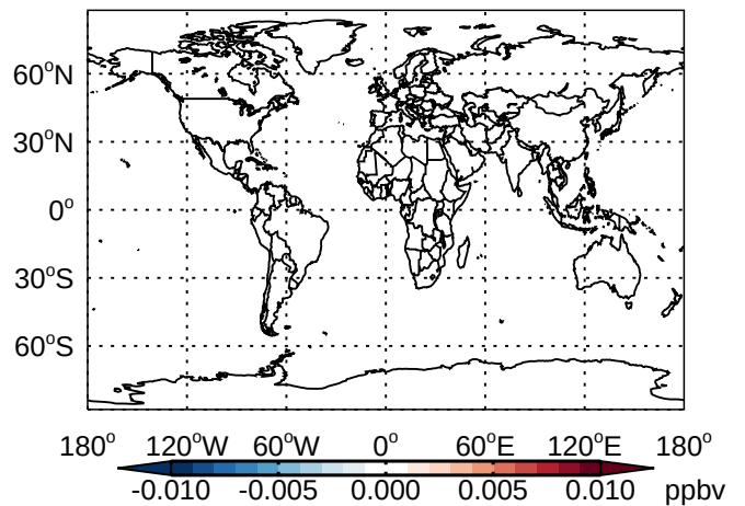
v11-01 - v10-01 Br- Diff @ 500 hPa for Jan
