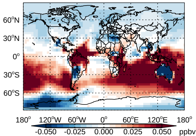
v11-01 - v10-01 MP - Diff @ Surface for Jan
