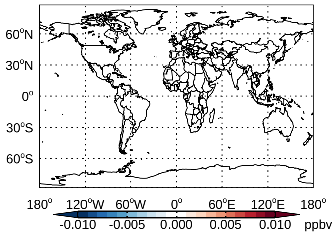
v11-01 - v10-01 HBr - Diff @ Surface for Jan
