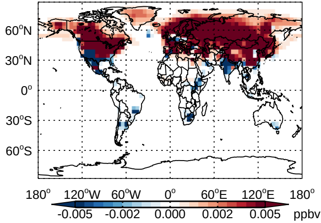
v11-01 - v10-01 N2O5 - Diff @ Surface for Jan
