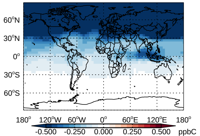
v11-01 - v10-01 C2H6- Diff @ 500 hPa for Jan
