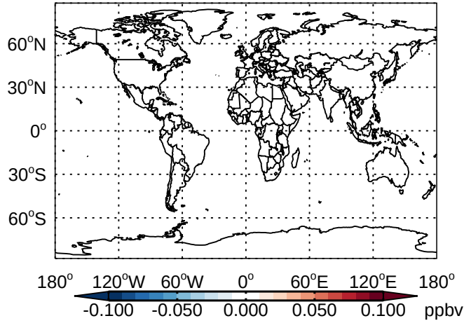
v11-01 - v10-01 HCl - Diff @ Surface for Jan
