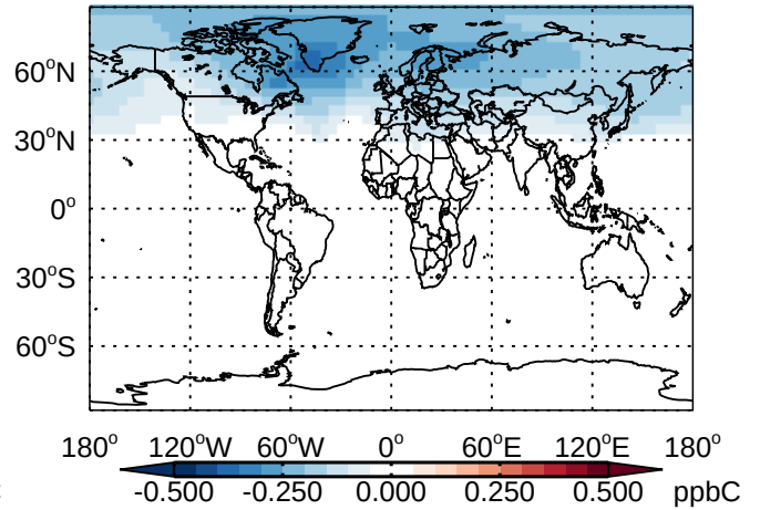
v11-01 - v10-01 ALK4- Diff @ 500 hPa for Jan
