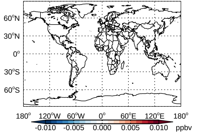
v11-01 - v10-01 BrO - Diff @ 500 hPa for Jan
