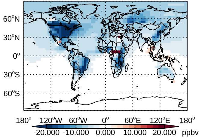
v11-01 - v10-01 CO - Diff @ Surface for Jan
