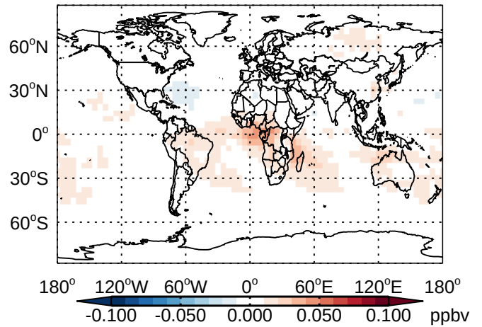
v11-01 - v10-01 HNO 3 - Diff @ 500 hPa for Jan
