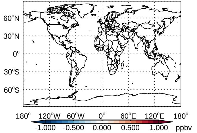
v11-01 - v10-01 NO- Diff @ 500 hPa for Jan
