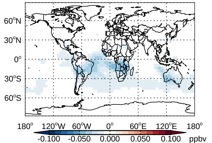
v11-01 - v10-01 H 2 O 2 - Diff @ 500 hPa for Jan
