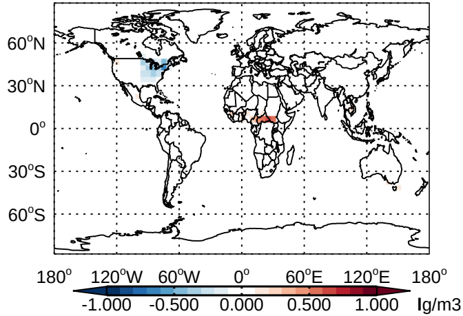
v11-01 - v10-01 OCPO - Diff @ Surface for Jan
