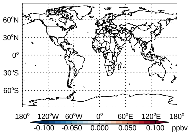
v11-01 - v10-01 CH3Cl - Diff @ Surface for Jan
