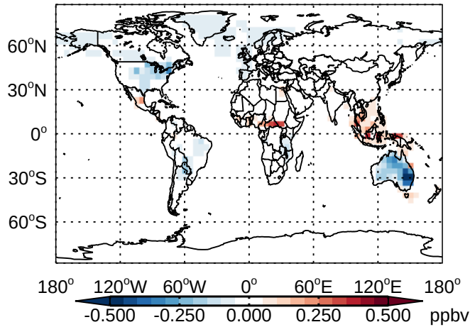
v11-01 - v10-01 CH2O - Diff @ Surface for Jan
