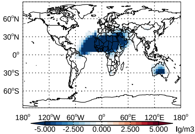
v11-01 - v10-01 DST1 - Diff @ Surface for Jan
