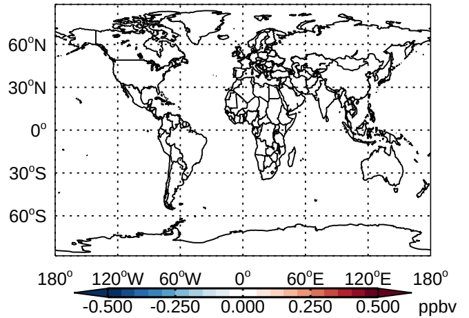
v11-01 - v10-01 CH2O- Diff @ 500 hPa for Jan
