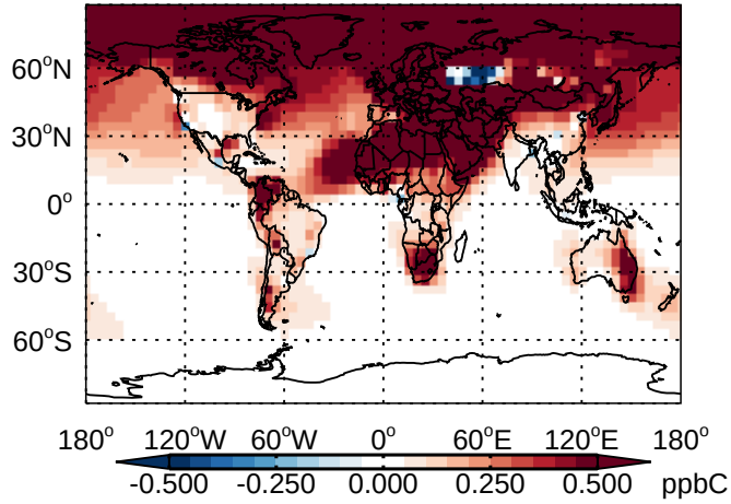
v11-01 - v10-01 C3H8 - Diff @ Surface for Jan
