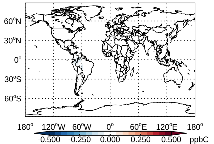
v11-01 - v10-01 ISOP- Diff @ 500 hPa for Jan
