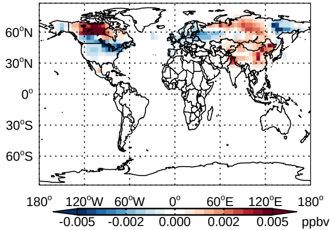
v11-01 - v10-01 HNO4 - Diff @ Surface for Jan
