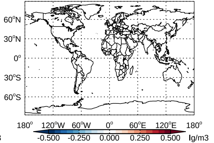
v11-01 - v10-01 NH4- Diff @ 500 hPa for Jan
