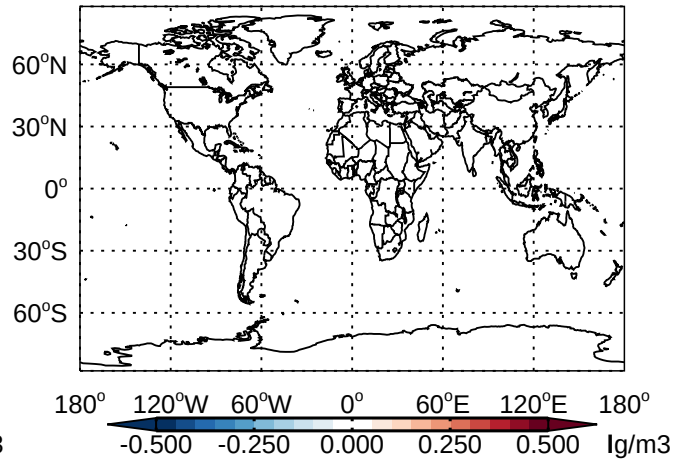
v11-01 - v10-01 NIT- Diff @ 500 hPa for Jan
