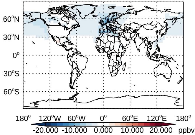
v11-01 - v10-01 O3 - Diff @ Surface for Jan
