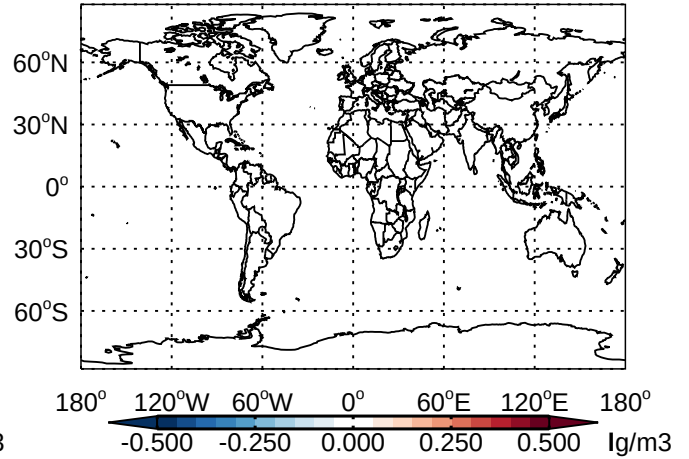
v11-01 - v10-01 OCPO- Diff @ 500 hPa for Jan
