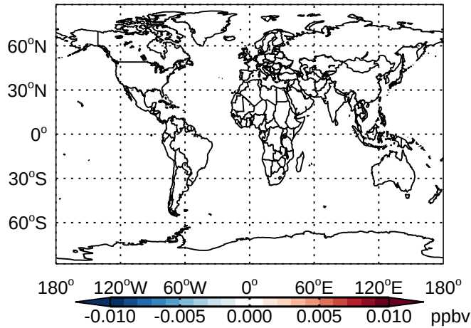
v11-01 - v10-01 Br2 - Diff @ Surface for Jan
