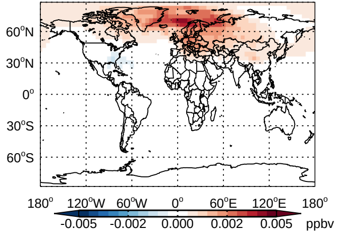
v11-01 - v10-01 N2O5- Diff @ 500 hPa for Jan
