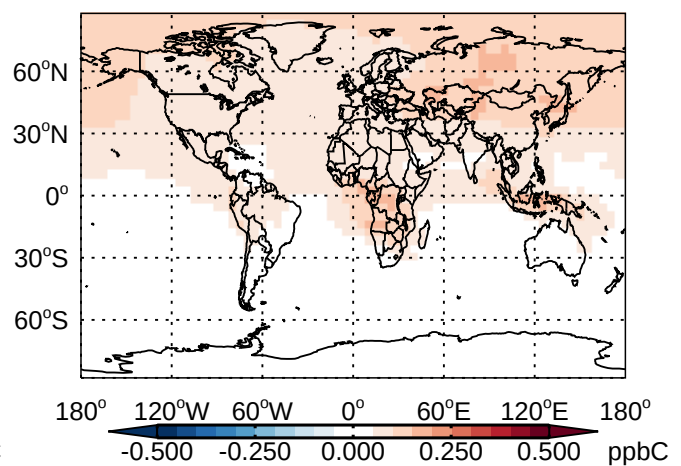
v11-01 - v10-01 ACET- Diff @ 500 hPa for Jan
