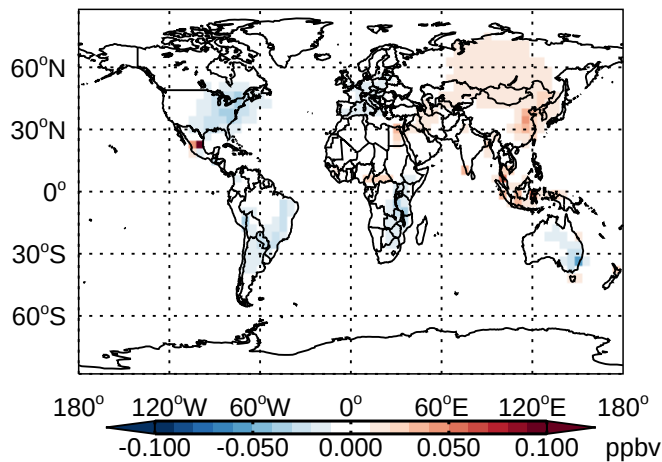
v11-01 - v10-01 PAN - Diff @ Surface for Jan
