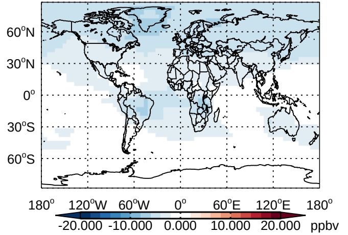
v11-01 - v10-01 CO- Diff @ 500 hPa for Jan
