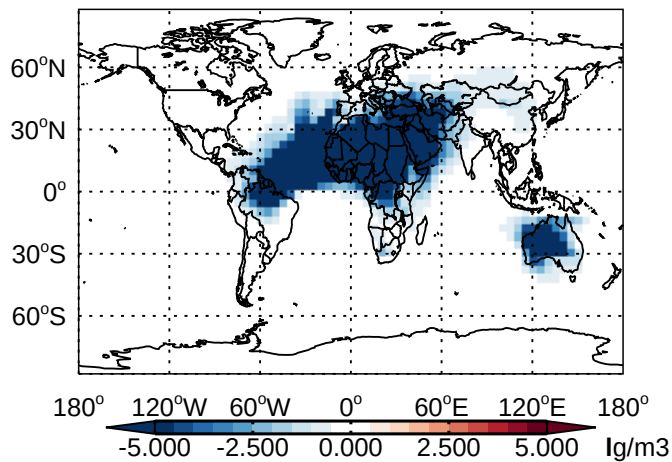
v11-01 - v10-01 DST2 - Diff @ Surface for Jan
