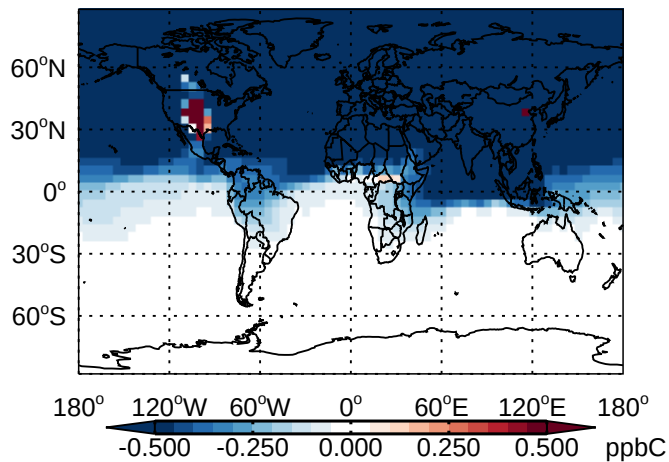
v11-01 - v10-01 C2H6 - Diff @ Surface for Jan
