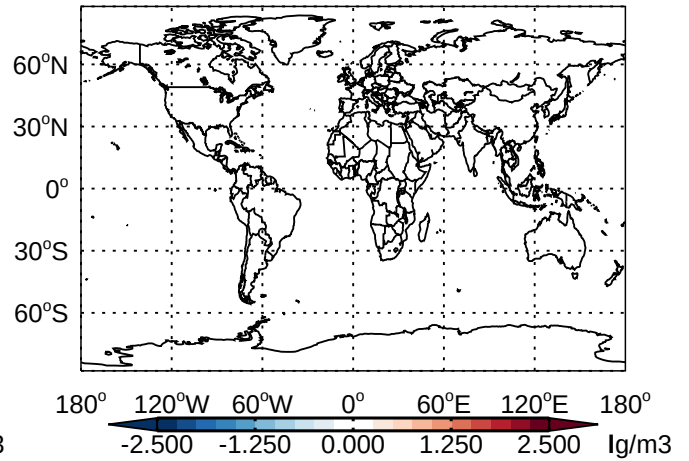
v11-01 - v10-01 DST1- Diff @ 500 hPa for Jan
