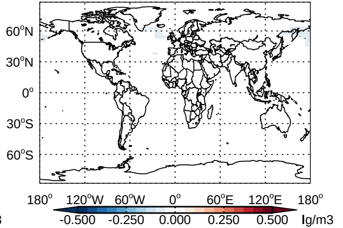
v11-01 - v10-01 SALC- Diff @ 500 hPa for Jan
