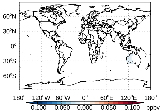
v11-01 - v10-01 PAN- Diff @ 500 hPa for Jan
