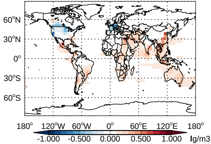
v11-01 - v10-01 NH4 - Diff @ Surface for Jan
