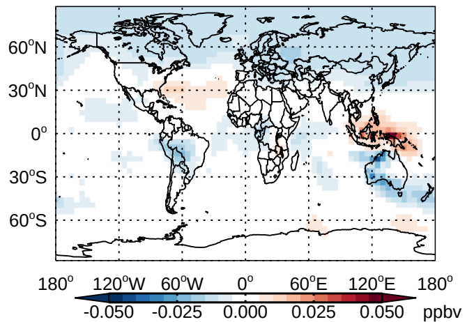
v11-01 - v10-01 MP- Diff @ 500 hPa for Jan
