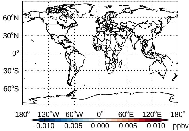
v11-01 - v10-01 BrO - Diff @ Surface for Jan
