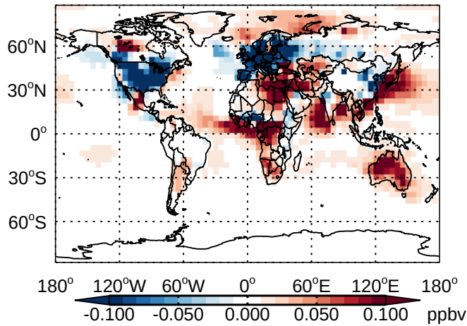
v11-01 - v10-01 HNO 3 - Diff @ Surface for Jan
