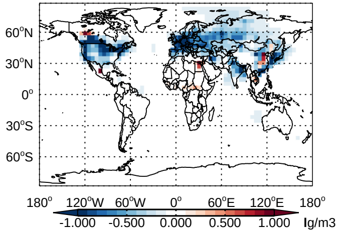
v11-01 - v10-01 NIT - Diff @ Surface for Jan
