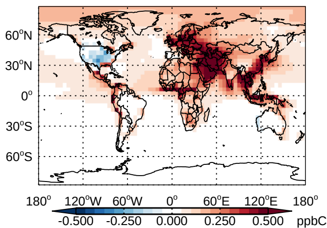
v11-01 - v10-01 ACET - Diff @ Surface for Jan
