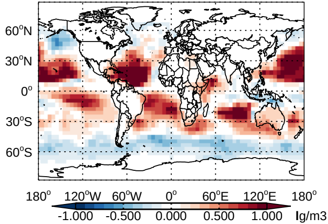
v11-01 - v10-01 SALC - Diff @ Surface for Jan
