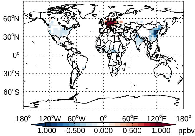
v11-01 - v10-01 NO - Diff @ Surface for Jan
