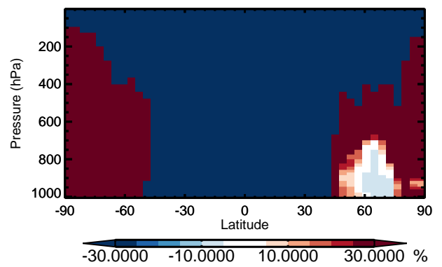
v11-01 / v10-01 ISOP - Zonal mean % diff for Apr
