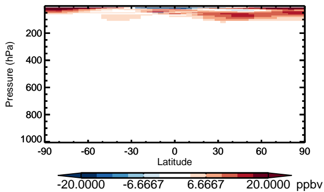
v11-01 - v10-01 O3 - Zonal mean abs diff for Apr
