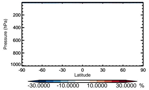
v11-01 / v10-01 CH 2 Br 2 - Zonal mean % diff for Apr
