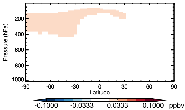
v11-01 - v10-01 HCFC141b - Zonal mean abs diff for Apr
