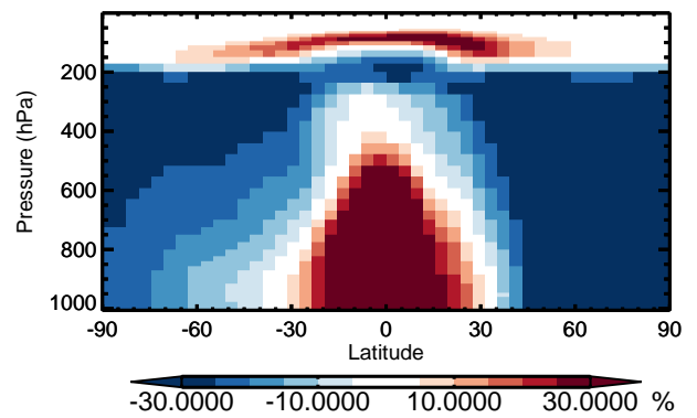
v11-01 / v10-01 MSA - Zonal mean % diff for Apr
