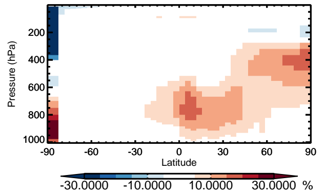
v11-01 / v10-01 ClOO - Zonal mean % diff for Apr
