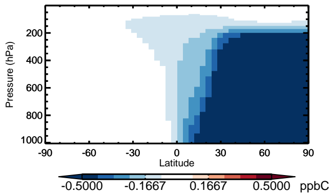
v11-01 - v10-01 C2H6 - Zonal mean abs diff for Apr
