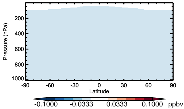
v11-01 - v10-01 CFC115 - Zonal mean abs diff for Apr
