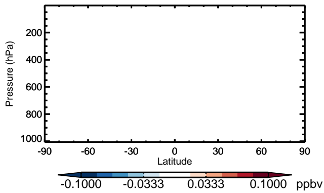
v11-01 - v10-01 MTPA - Zonal mean abs diff for Apr
