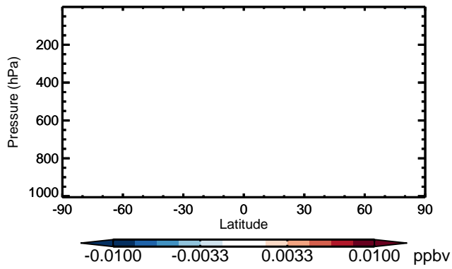
v11-01 - v10-01 BrO - Zonal mean abs diff for Apr
