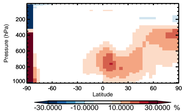
v11-01 / v10-01 Cl - Zonal mean % diff for Apr
