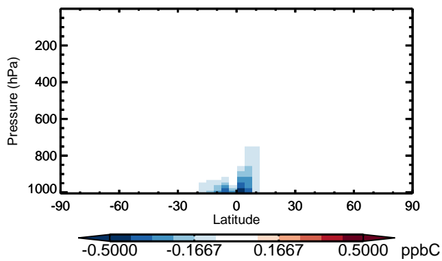
v11-01 - v10-01 ISOP - Zonal mean abs diff for Apr
