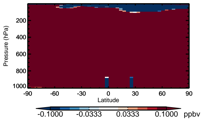
v11-01 - v10-01 CH4 - Zonal mean abs diff for Apr
