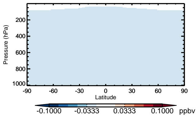
v11-01 - v10-01 HCFC123 - Zonal mean abs diff for Apr
