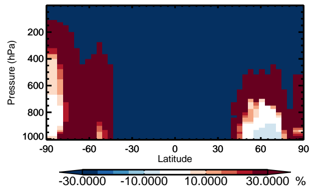
v11-01 / v10-01 MTPA - Zonal mean % diff for Apr
