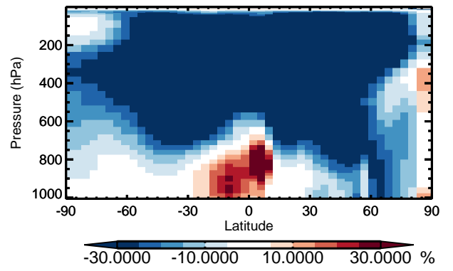
v11-01 / v10-01 OCIO - Zonal mean % diff for Apr
