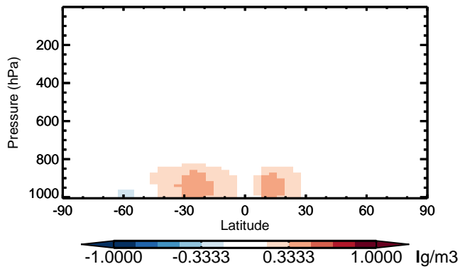
v11-01 - v10-01 SALC - Zonal mean abs diff for Apr
