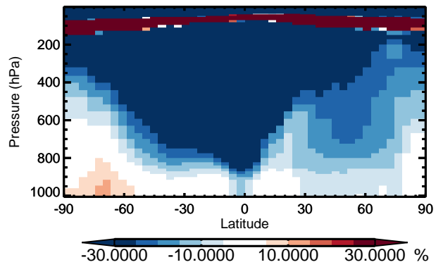
v11-01 / v10-01 OCPO - Zonal mean % diff for Apr
