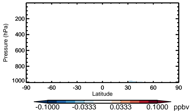
v11-01 - v10-01 XYLE - Zonal mean abs diff for Apr
