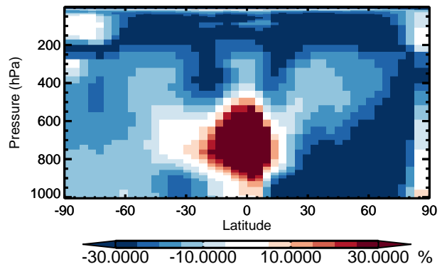
v11-01 / v10-01 Br2 - Zonal mean % diff for Apr
