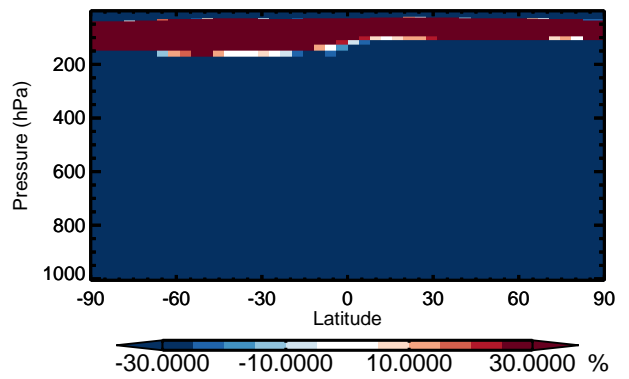
v11-01 / v10-01 DST2 - Zonal mean % diff for Apr
