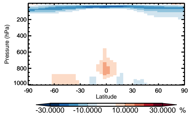
v11-01 / v10-01 PAN - Zonal mean % diff for Apr
