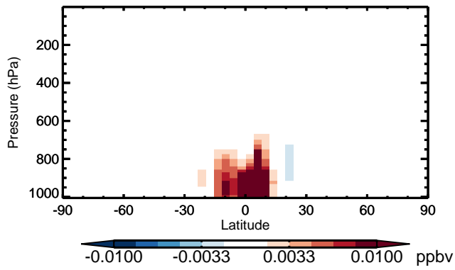
v11-01 - v10-01 IEPOX - Zonal mean abs diff for Apr
