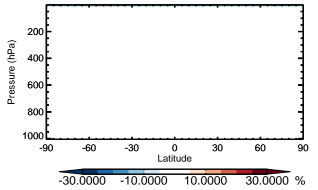
v11-01 / v10-01 OCS - Zonal mean % diff for Apr
