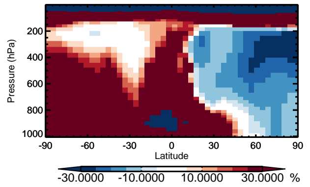
v11-01 / v10-01 IEPOX - Zonal mean % diff for Apr
