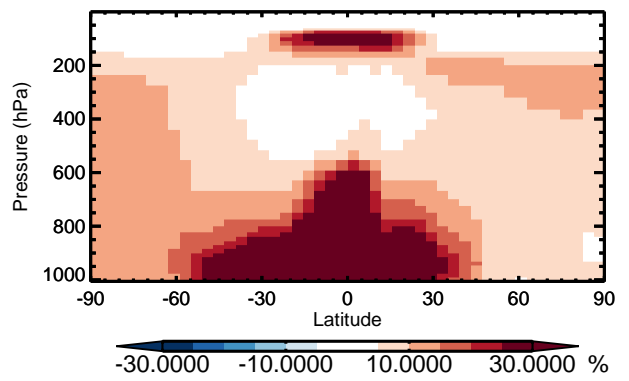
v11-01 / v10-01 TSOG3 - Zonal mean % diff for Apr
