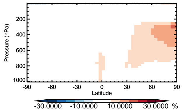
v11-01 / v10-01 CH2O - Zonal mean % diff for Apr
