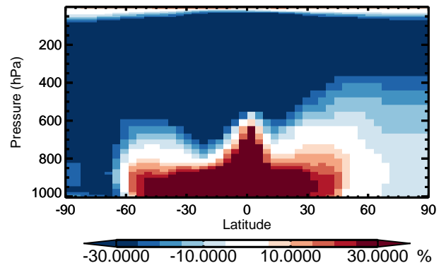
v11-01 / v10-01 TSOA0 - Zonal mean % diff for Apr
