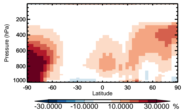
v11-01 / v10-01 MPN - Zonal mean % diff for Apr
