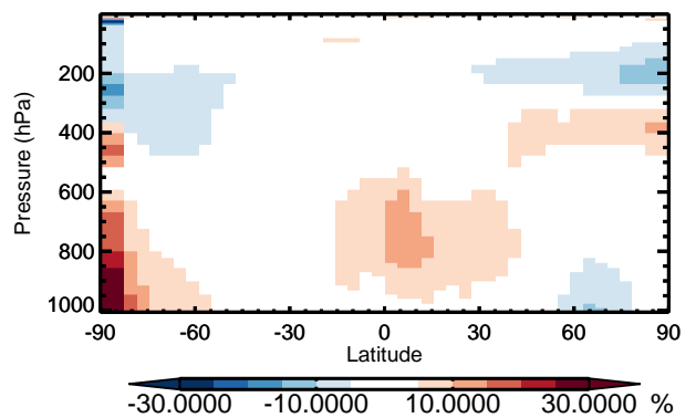
v11-01 / v10-01 ClO - Zonal mean % diff for Apr
