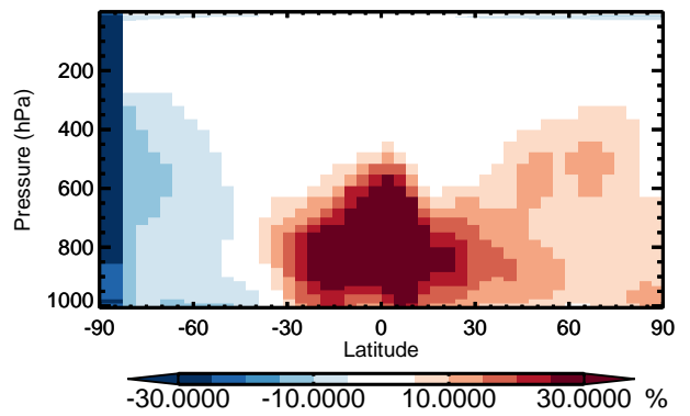
v11-01 / v10-01 Br - Zonal mean % diff for Apr
