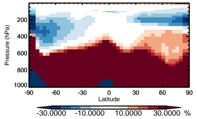
v11-01 / v10-01 Cl 2 O 2 - Zonal mean % diff for Apr
