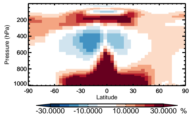
v11-01 / v10-01 ISOG1 - Zonal mean % diff for Apr
