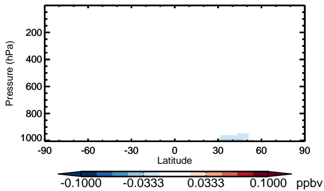
v11-01 - v10-01 TOLU - Zonal mean abs diff for Apr
