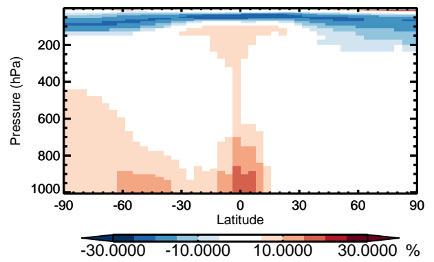
v11-01 / v10-01 MAP - Zonal mean % diff for Apr
