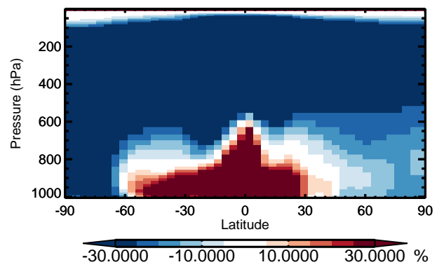
v11-01 / v10-01 ISOA2 - Zonal mean % diff for Apr
