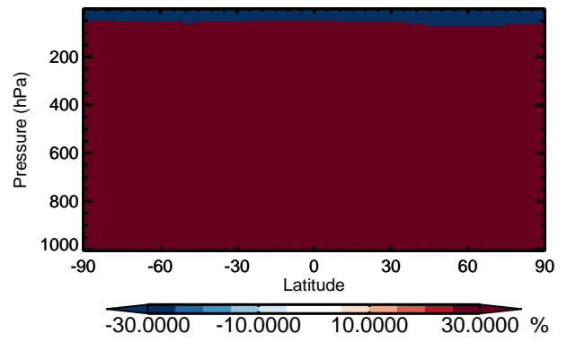
v11-01 / v10-01 MVKN - Zonal mean % diff for Apr
