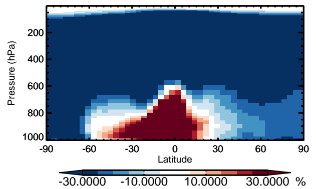
v11-01 / v10-01 ASOA3 - Zonal mean % diff for Apr
