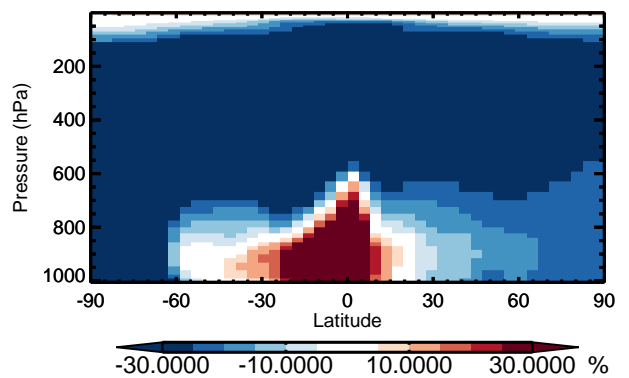
v11-01 / v10-01 ASOA1 - Zonal mean % diff for Apr
