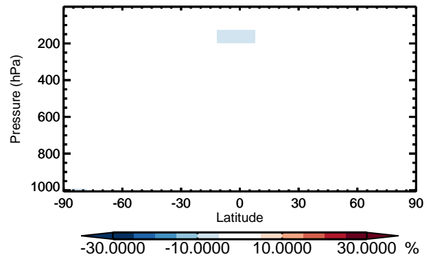
v11-01 / v10-01 H 2 O - Zonal mean % diff for Apr
