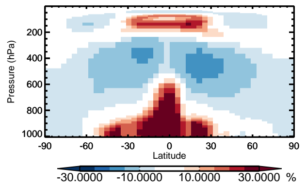
v11-01 / v10-01 ISOG2 - Zonal mean % diff for Apr
