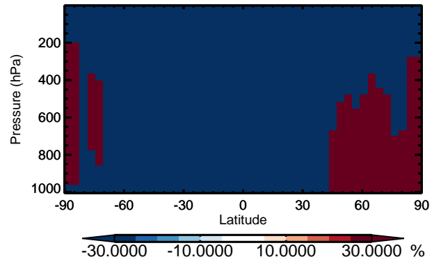
v11-01 / v10-01 ISOPND - Zonal mean % diff for Apr
