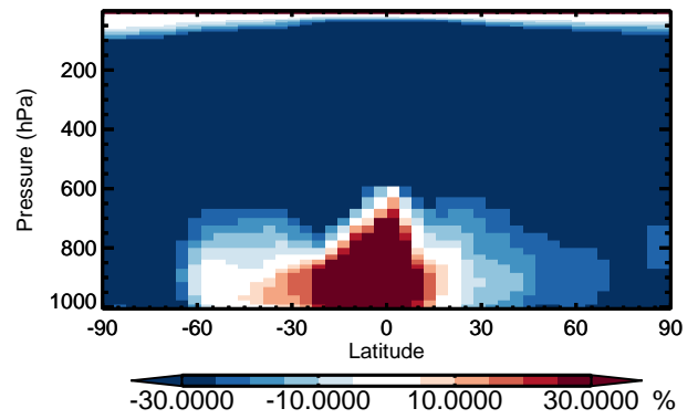
v11-01 / v10-01 ASOA2 - Zonal mean % diff for Apr
