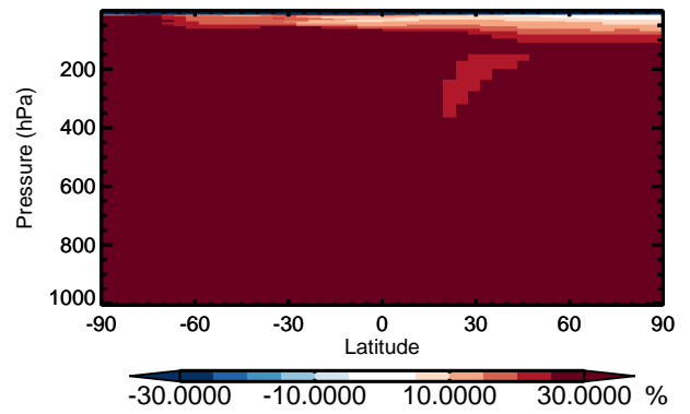
v11-01 / v10-01 C3H8 - Zonal mean % diff for Apr
