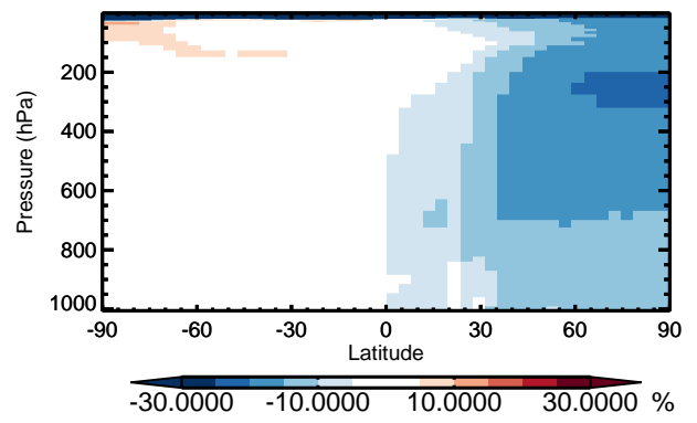
v11-01 / v10-01 ALK4 - Zonal mean % diff for Apr
