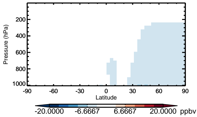
v11-01 - v10-01 CO - Zonal mean abs diff for Apr
