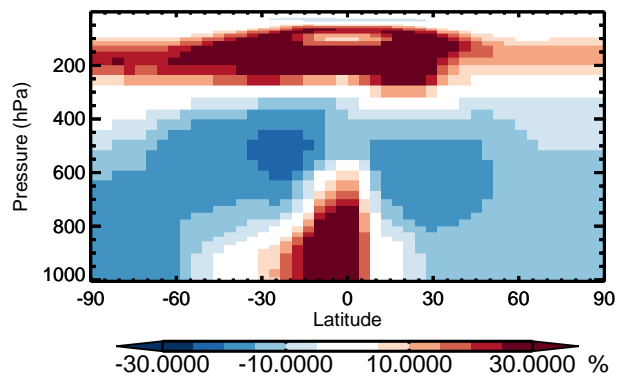
v11-01 / v10-01 ASOG1 - Zonal mean % diff for Apr
