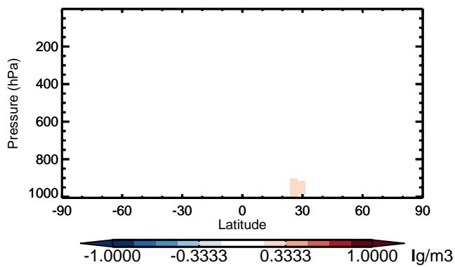
v11-01 - v10-01 SO 4 - Zonal mean abs diff for Apr
