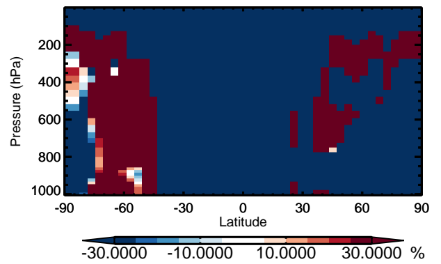
v11-01 / v10-01 MOBA - Zonal mean % diff for Apr
