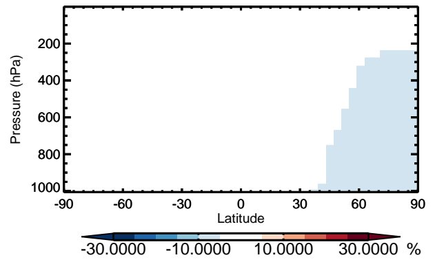
v11-01 / v10-01 CO - Zonal mean % diff for Apr
