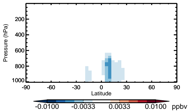
v11-01 - v10-01 MACRN - Zonal mean abs diff for Apr
