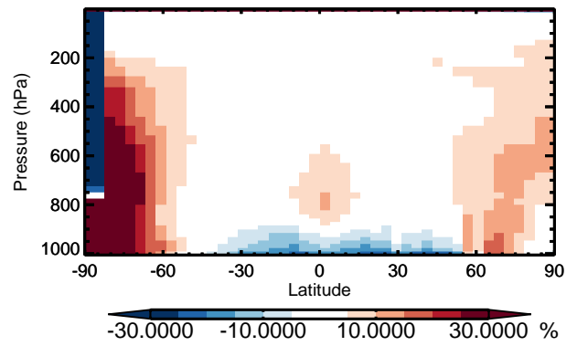
v11-01 / v10-01 NO - Zonal mean % diff for Apr
