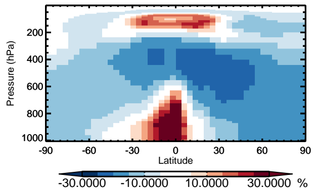
v11-01 / v10-01 ASOG2 - Zonal mean % diff for Apr
