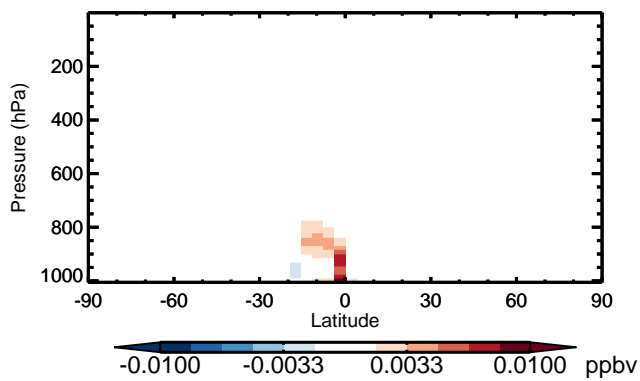
v11-01 - v10-01 RIP - Zonal mean abs diff for Apr
