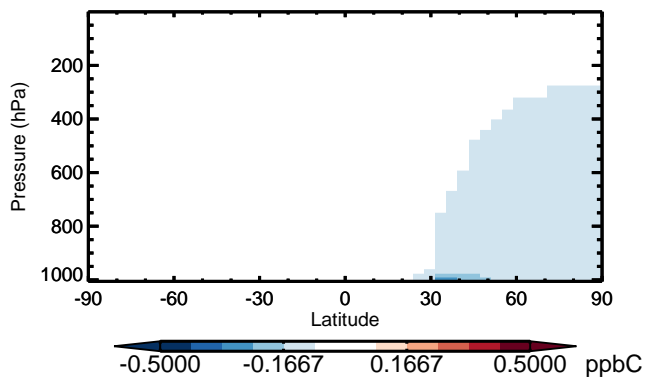
v11-01 - v10-01 ALK4 - Zonal mean abs diff for Apr
