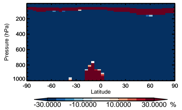
v11-01 / v10-01 MACRN - Zonal mean % diff for Apr
