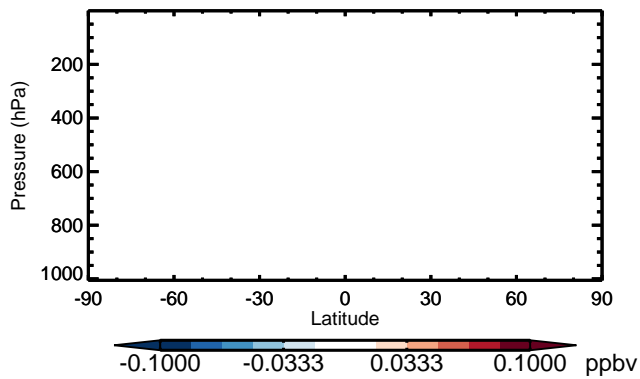
v11-01 - v10-01 ASOG2 - Zonal mean abs diff for Apr
