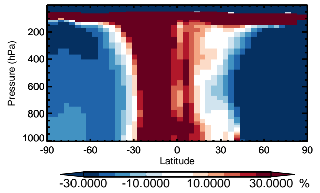
v11-01 / v10-01 DMS - Zonal mean % diff for Apr
