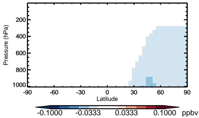
v11-01 - v10-01 BENZ - Zonal mean abs diff for Apr
