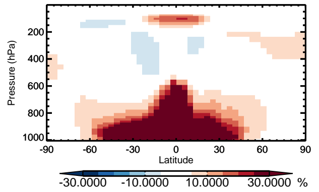
v11-01 / v10-01 ISOA3 - Zonal mean % diff for Apr
