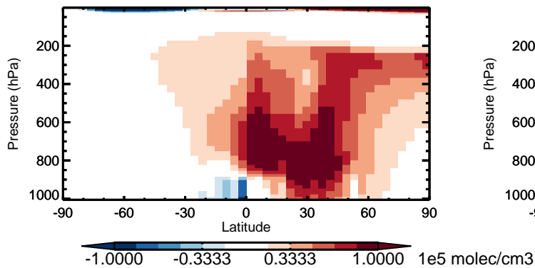
v11-01 - v10-01 OH - Zonal mean abs diff for Apr
