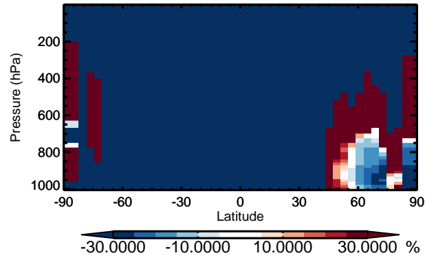
v11-01 / v10-01 ISOPNB - Zonal mean % diff for Apr
