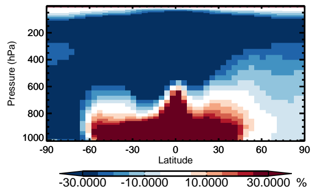
v11-01 / v10-01 ISOA1 - Zonal mean % diff for Apr
