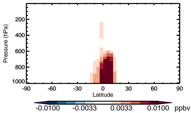
v11-01 - v10-01 MAP - Zonal mean abs diff for Apr
