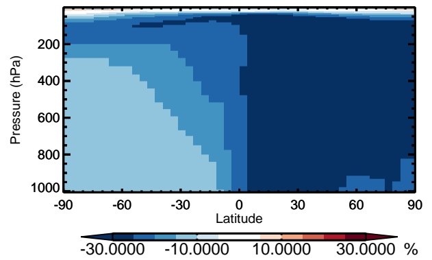
v11-01 / v10-01 C2H6 - Zonal mean % diff for Apr
