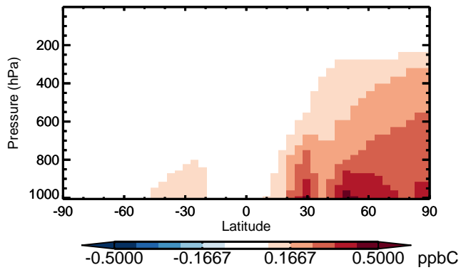
v11-01 - v10-01 C3H8 - Zonal mean abs diff for Apr
