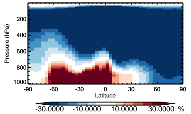
v11-01 / v10-01 TSOA0 - Zonal mean % diff for Jan
