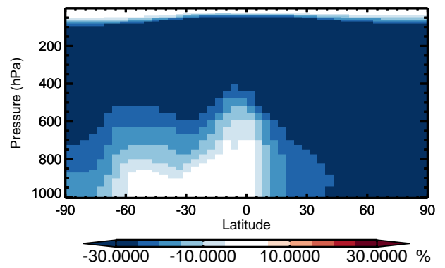
v11-01 / v10-01 ASOAN - Zonal mean % diff for Jan
