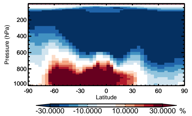
v11-01 / v10-01 TSOA2 - Zonal mean % diff for Jan
