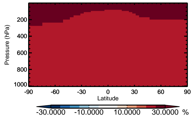
v11-01 / v10-01 HCFC142b - Zonal mean % diff for Jan
