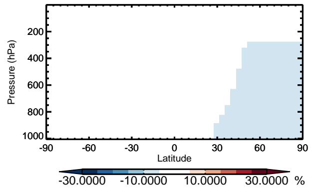
v11-01 / v10-01 CO - Zonal mean % diff for Jan
