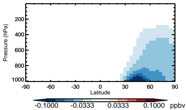
v11-01 - v10-01 TOLU - Zonal mean abs diff for Jan
