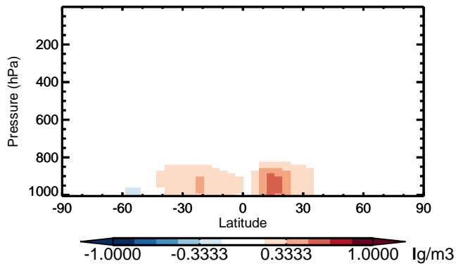
v11-01 - v10-01 SALC - Zonal mean abs diff for Jan
