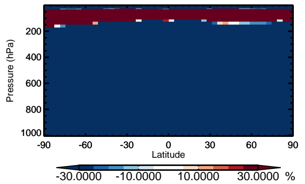
v11-01 / v10-01 DST2 - Zonal mean % diff for Jan
