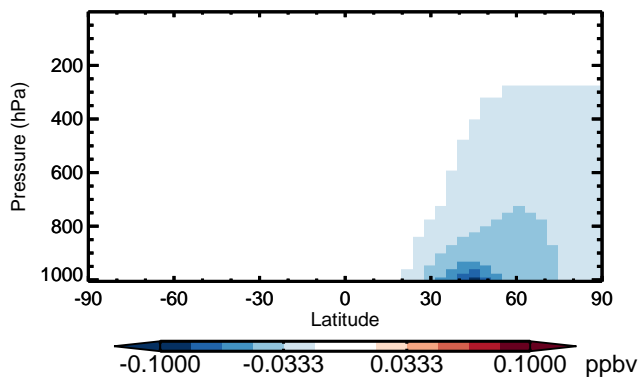
v11-01 - v10-01 BENZ - Zonal mean abs diff for Jan
