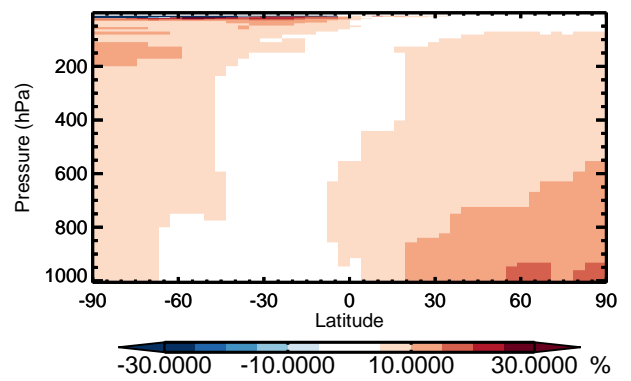
v11-01 / v10-01 ACET - Zonal mean % diff for Jan
