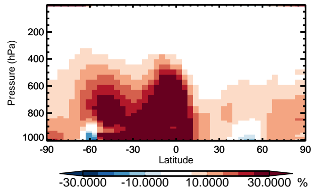
v11-01 / v10-01 HNO 3 - Zonal mean % diff for Jan
