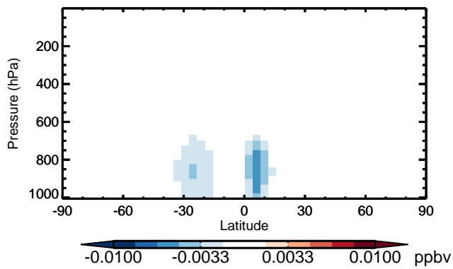
v11-01 - v10-01 MACRN - Zonal mean abs diff for Jan
