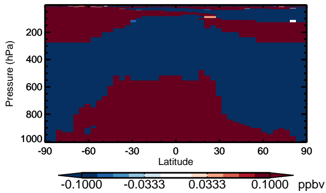
v11-01 - v10-01 H2O - Zonal mean abs diff for Jan
