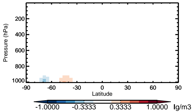
v11-01 - v10-01 DMS - Zonal mean abs diff for Jan
