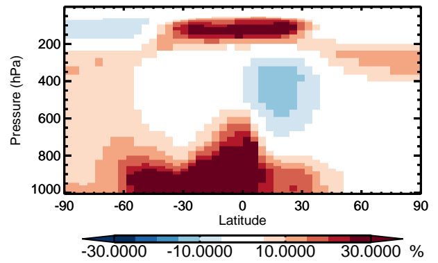
v11-01 / v10-01 TSOG2 - Zonal mean % diff for Jan
