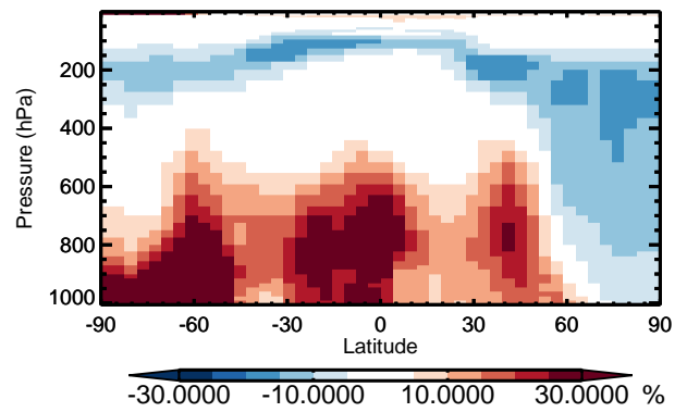
v11-01 / v10-01 Cl2 - Zonal mean % diff for Jan
