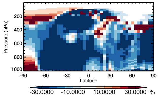
v11-01 / v10-01 NH 3 - Zonal mean % diff for Jan
