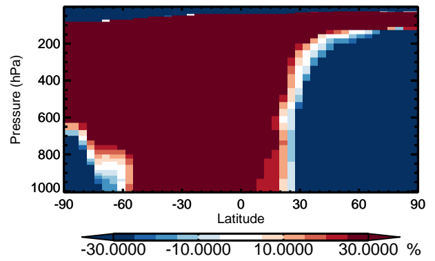
v11-01 / v10-01 DMS - Zonal mean % diff for Jan
