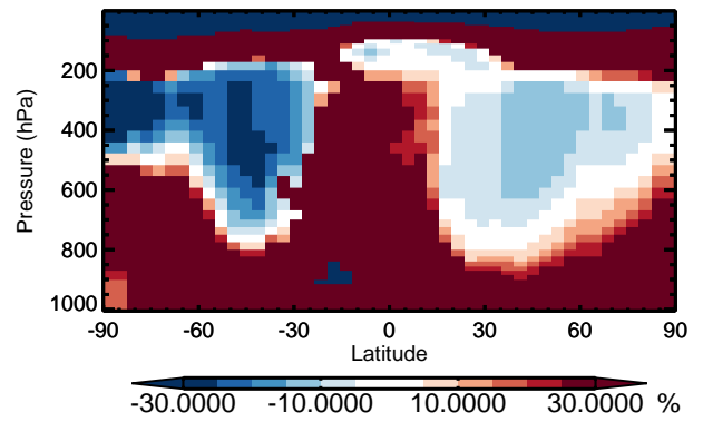
v11-01 / v10-01 IEPOX - Zonal mean % diff for Jan
