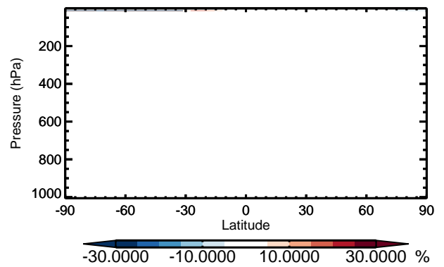
v11-01 / v10-01 CH 3 Br - Zonal mean % diff for Jan
