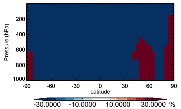
v11-01 / v10-01 RIP - Zonal mean % diff for Jan
