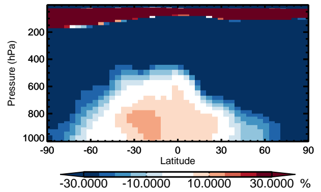
v11-01 / v10-01 SALC - Zonal mean % diff for Jan
