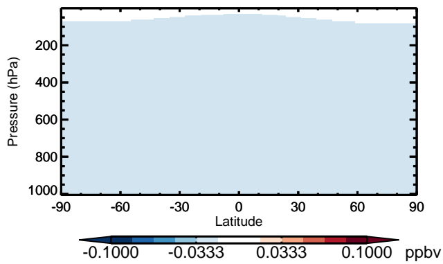
v11-01 - v10-01 HCFC123 - Zonal mean abs diff for Jan
