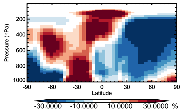
v11-01 / v10-01 SO 2 - Zonal mean % diff for Jan
