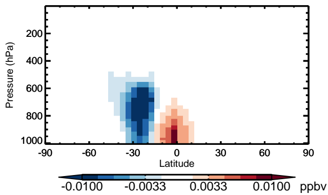
v11-01 - v10-01 MAP - Zonal mean abs diff for Jan
