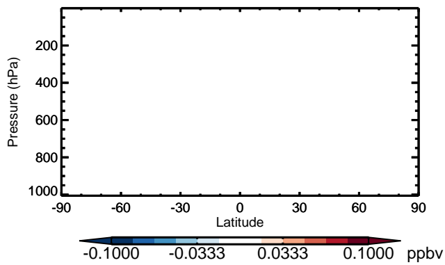
v11-01 - v10-01 ISOPNB - Zonal mean abs diff for Jan
