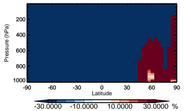
v11-01 / v10-01 ISOP - Zonal mean % diff for Jan
