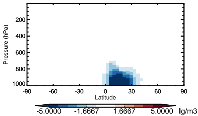
v11-01 - v10-01 DST2 - Zonal mean abs diff for Jan
