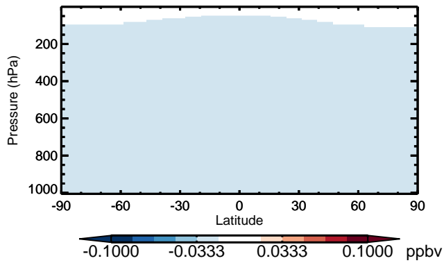
v11-01 - v10-01 CFC115 - Zonal mean abs diff for Jan
