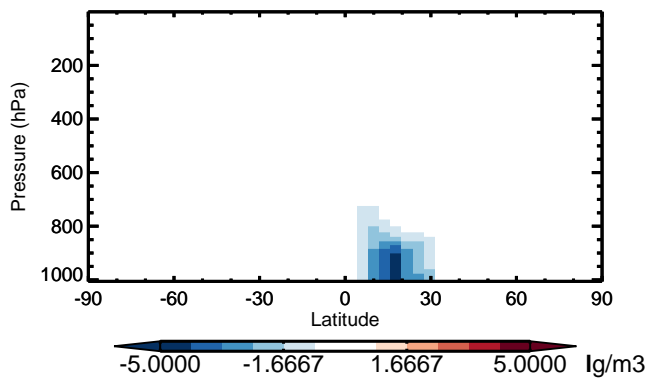
v11-01 - v10-01 DST1 - Zonal mean abs diff for Jan
