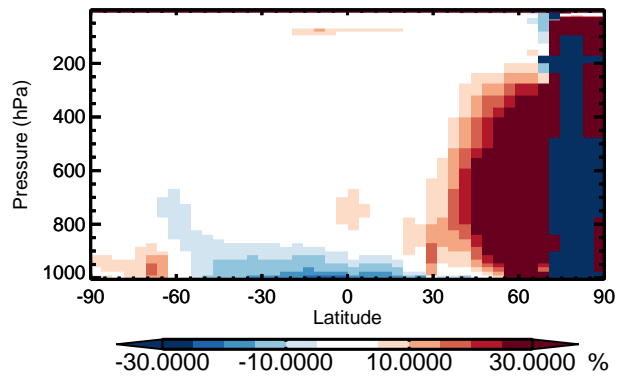
v11-01 / v10-01 NO - Zonal mean % diff for Jan
