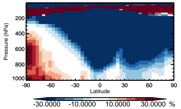
v11-01 / v10-01 OCPO - Zonal mean % diff for Jan
