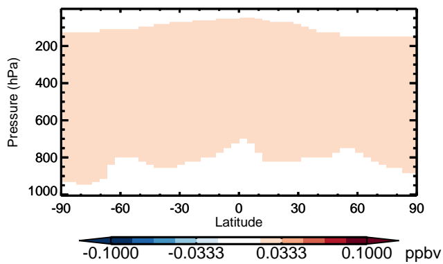
v11-01 - v10-01 HCFC141b - Zonal mean abs diff for Jan
