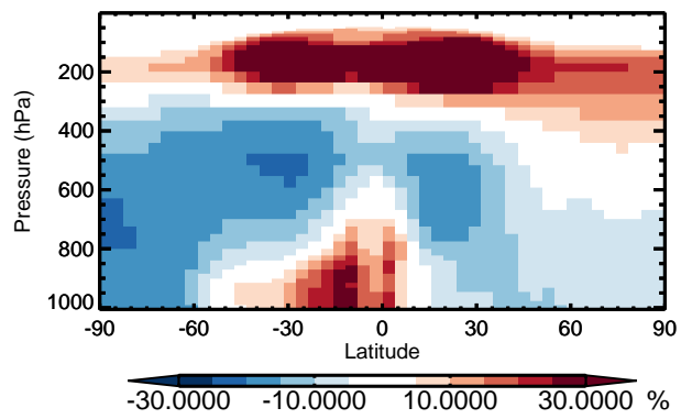
v11-01 / v10-01 ASOG1 - Zonal mean % diff for Jan
