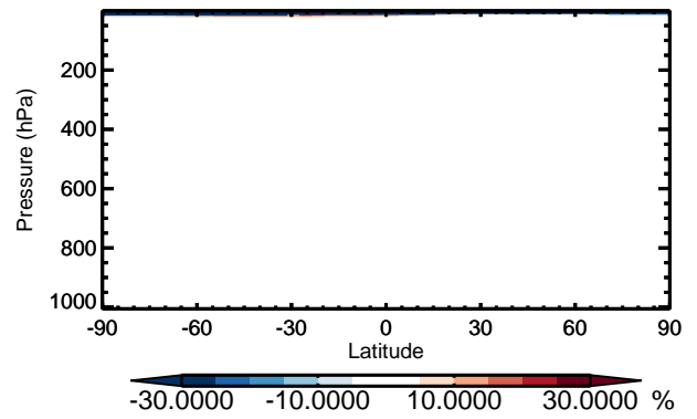
v11-01 / v10-01 CH 2 Br 2 - Zonal mean % diff for Jan
