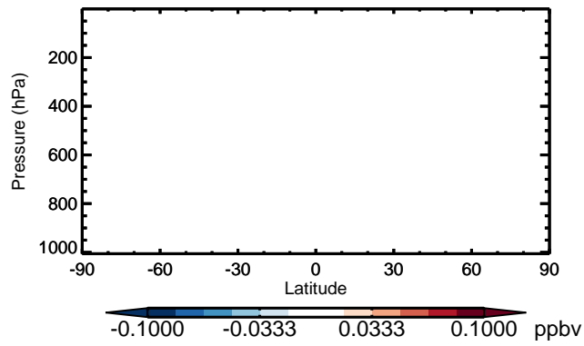
v11-01 - v10-01 CFC11 - Zonal mean abs diff for Jan
