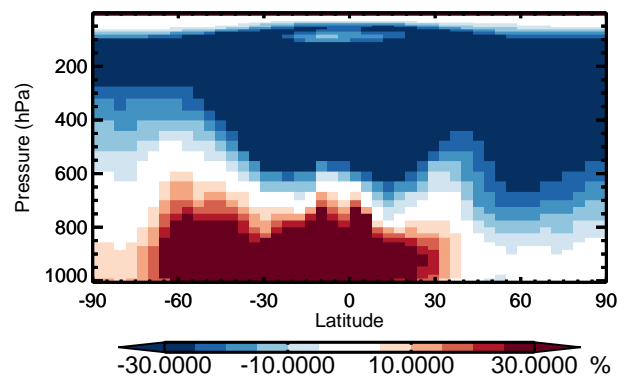
v11-01 / v10-01 TSOA3 - Zonal mean % diff for Jan
