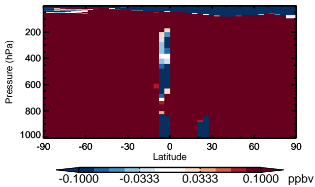
v11-01 - v10-01 CH4 - Zonal mean abs diff for Jan
