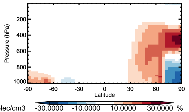
v11-01 / v10-01 OH - Zonal mean % diff for Jan
