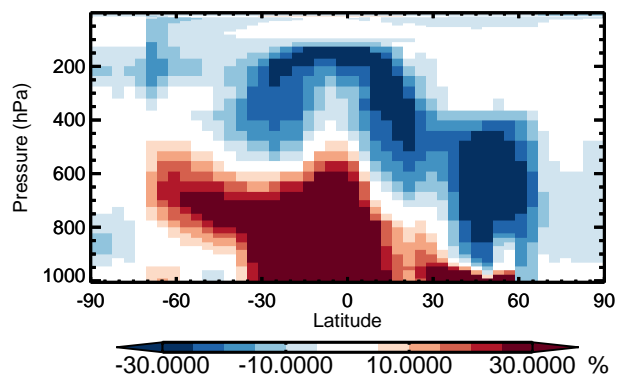
v11-01 / v10-01 BrCl - Zonal mean % diff for Jan
