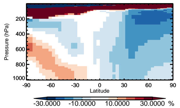
v11-01 / v10-01 TOLU - Zonal mean % diff for Jan
