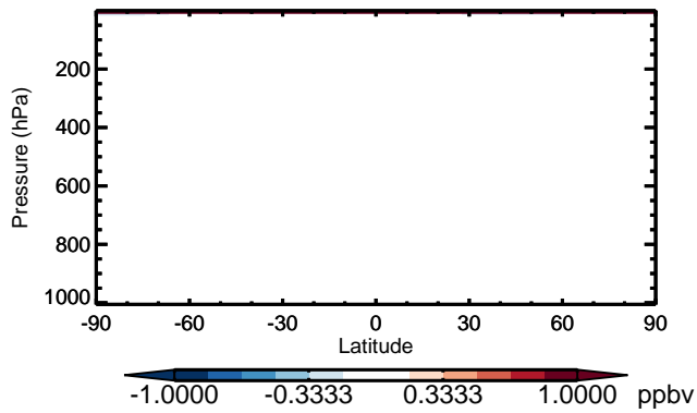
v11-01 - v10-01 NO - Zonal mean abs diff for Jan
