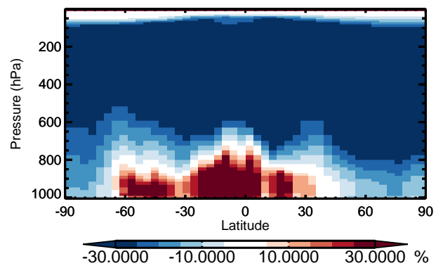
v11-01 / v10-01 ISOA2 - Zonal mean % diff for Jan
