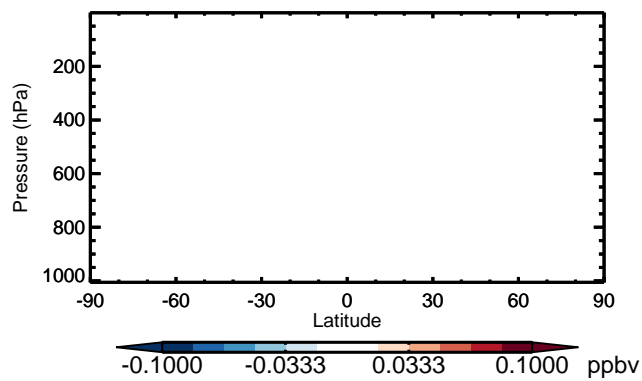
v11-01 - v10-01 TSOA3 - Zonal mean abs diff for Jan
