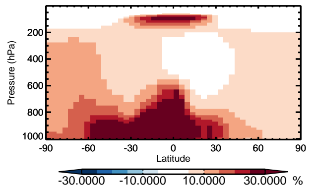
v11-01 / v10-01 TSOG3 - Zonal mean % diff for Jan
