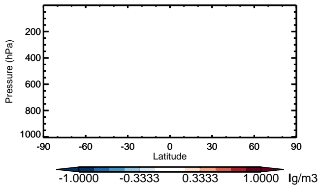
v11-01 - v10-01 NH 3 - Zonal mean abs diff for Jan
