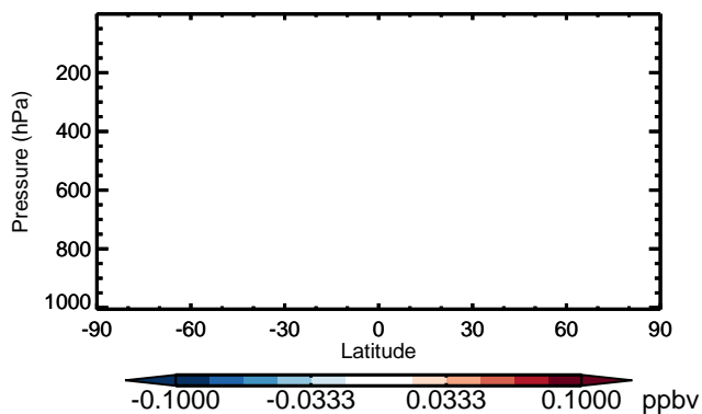
v11-01 - v10-01 TSOG0 - Zonal mean abs diff for Jan
