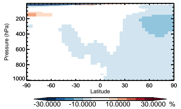
v11-01 / v10-01 BENZ - Zonal mean % diff for Jan
