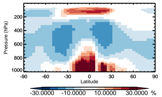
v11-01 / v10-01 ISOG2 - Zonal mean % diff for Jan
