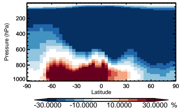
v11-01 / v10-01 TSOA1 - Zonal mean % diff for Jan
