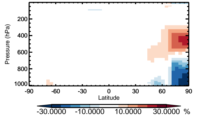
v11-01 / v10-01 HO2 - Zonal mean % diff for Jan
