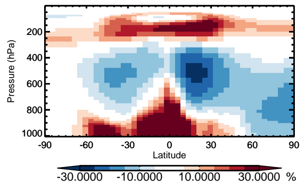
v11-01 / v10-01 ISOG1 - Zonal mean % diff for Jan
