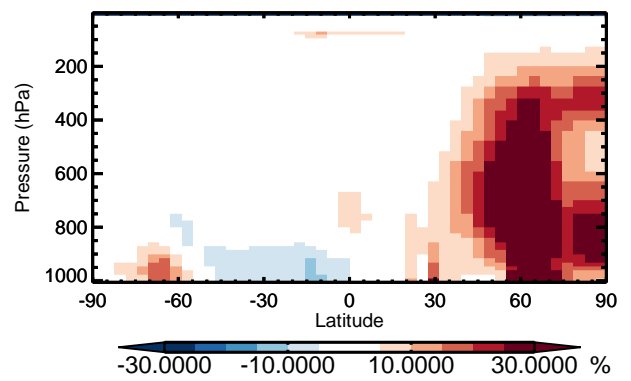
v11-01 / v10-01 NO2 - Zonal mean % diff for Jan
