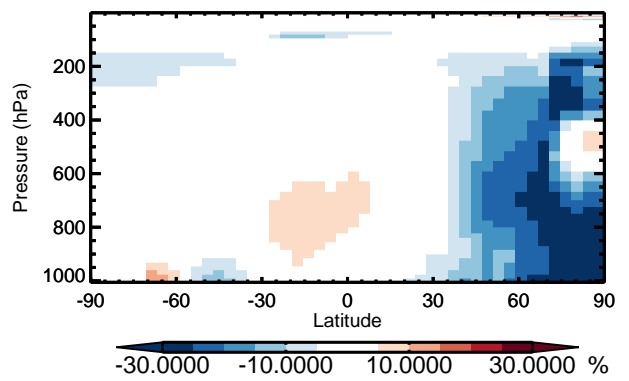
v11-01 / v10-01 ClO - Zonal mean % diff for Jan
