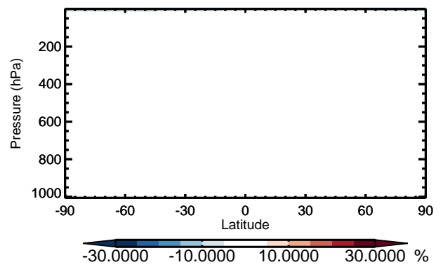
v11-01 / v10-01 H1301 - Zonal mean % diff for Jan
