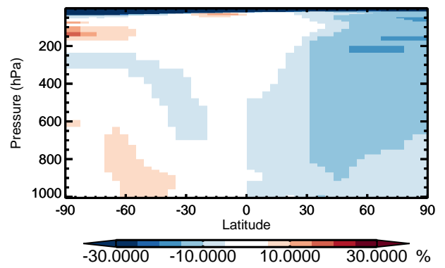
v11-01 / v10-01 ALK4 - Zonal mean % diff for Jan
