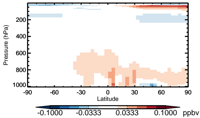
v11-01 - v10-01 HNO 3 - Zonal mean abs diff for Jan
