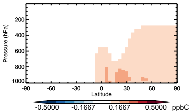
v11-01 - v10-01 ACET - Zonal mean abs diff for Jan
