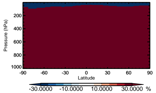
v11-01 / v10-01 MVKN - Zonal mean % diff for Jan
