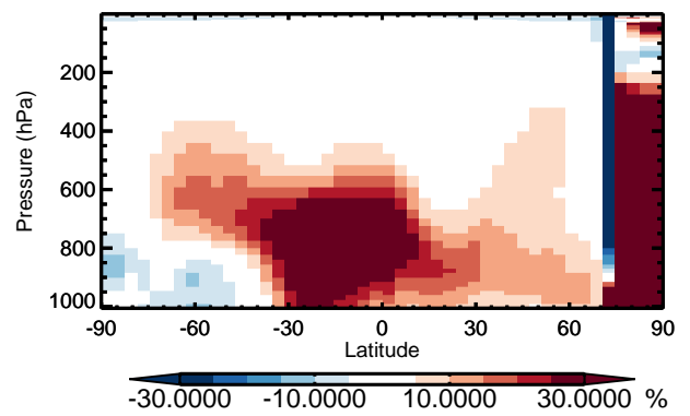
v11-01 / v10-01 Br - Zonal mean % diff for Jan
