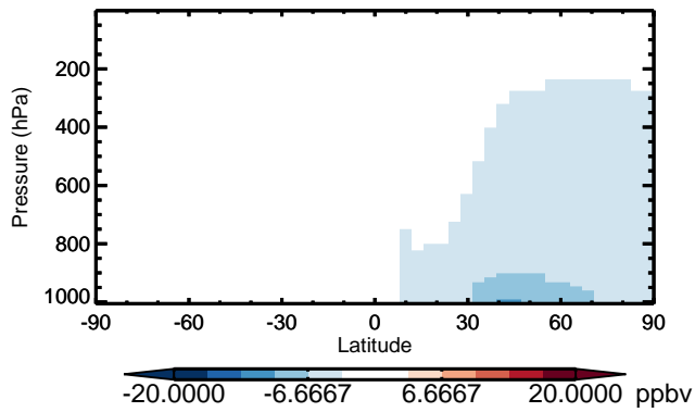
v11-01 - v10-01 CO - Zonal mean abs diff for Jan
