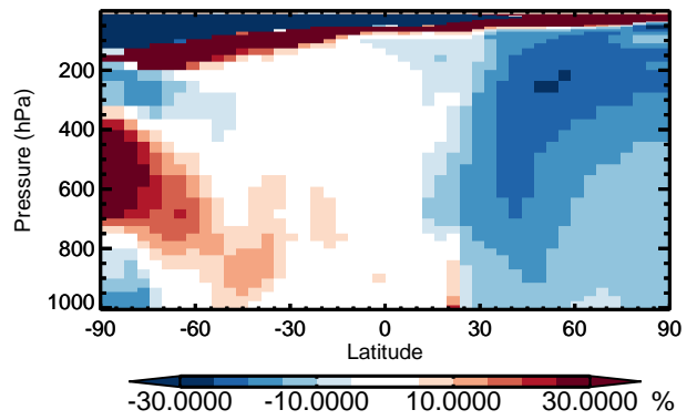
v11-01 / v10-01 XYLE - Zonal mean % diff for Jan
