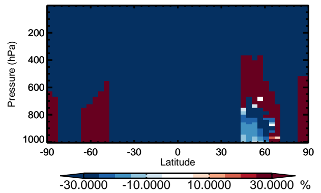
v11-01 / v10-01 MTPA - Zonal mean % diff for Jan
