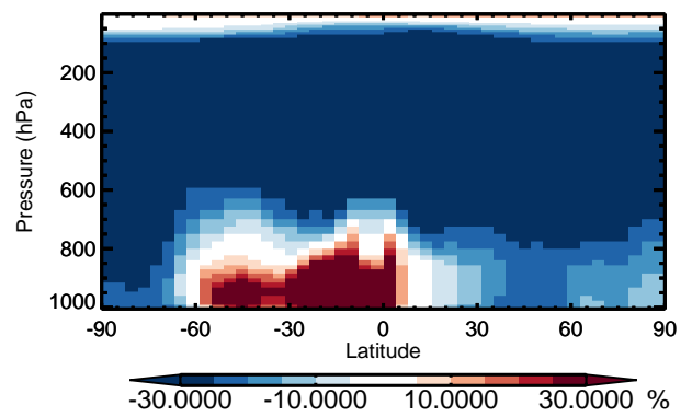
v11-01 / v10-01 ASOA1 - Zonal mean % diff for Jan
