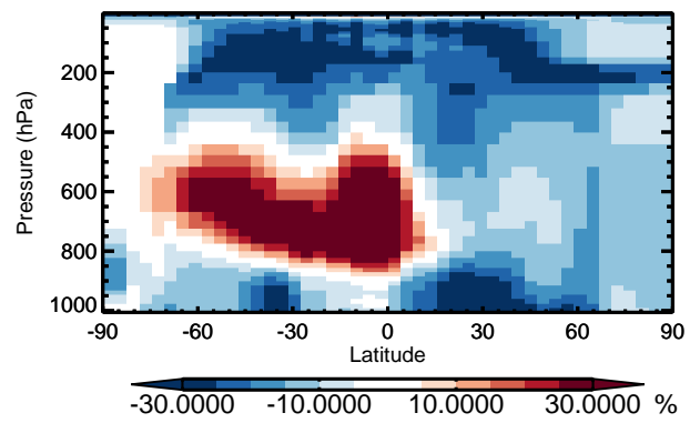
v11-01 / v10-01 Br2 - Zonal mean % diff for Jan
