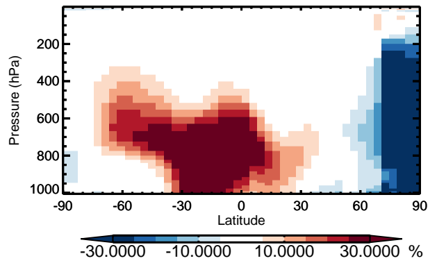
v11-01 / v10-01 BrO - Zonal mean % diff for Jan
