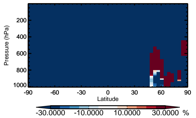
v11-01 / v10-01 ISOPNB - Zonal mean % diff for Jan
