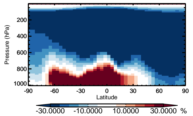
v11-01 / v10-01 ISOA1 - Zonal mean % diff for Jan
