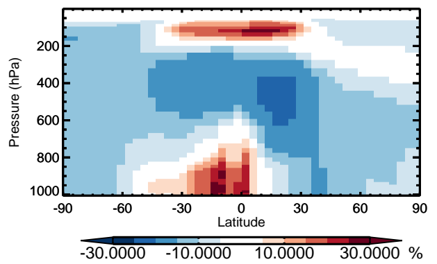
v11-01 / v10-01 ASOG2 - Zonal mean % diff for Jan
