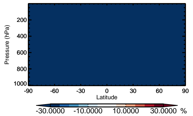
v11-01 / v10-01 HCFC123 - Zonal mean % diff for Jan
