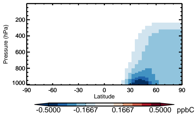
v11-01 - v10-01 ALK4 - Zonal mean abs diff for Jan
