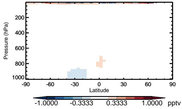
v11-01 - v10-01 HO2 - Zonal mean abs diff for Jan
