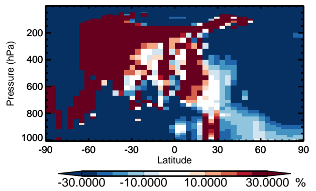
v11-01 / v10-01 NIT - Zonal mean % diff for Jan
