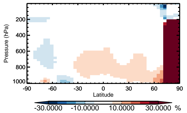
v11-01 / v10-01 Cl - Zonal mean % diff for Jan
