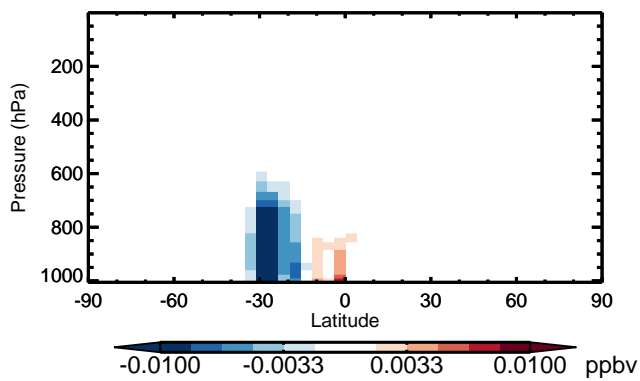
v11-01 - v10-01 RIP - Zonal mean abs diff for Jan
