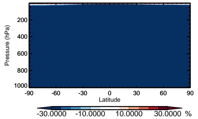
v11-01 / v10-01 CFC115 - Zonal mean % diff for Jan
