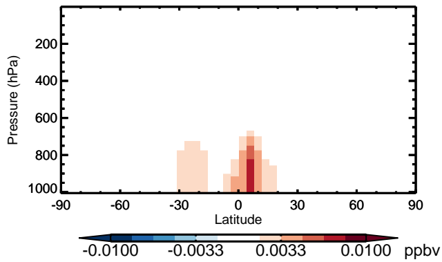
v11-01 - v10-01 MVKN - Zonal mean abs diff for Jan
