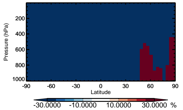
v11-01 / v10-01 ISOPND - Zonal mean % diff for Jan
