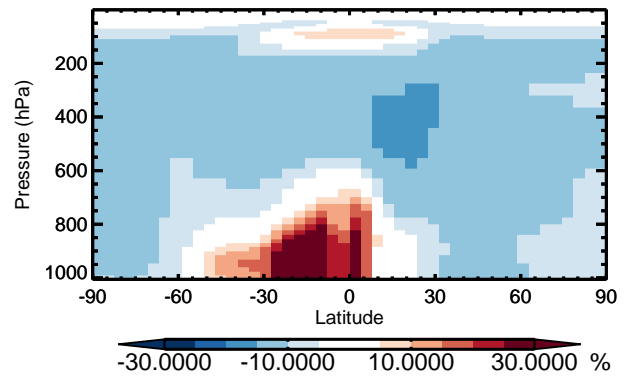
v11-01 / v10-01 ASOG3 - Zonal mean % diff for Jan
