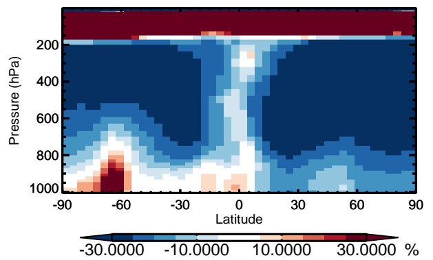
v11-01 / v10-01 DST1 - Zonal mean % diff for Jan
