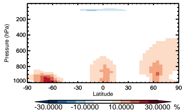
v11-01 / v10-01 H 2 O 2 - Zonal mean % diff for Jan
