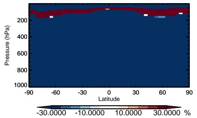
v11-01 / v10-01 MACRN - Zonal mean % diff for Jan
