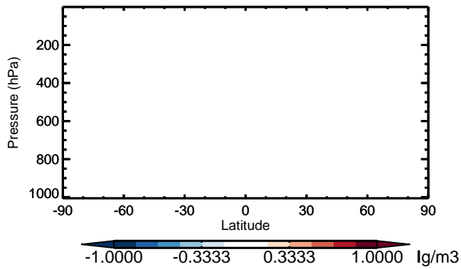
v11-01 - v10-01 OCPO - Zonal mean abs diff for Jan
