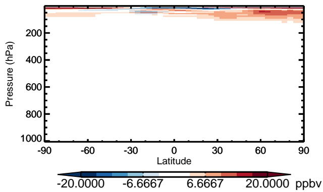
v11-01 - v10-01 O3 - Zonal mean abs diff for Jan
