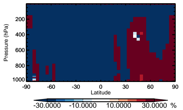
v11-01 / v10-01 MOBA - Zonal mean % diff for Jan
