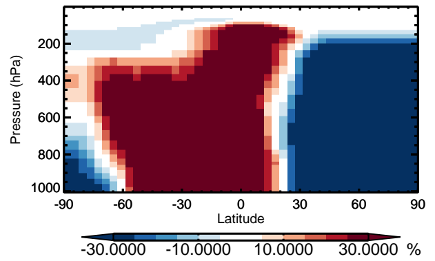
v11-01 / v10-01 MSA - Zonal mean % diff for Jan
