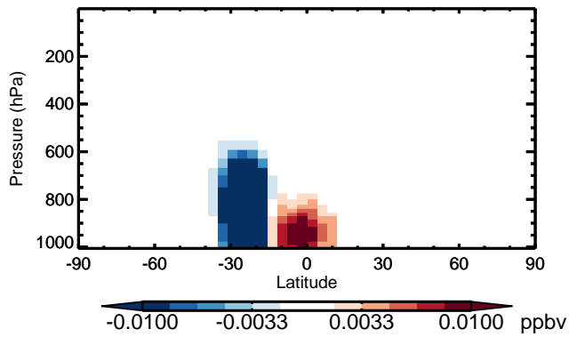
v11-01 - v10-01 IEPOX - Zonal mean abs diff for Jan
