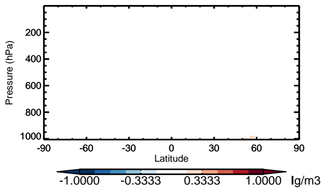
v11-01 - v10-01 SO 2 - Zonal mean abs diff for Jan
