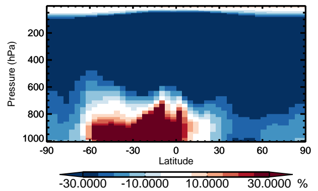
v11-01 / v10-01 ASOA3 - Zonal mean % diff for Jan
