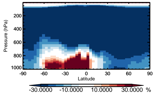
v11-01 / v10-01 ASOA2 - Zonal mean % diff for Jan
