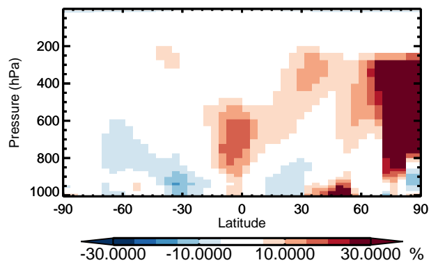
v11-01 / v10-01 HBr - Zonal mean % diff for Jan
