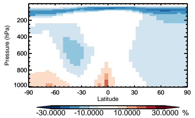
v11-01 / v10-01 MAP - Zonal mean % diff for Jan
