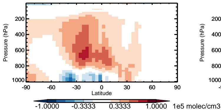
v11-01 - v10-01 OH - Zonal mean abs diff for Jan
