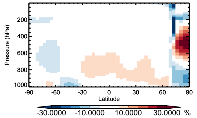
v11-01 / v10-01 ClOO - Zonal mean % diff for Jan
