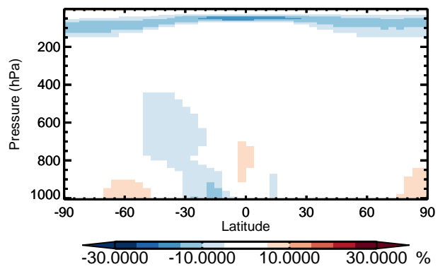
v11-01 / v10-01 PAN - Zonal mean % diff for Jan
