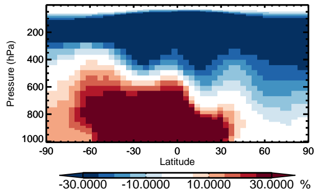
v11-01 / v10-01 NH4 - Zonal mean % diff for Jan
