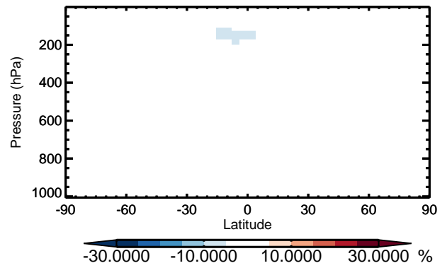
v11-01 / v10-01 H2O - Zonal mean % diff for Jan
