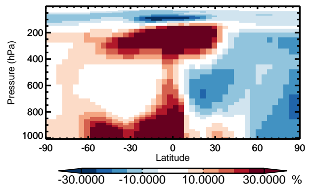
v11-01 / v10-01 TSOG0 - Zonal mean % diff for Jan
