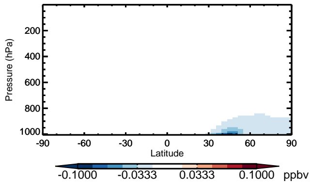
v11-01 - v10-01 XYLE - Zonal mean abs diff for Jan
