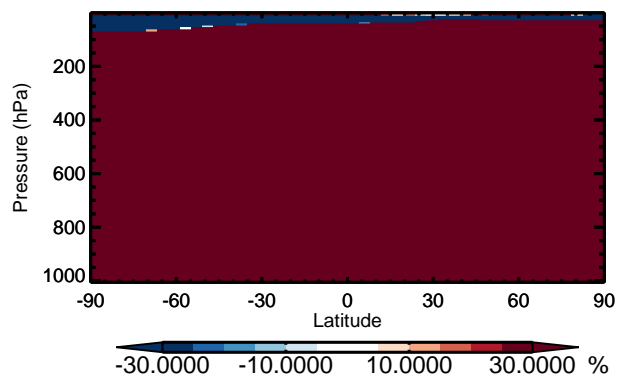
v11-01 / v10-01 NITs - Zonal mean % diff for Jan
