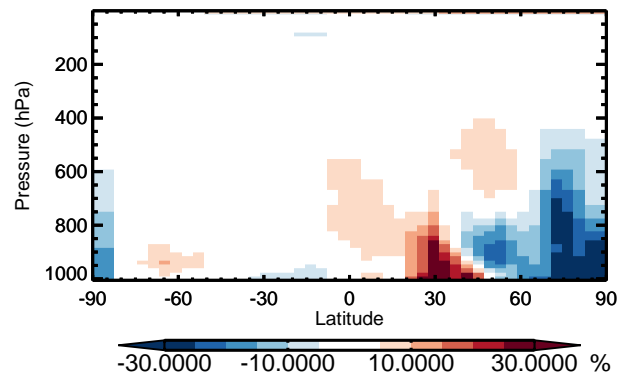
v11-01 / v10-01 MPN - Zonal mean % diff for Jan
