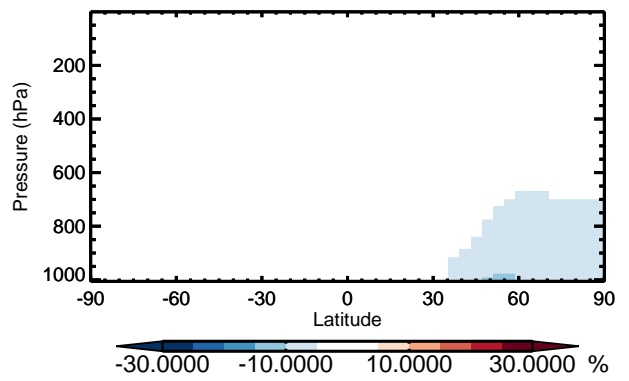
v11-01 / v10-01 O3 - Zonal mean % diff for Jan
