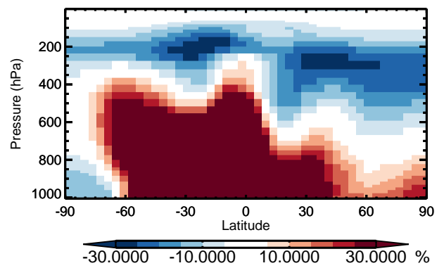
v11-01 / v10-01 SO 4 - Zonal mean % diff for Jan
