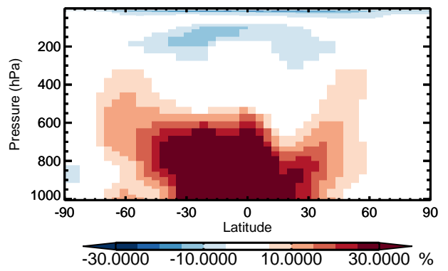
v11-01 / v10-01 HOBr - Zonal mean % diff for Jan
