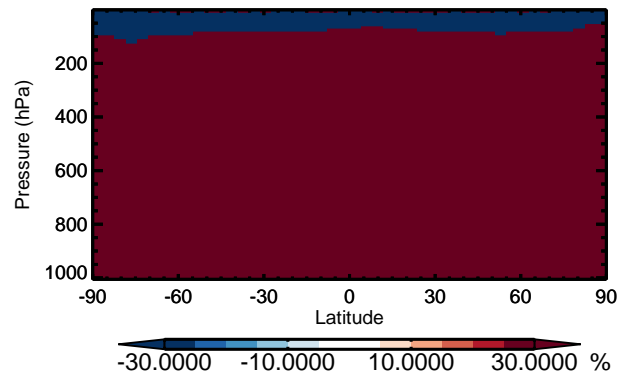
v11-01 / v10-01 SO 4 s - Zonal mean % diff for Jan
