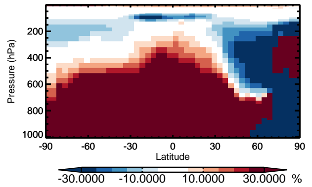
v11-01 / v10-01 Cl2O2 - Zonal mean % diff for Jan
