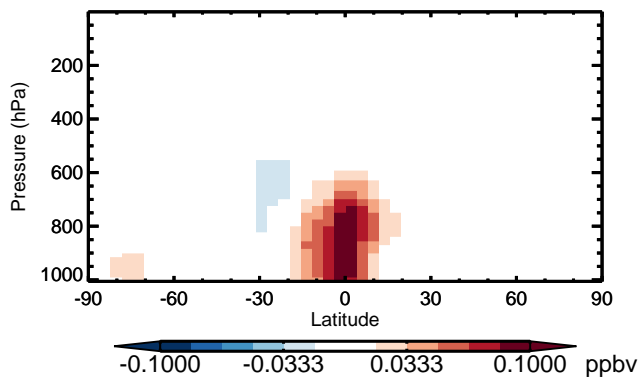
v11-01 - v10-01 H 2 O 2 - Zonal mean abs diff for Jan
