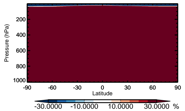
v11-01 / v10-01 HCFC141b - Zonal mean % diff for Jan
