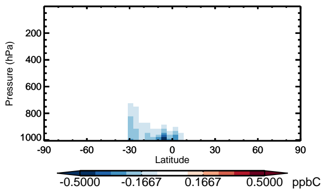
v11-01 - v10-01 ISOP - Zonal mean abs diff for Jan
