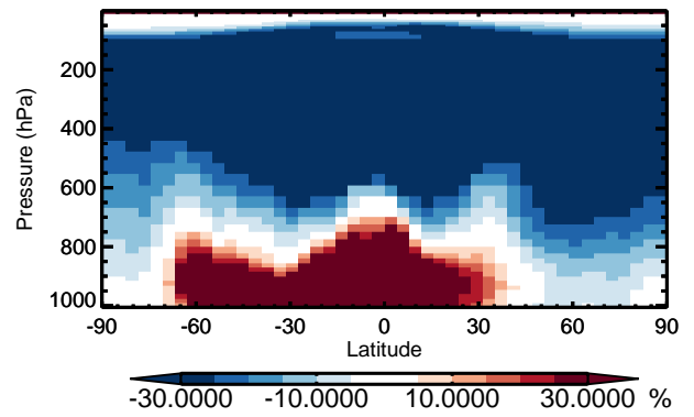
v11-01 / v10-01 ISOA3 - Zonal mean % diff for Jan
