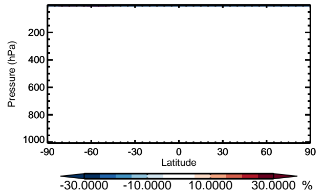
v11-01 / v10-01 CFC11 - Zonal mean % diff for Jan
