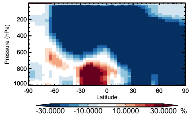
v11-01 / v10-01 OCIO - Zonal mean % diff for Jan
