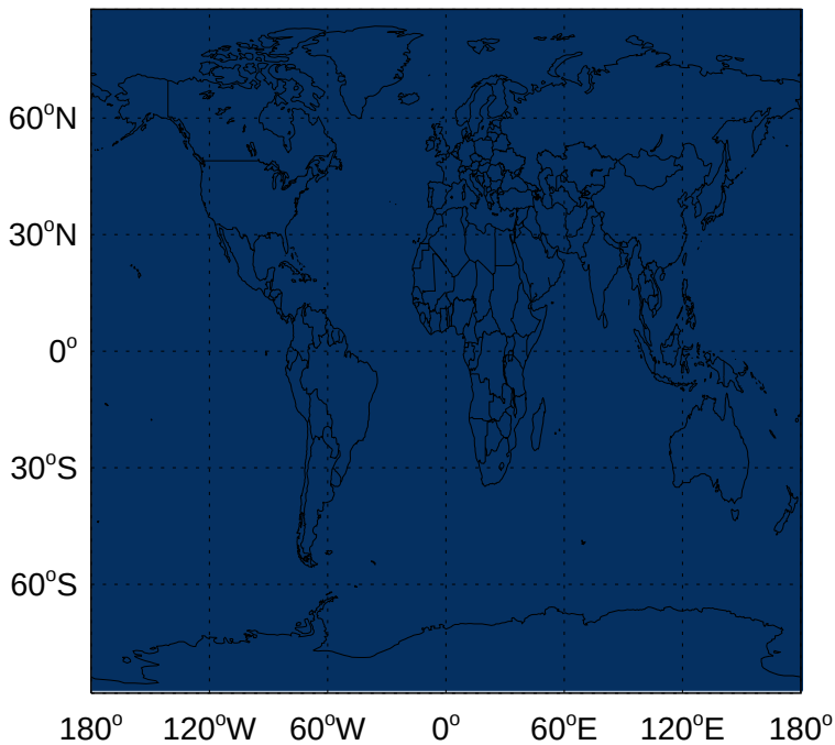
v11-01-public-Run0 - v11-01g-Run0 ACET biomass emissions for Apr
