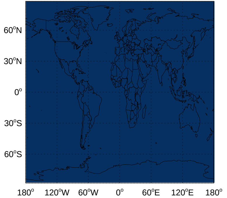
v11-01-public-Run0 - v11-01k-Run0 ACET anthro+biofuel emissions for Apr
