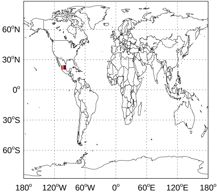
v11-01-public-Run0 - v11-01g-Run0 ACET anthro+biofuel emissions for Apr
