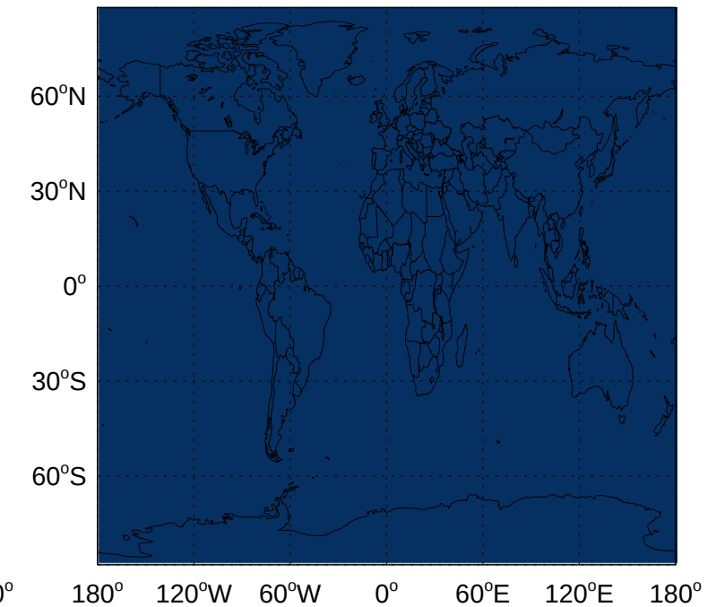
v11-01-public-Run0 - v11-01k-Run0 ACET biomass emissions for Apr
