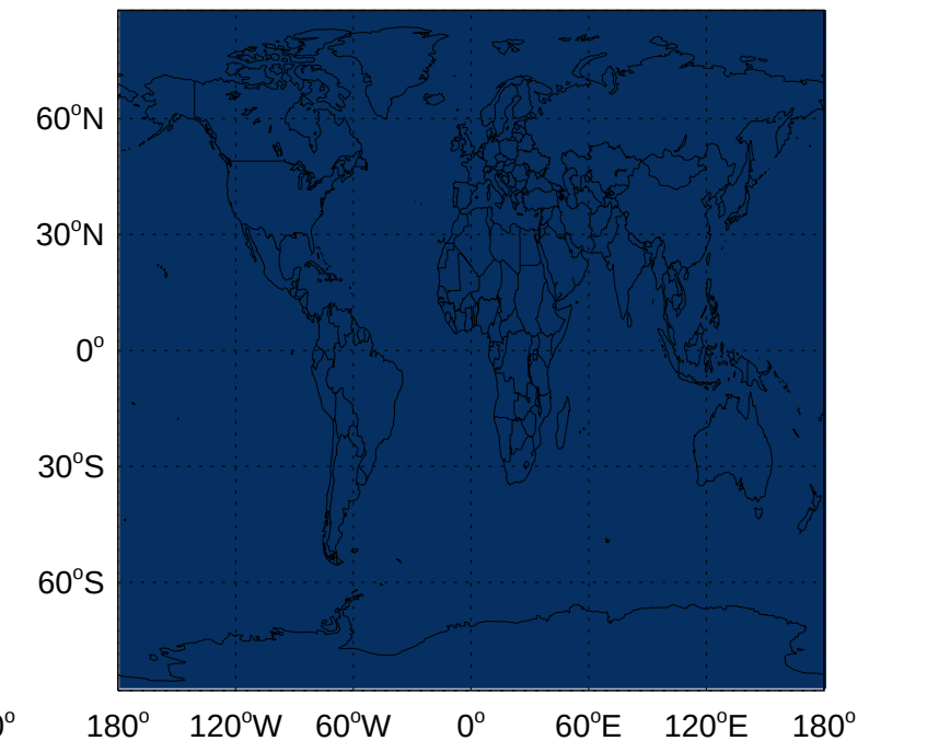
v11-01-public-Run0 - v11-01k-Run0 ACET ocean source emissions for Jul
