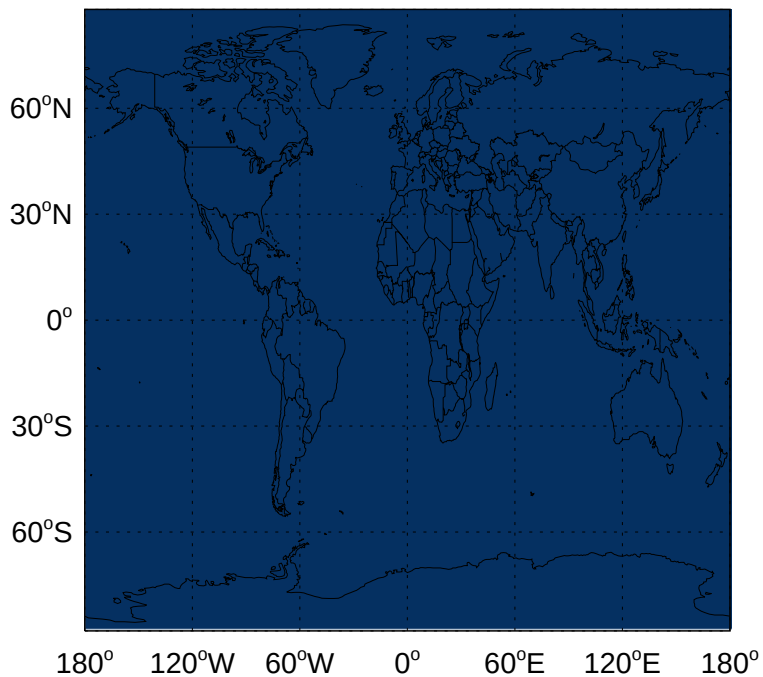
v11-01-public-Run0 - v11-01g-Run0 ACET ocean source emissions for Jul
