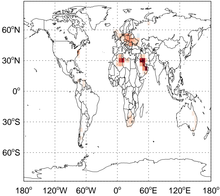
v11-01-public-Run0 - v11-01g-Run0 C3H8 anthro+biofuel emissions for Jul
