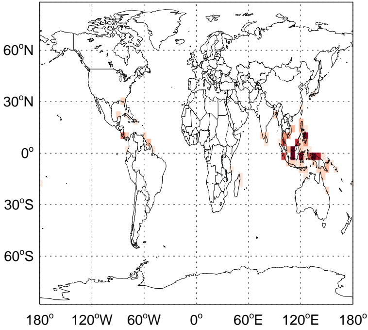
v11-01-public-Run0 - v11-01g-Run0 CO from MONOT emissions for Apr
