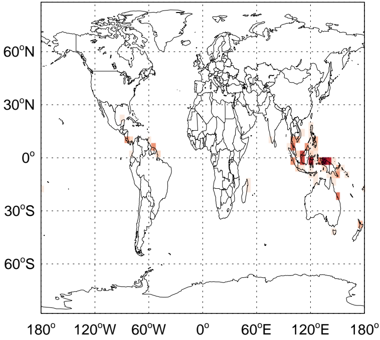
v11-01-public-Run0 - v11-01g-Run0 CO from MONOT emissions for Jan
