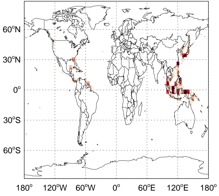
v11-01-public-Run0 - v11-01g-Run0 CO from MONOT emissions for Jul
