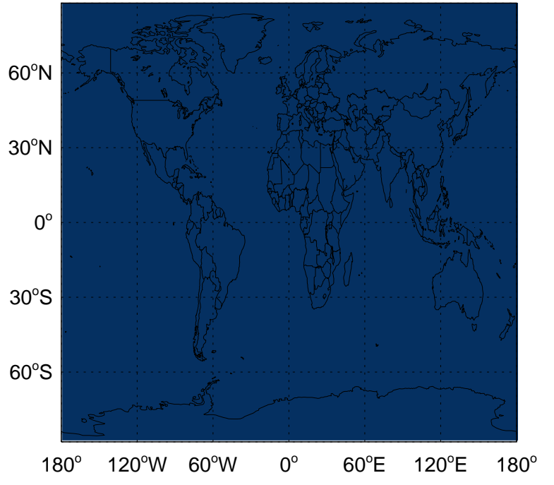
v11-01-public-Run0 - v11-01k-Run0 CO from MONOT emissions for Jul
