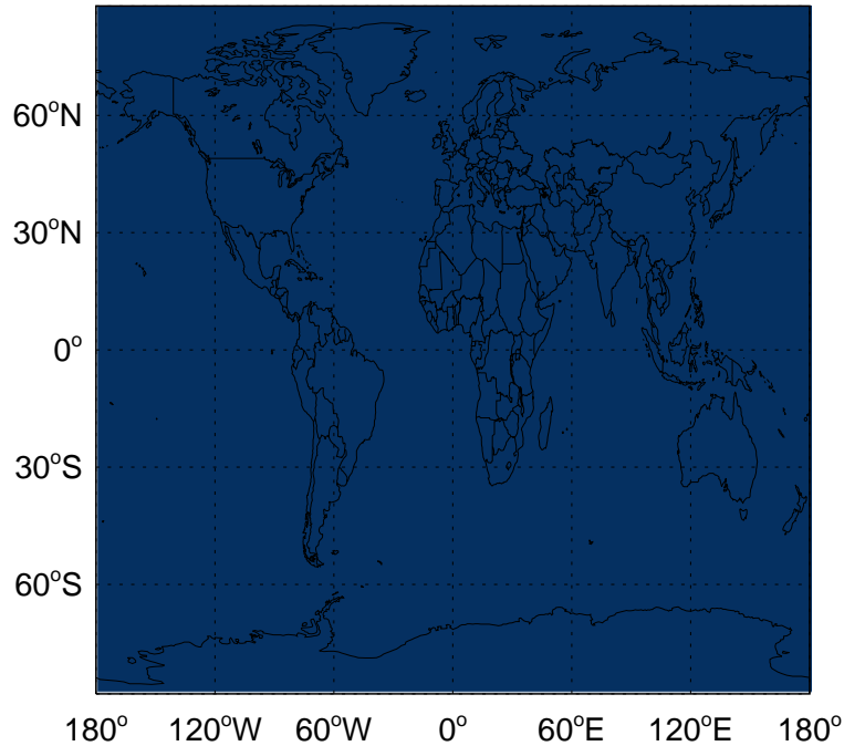
v11-01-public-Run0 - v11-01k-Run0 MEK biomass emissions for Apr
