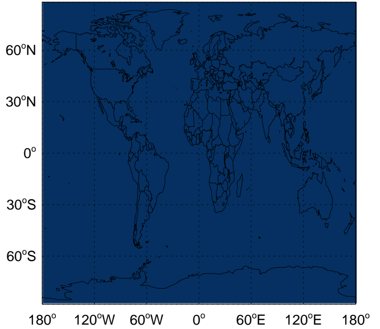
v11-01-public-Run0 - v11-01k-Run0 MEK anthro+biofuel emissions for Apr
