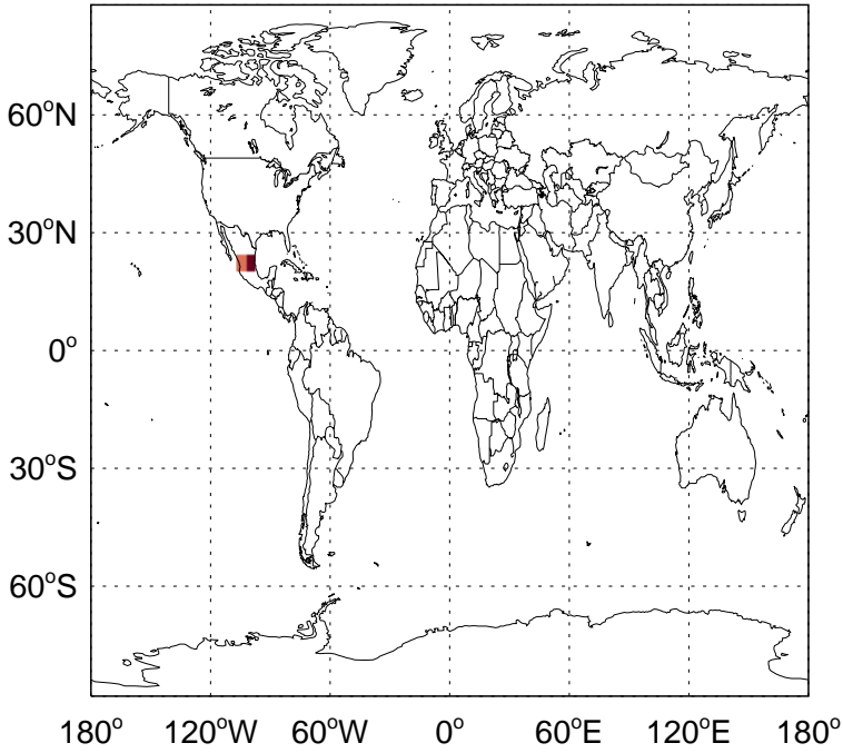
v11-01-public-Run0 - v11-01g-Run0 MEK anthro+biofuel emissions for Jul
