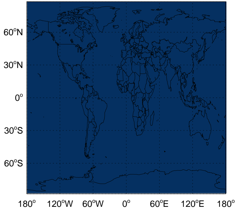
NH3 biofuel emissions for Apr
