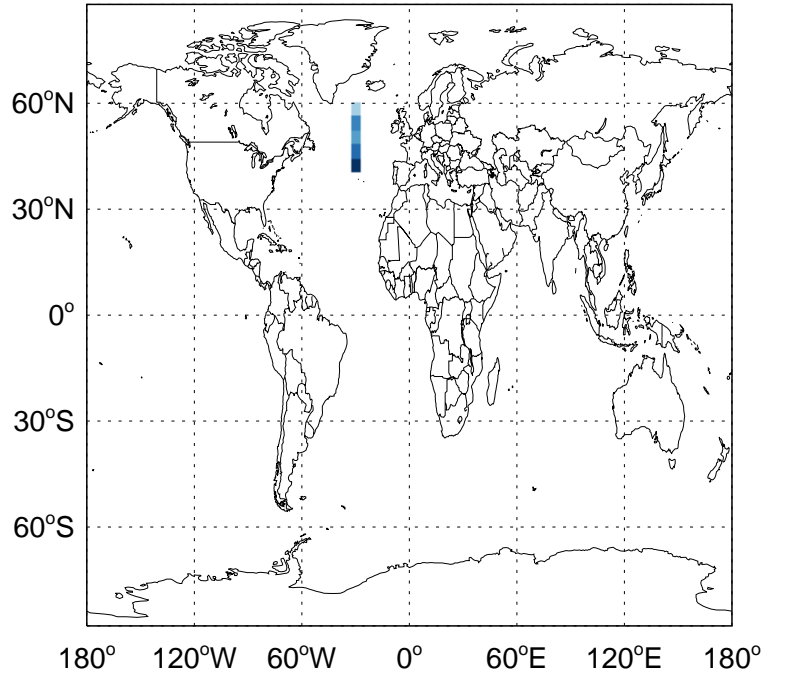
NH3 anthro emissions for Apr
