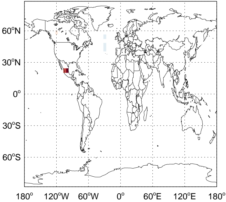
NH3 anthro emissions for Apr
